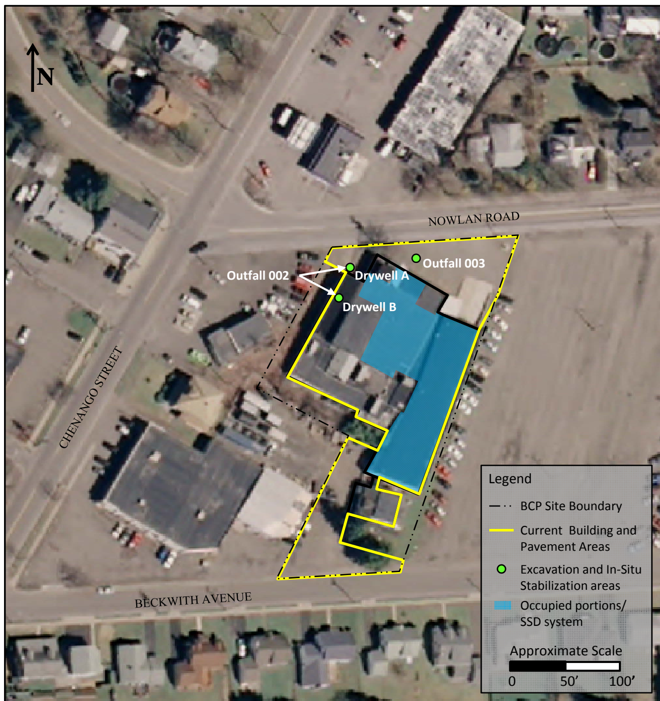
SITE FEATURES AND REMEDIAL ELEMENTS TCMF Hillcrest Facility BCP Site Number: C704045 Town of Fenton, Broome County
