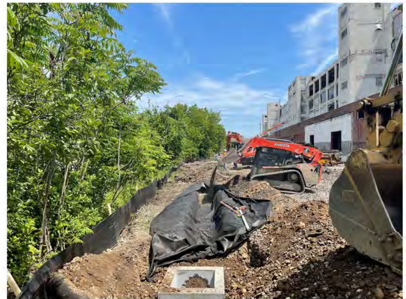
2022-06-06 14:02 42.1161278 N , 75.9527806 W Installation of storm sewer line along Avenue C, looking east
