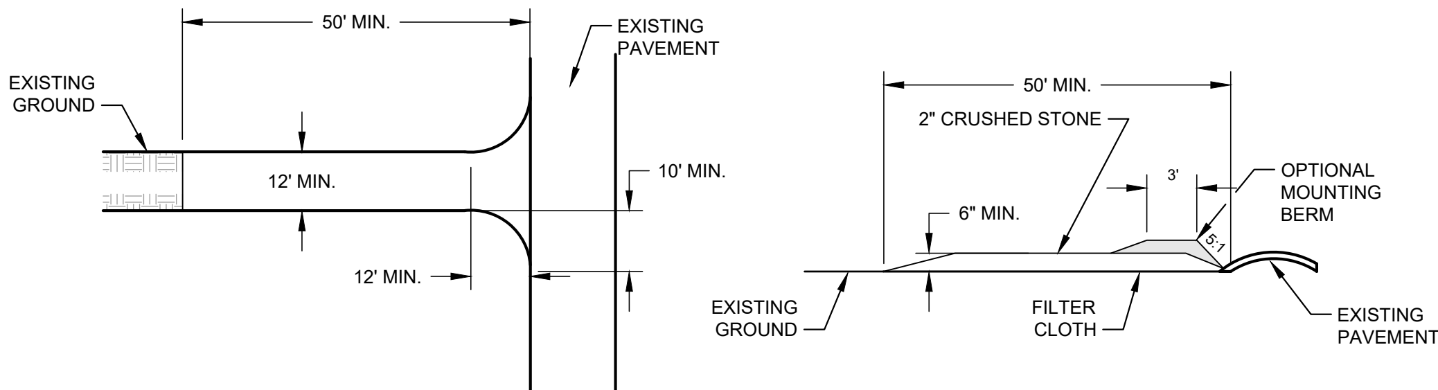
2 CONSTRUCTION ENTRANCE SCALE: NTS
