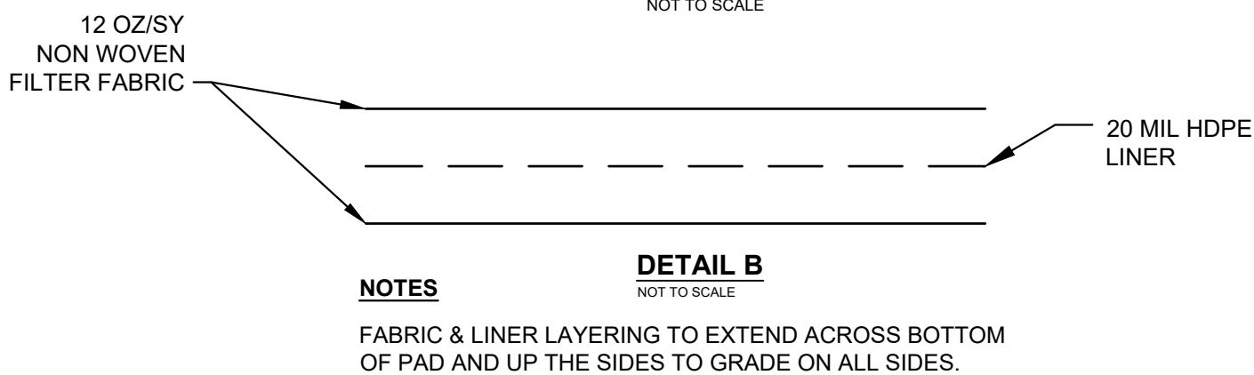
5 TRUCK WASH / DECON PAD SCALE: NTS
