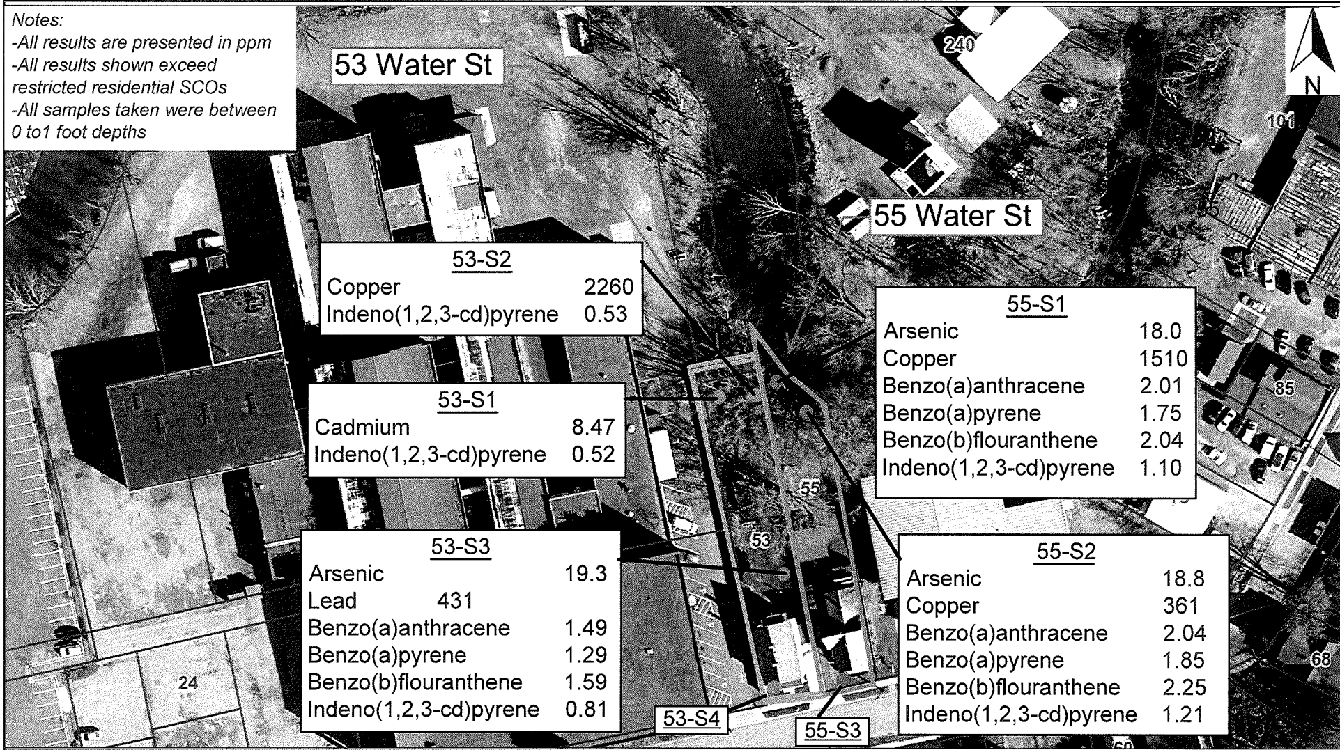
FIGURE 3: SAMPLE LOCATIONS AND EXCEEDANCES
