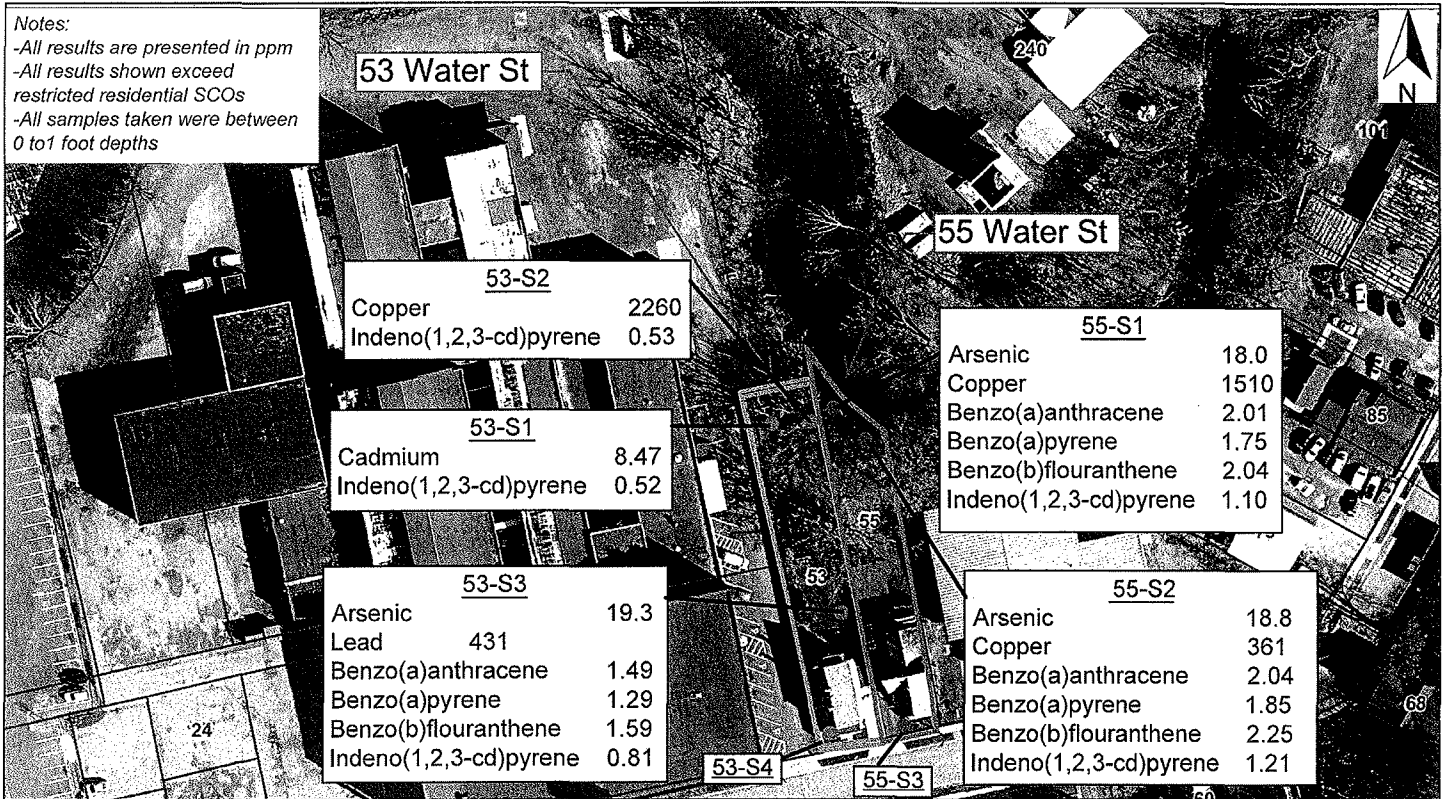
FIGURE 3: SAMPLE LOCATIONS AND EXCEEDANCES
