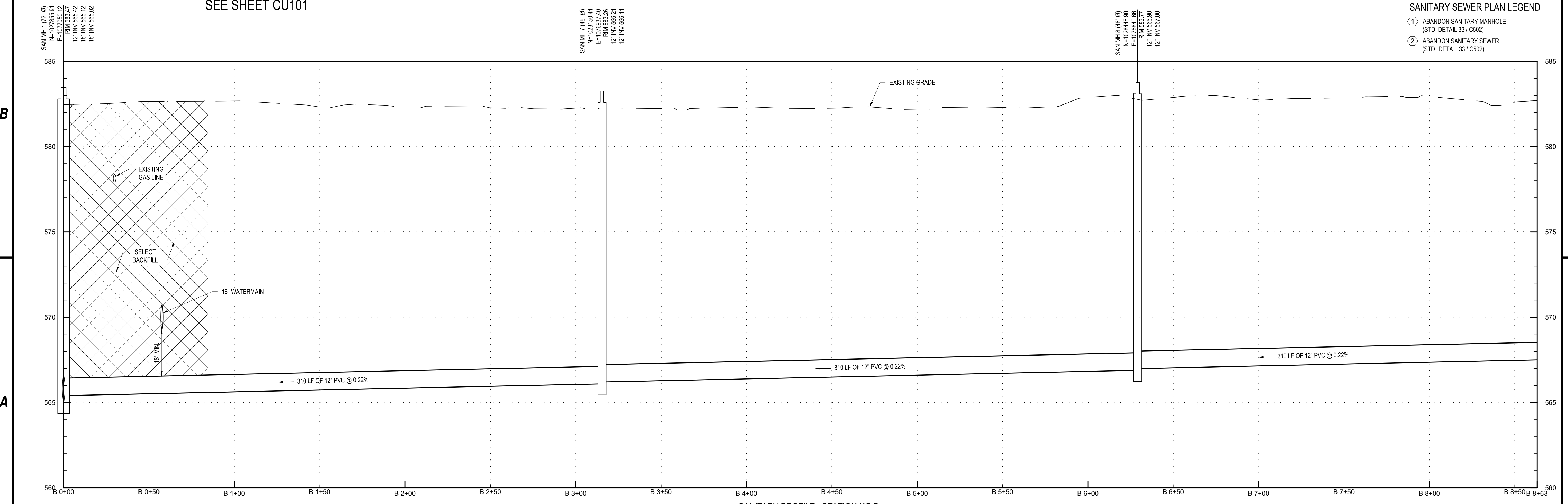
SANITARY PROFILE - STATIONING B HORZ: 1" = 30' VERT: 1" = 3'
