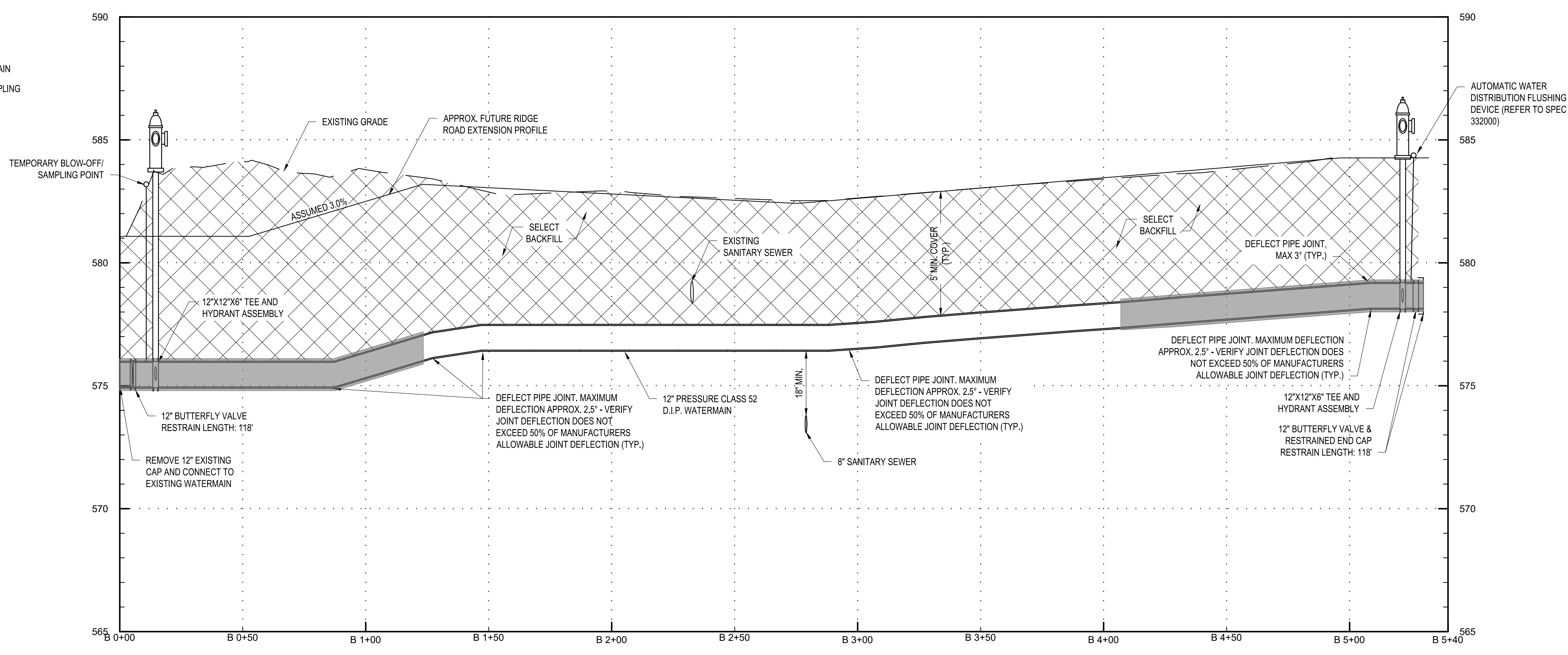
WATER PROFILE - STATIONING B HORZ: 1" = 30' VERT: 1" = 3'
