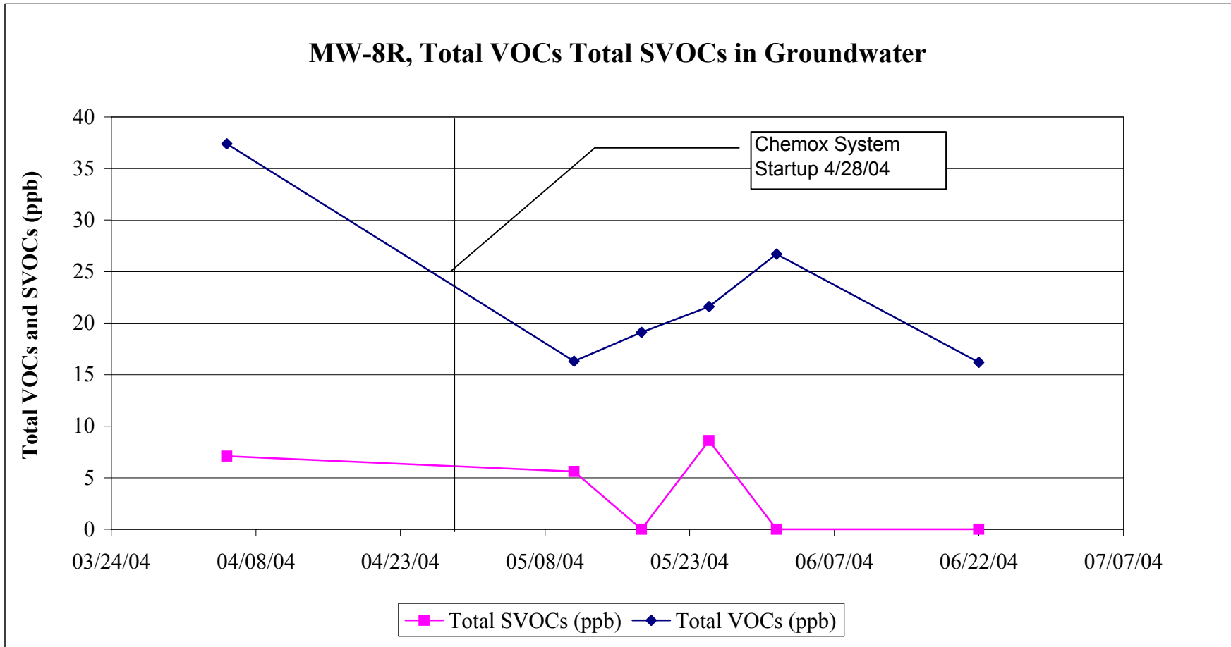
Figure 15. Summary of Total Volatile Organic Compounds (VOCs) and Semivolatile Organic Compounds (SVOCs) for MW-8R, Buffalo Terminal, ExxonMobil Oil Corporation, Buffalo, New York
