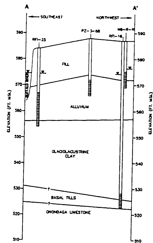
CROSS-SECTION A-A'
