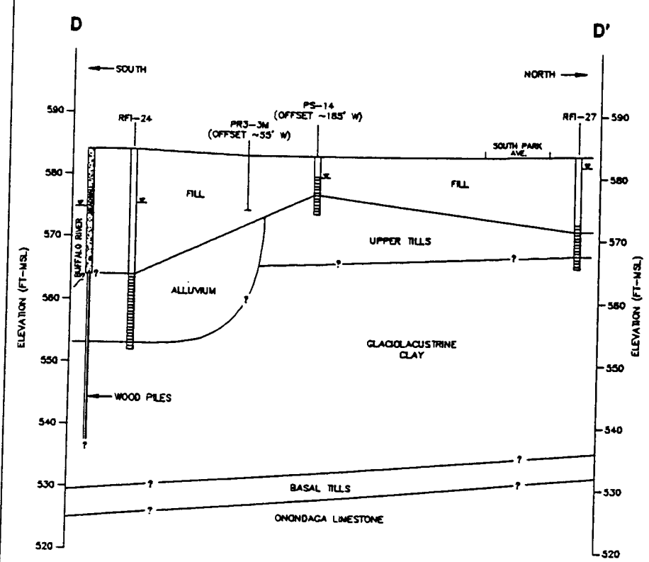
CROSS-SECTION D-D'
