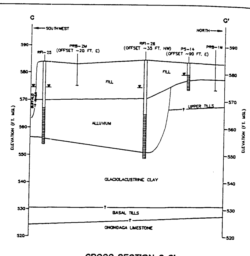
CROSS-SECTION C-C'
