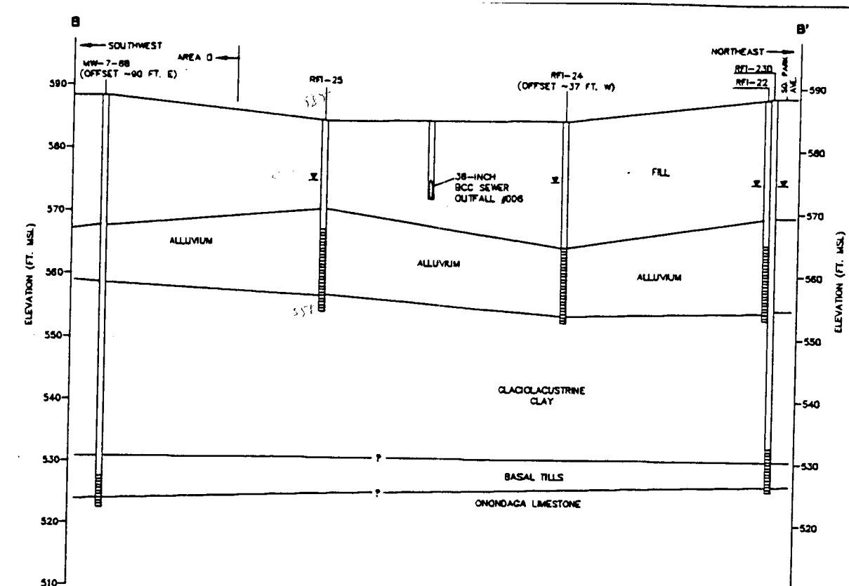
CROSS-SECTION B-B'
