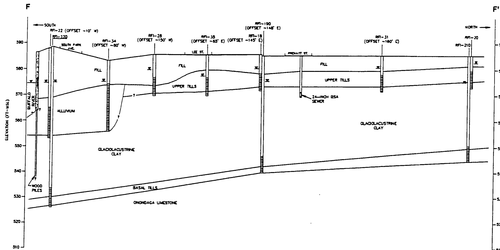
CROSS-SECTION F-F'
