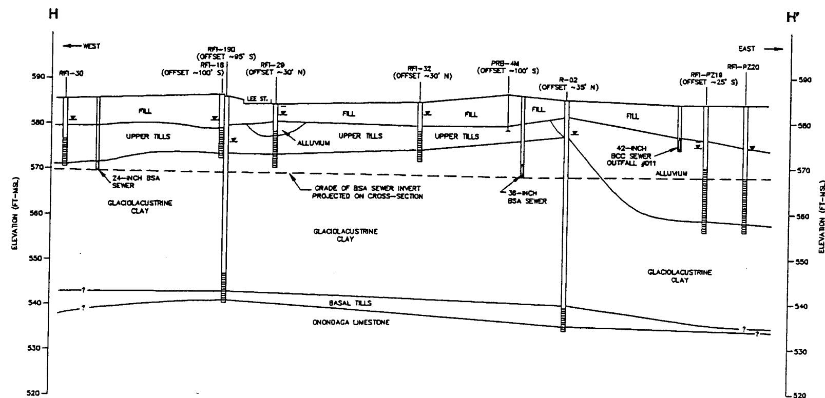
CROSS-SECTION H-H'
