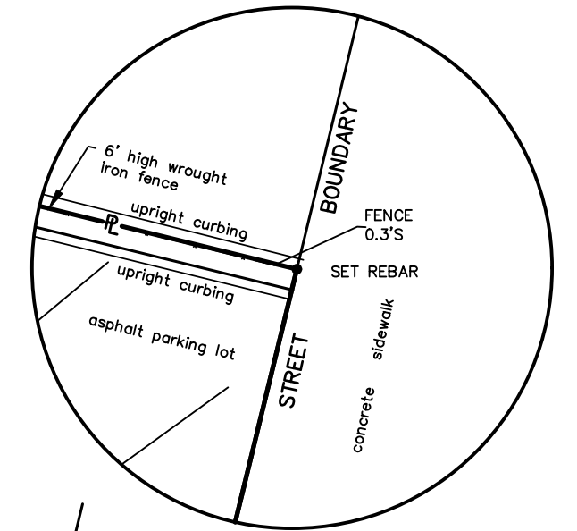
PROPERTY CORNER DETAIL
