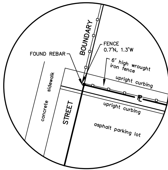
PROPERTY CORNER DETAIL
