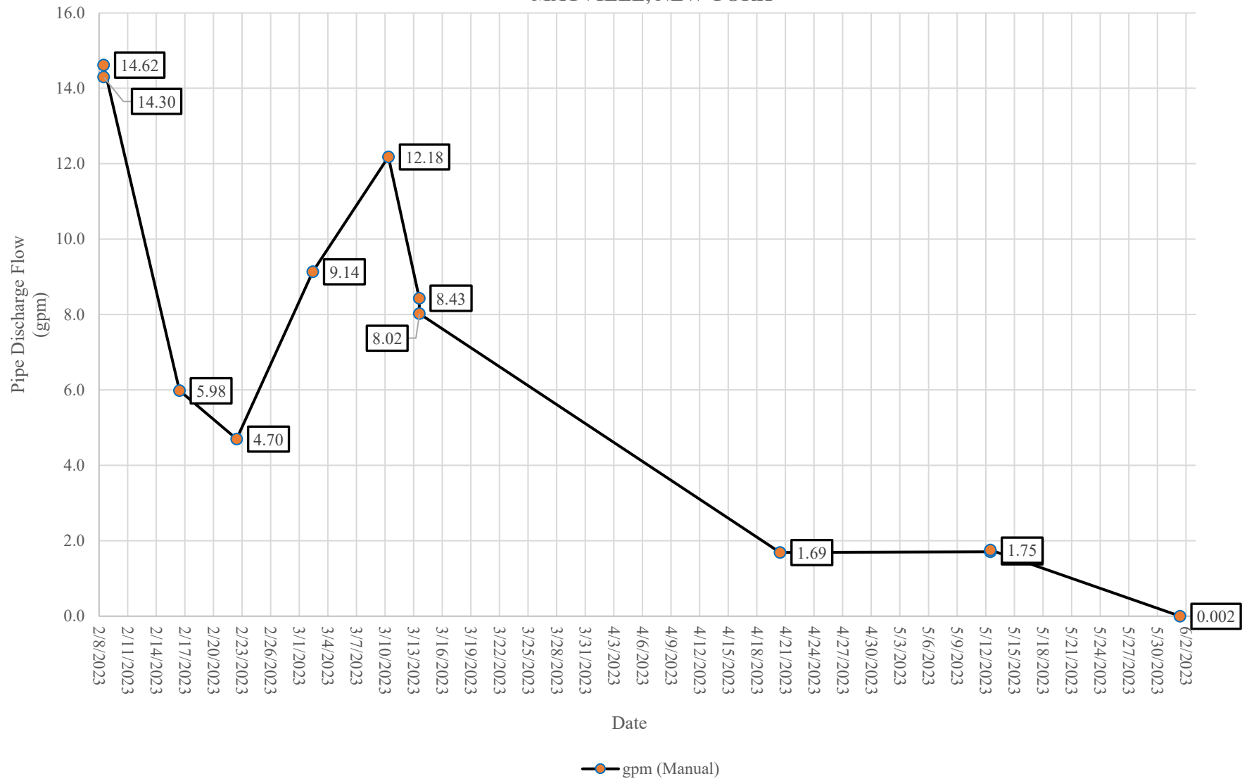
FIGURE 5 FIELD DRAINAGE DISCHARGE PIPE - FLOW MONITORING MANUAL FLOW RATE MEASUREMENTS 2023-02-08 to 2023-06-01 NYSDEC - MAYVILLE, SPILL #2008000 MAYVILLE, NEW YORK
