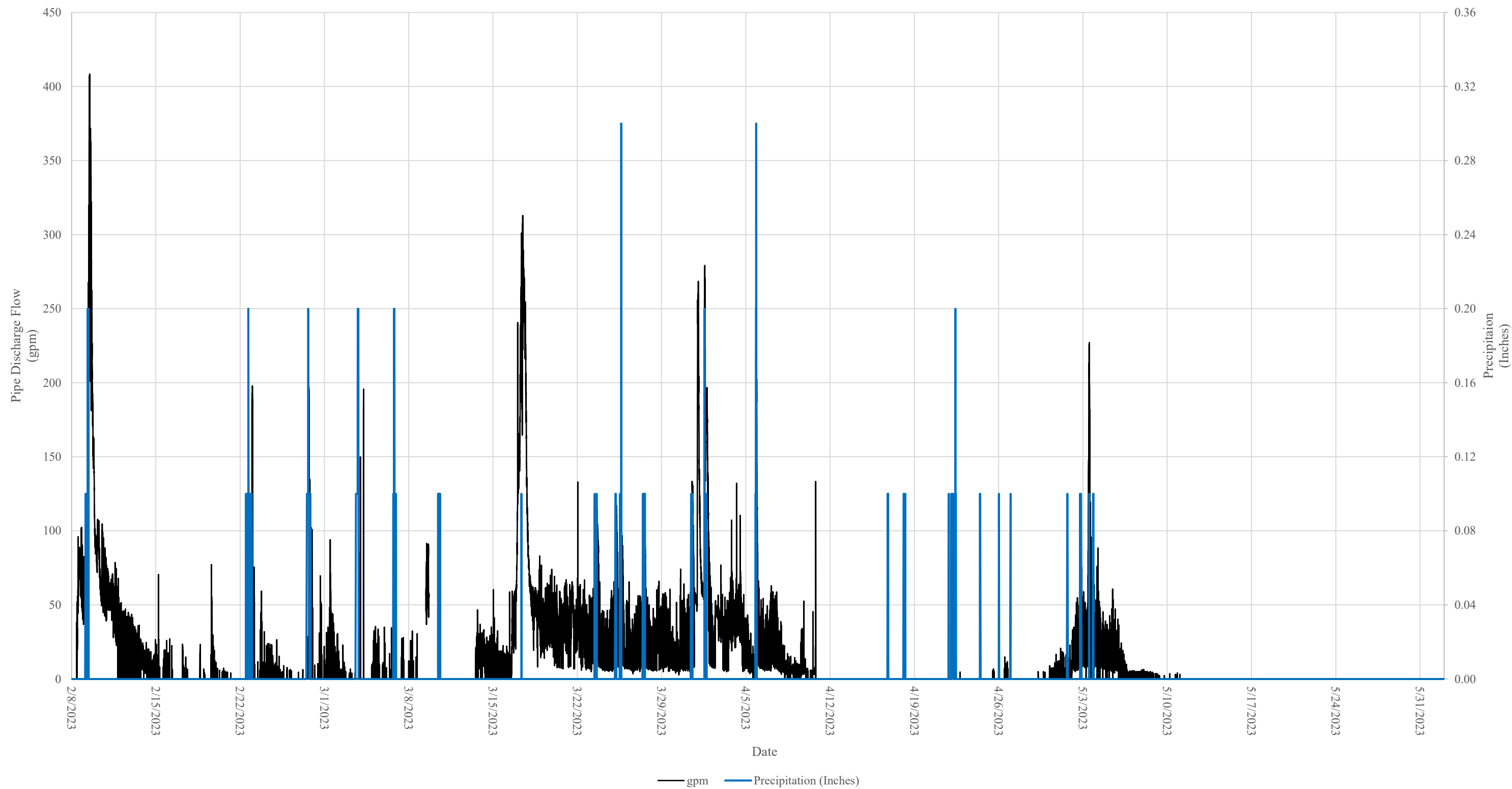
FIGURE 4 FIELD DRAINAGE DISCHARGE PIPE - FLOW MONITORING RECORDED FLOW VOLUMES (gpm) AND PRECIPITATION 2023-02-08 to 2023-06-01 NYSDEC - MAYVILLE, SPILL #2008000 MAYVILLE, NEW YORK
