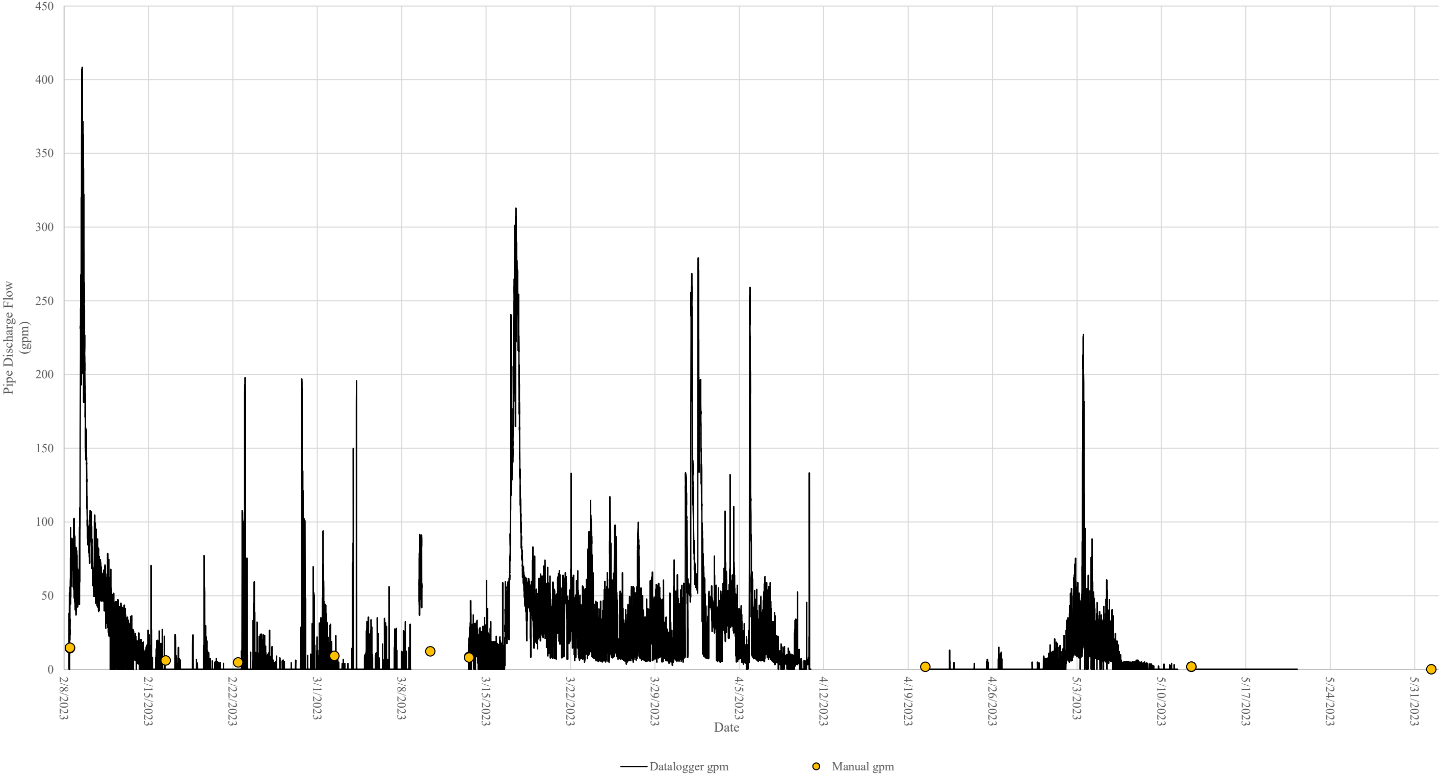
FIGURE 6 FIELD DRAINAGE DISCHARGE PIPE - FLOW MONITORING RECORDED FLOW VOLUMES (gpm) - DATALOGGER AND MANUAL 2023-02-08 to 2023-06-01 NYSDEC - MAYVILLE, SPILL #2008000 MAYVILLE, NEW YORK
