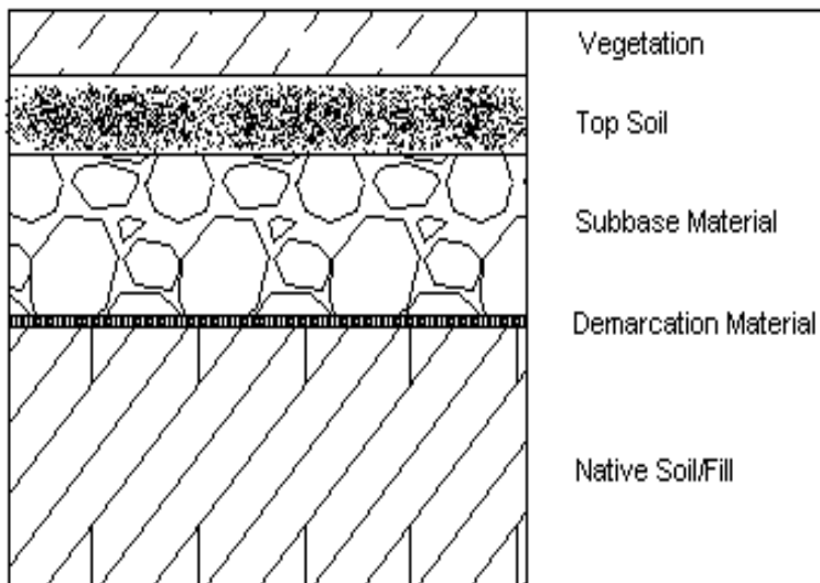
Detail 1: Cover System Cross Section
