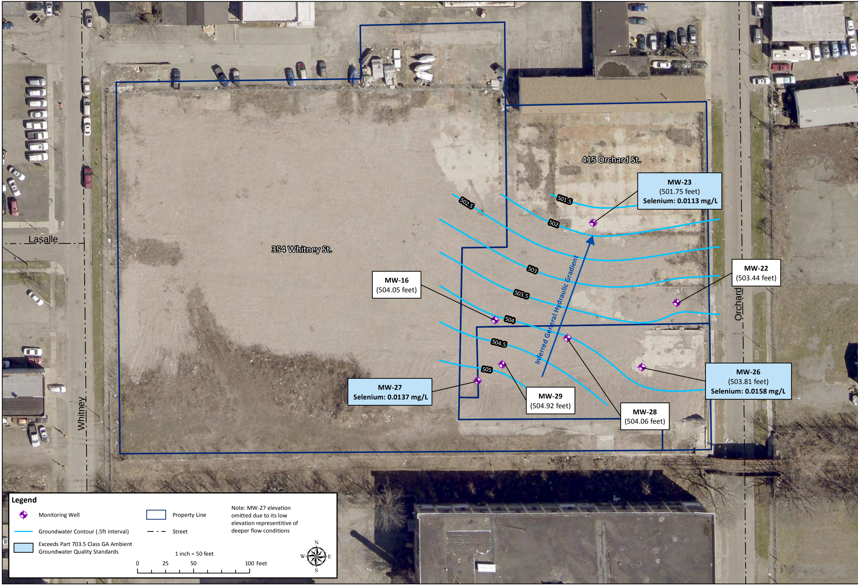
FIGURE 6. GROUNDWATER CONTOUR & SAMPLE RESULTS MAY 2018 ORCHARD WHITNEY PERIODIC REVIEW REPORT ERP SITE #E828123 ROCHESTER, NY
