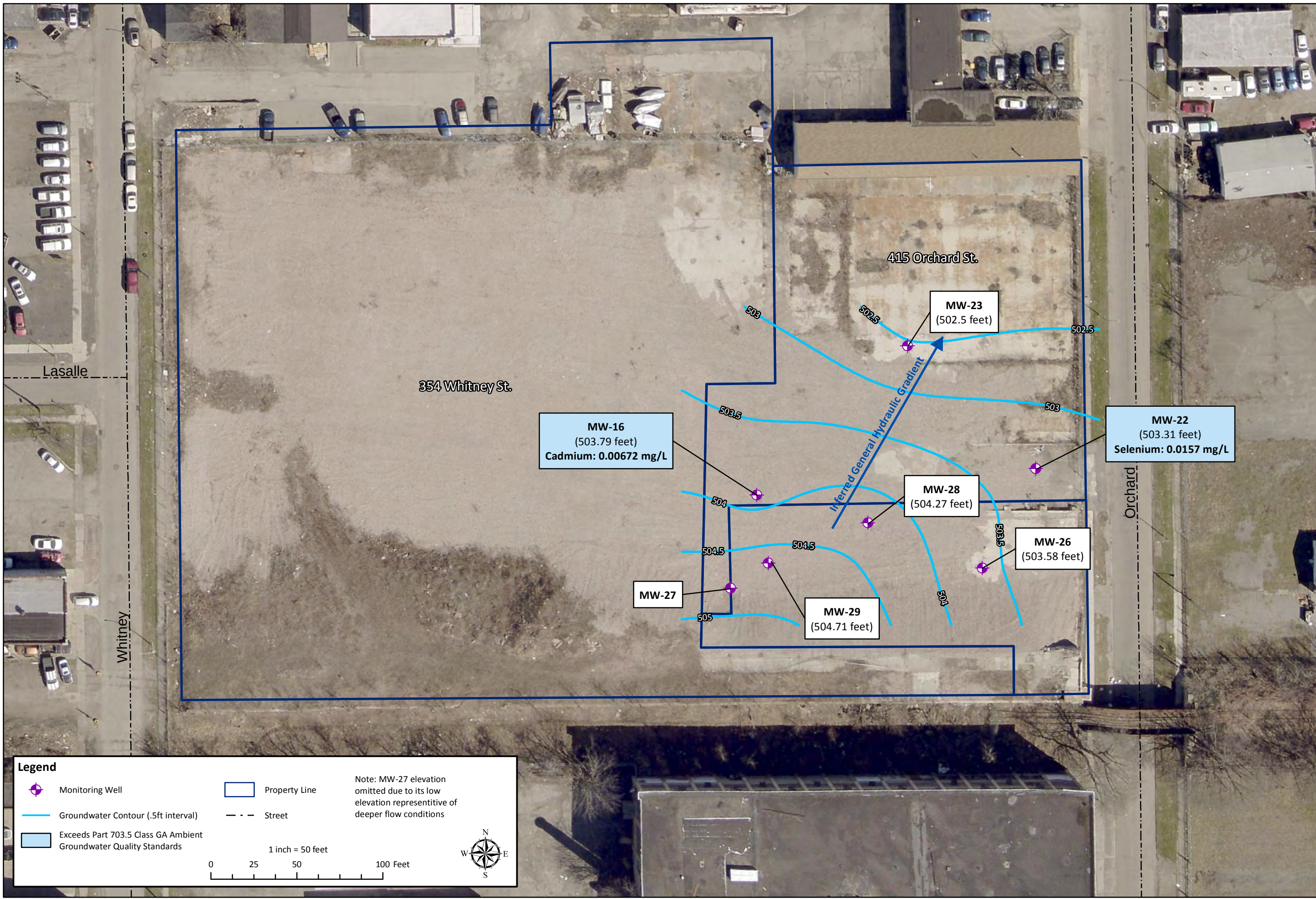
FIGURE 5. GROUNDWATER CONTOUR & SAMPLE RESULTS MARCH 2018 ORCHARD WHITNEY PERIODIC REVIEW REPORT ERP SITE #E828123 ROCHESTER, NY
