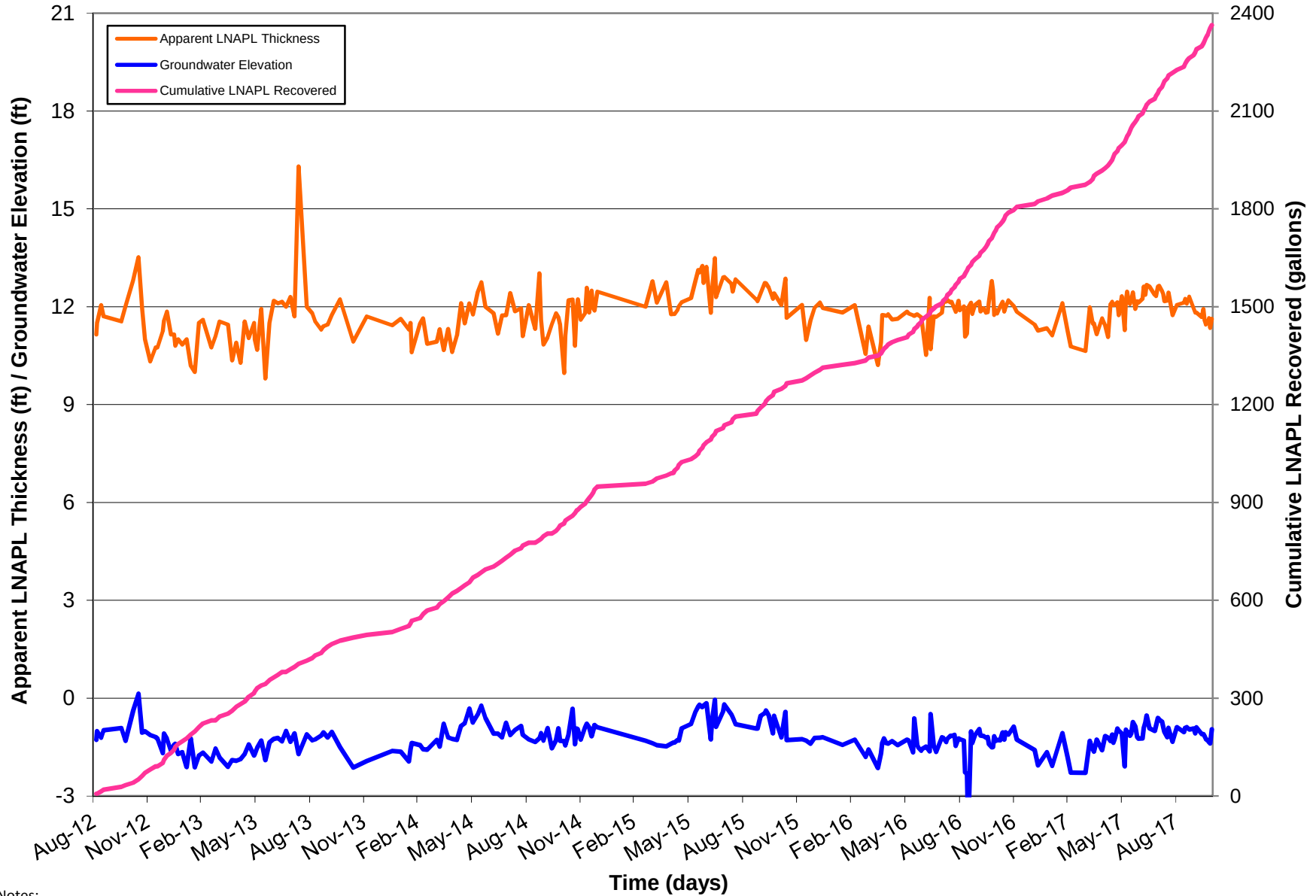
FIGURE 3 Monitoring Well Hydrograph for MW-48D Former Pratt Oil Works, Long Island City, New York
