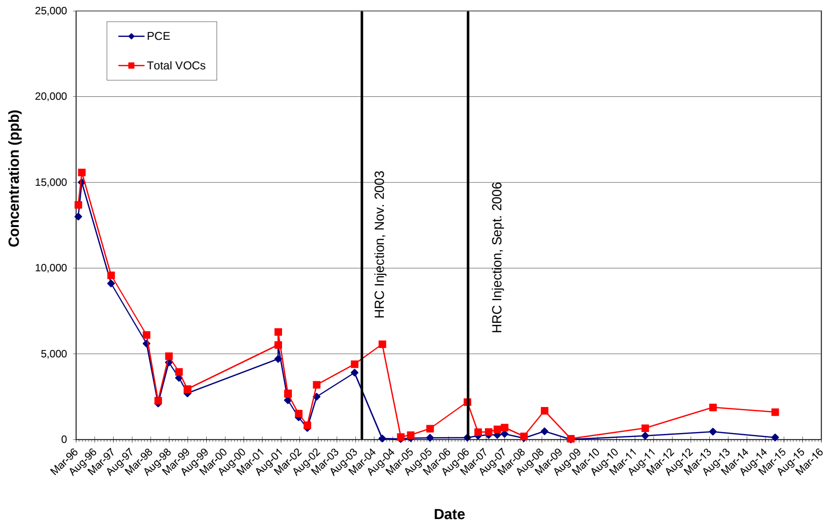
FIGURE 5 Well MW-2 Total VOC & PCE Concentrations
