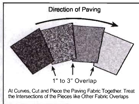
Figure 8 PETROMAT PLACEMENT AROUND CURVES
