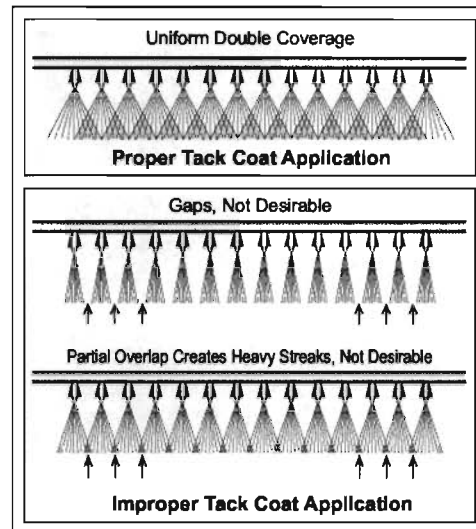
Figure 1 DISTRIBUTOR TRUCK SPRAYS
