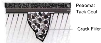
Figure 4 CRACK FILLING
