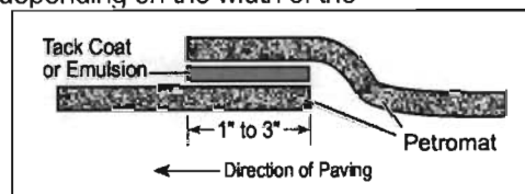
Figure 7 JOINTS AND OVERLAPS
