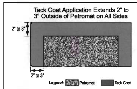
Figure 6 TACK COAT APPLICATION
