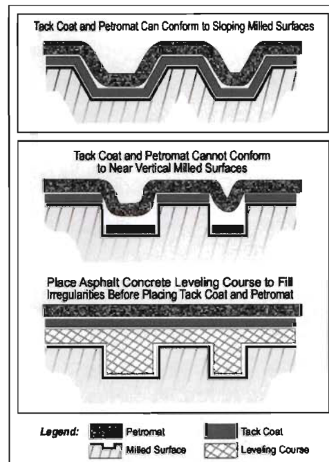
Figure 3 PREPARATION OF MILLED OR VERTICAL SURFACES
