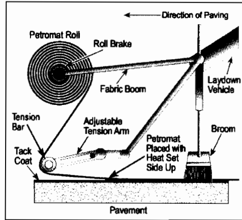
Figure 2 COMPONENTS OF LAYDOWN EQUIPMENT
