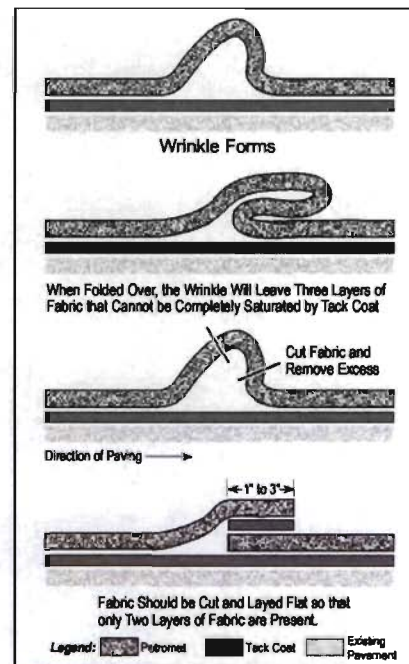
Figure 9 WRINKLE REPAIR
