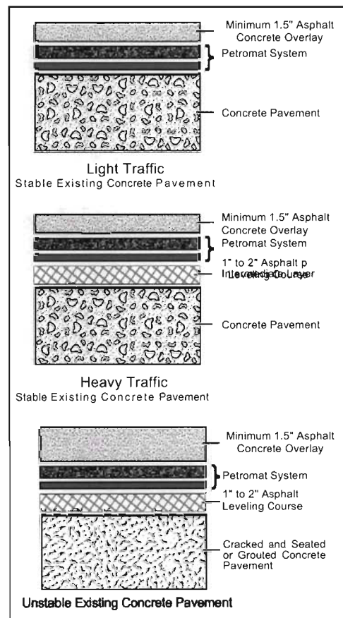
Figure 5 PORTLAND CEMENT CONCRETE PAVEMENT TREATMENTS
