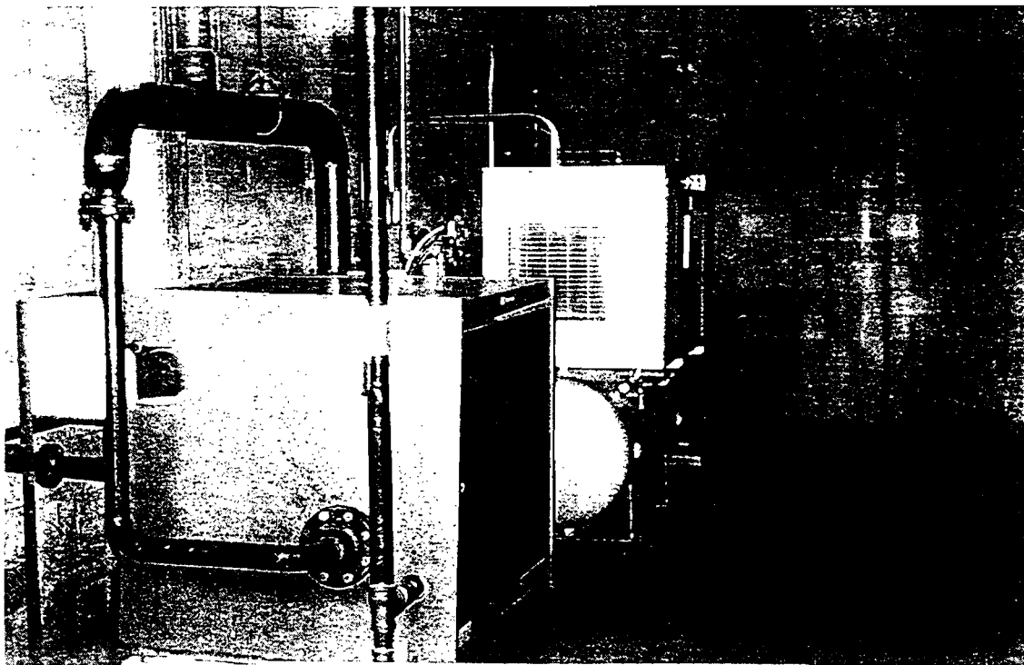
Gas fired furnace
