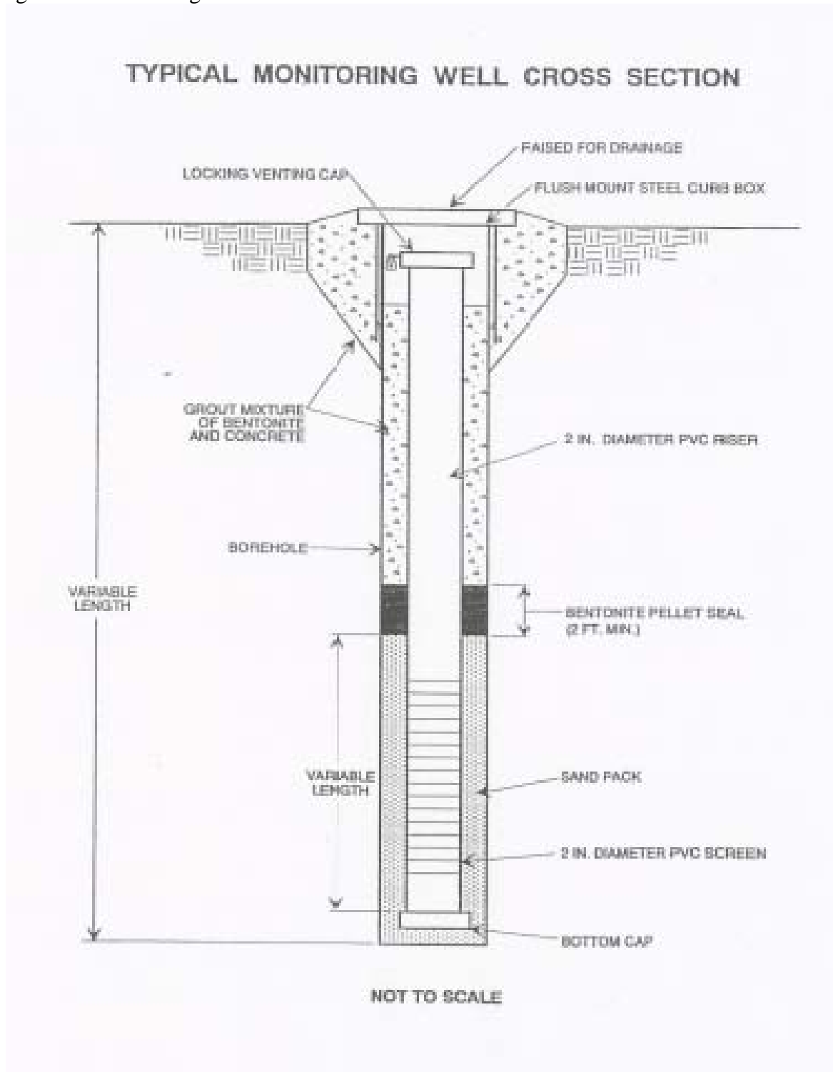
Figure 4.2 Monitoring Well Cross Section
