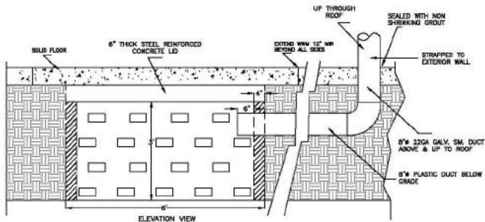
ELEVATION VIEW
