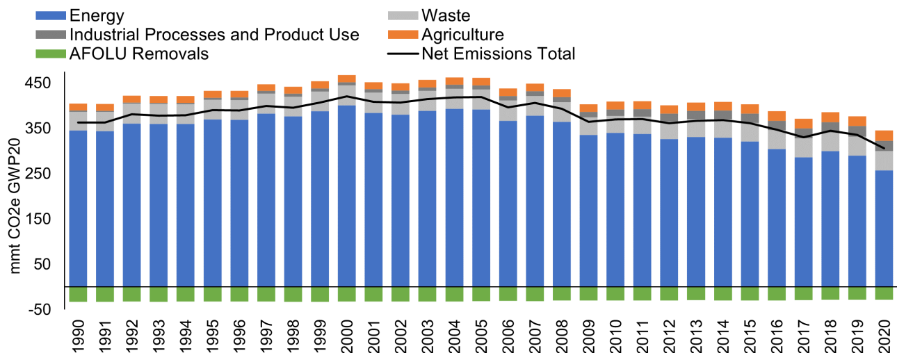
Figure ES.2: NYS Statewide Greenhouse Gas Emissions by Sector, 1990-2020 (mmt CO 2 e GWP20)
