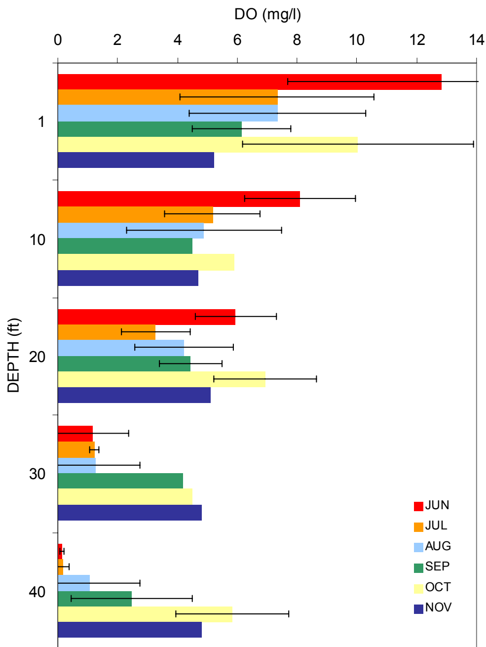
Figure 5c. Average monthly DO (mg/l) v. depth (ft) at South Norton station, 2001
