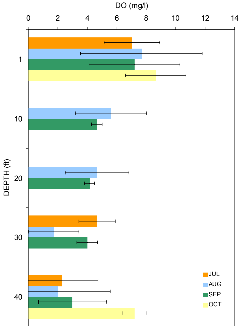
Figure 5b. Average monthly DO (mg/l) v. depth (ft) at South Norton station, 2000
