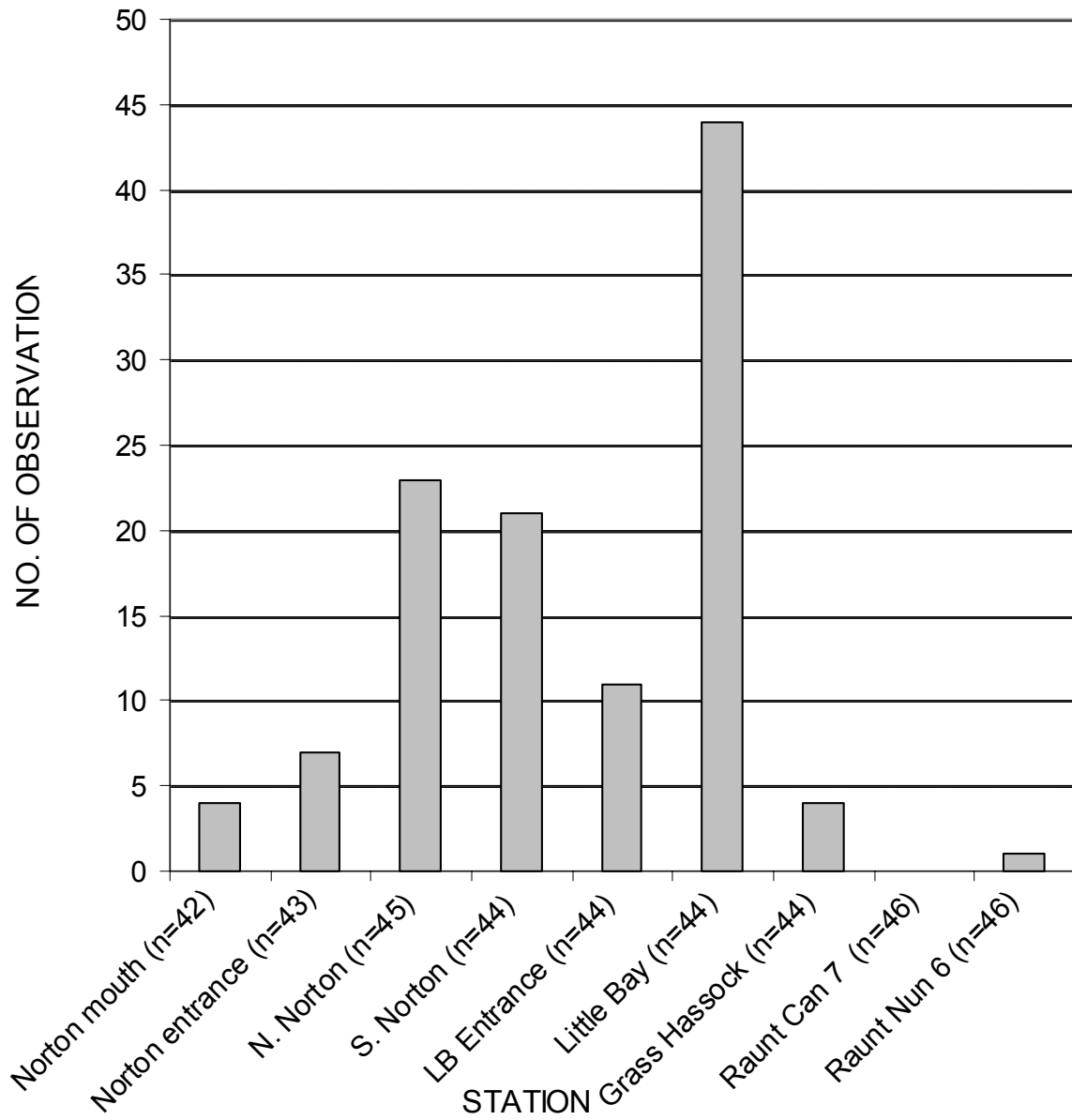
Figure 3b. Number of observations with DO readings < 3 mg/l. n=total number of observations at the station
