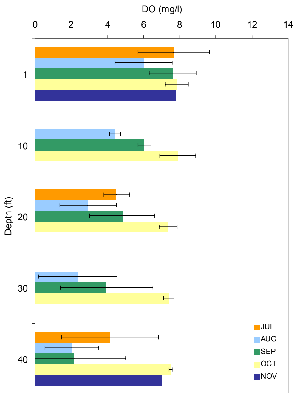
Figure 5d. Average monthly DO (mg/l) v. depth (ft) at South Norton station, 2002
