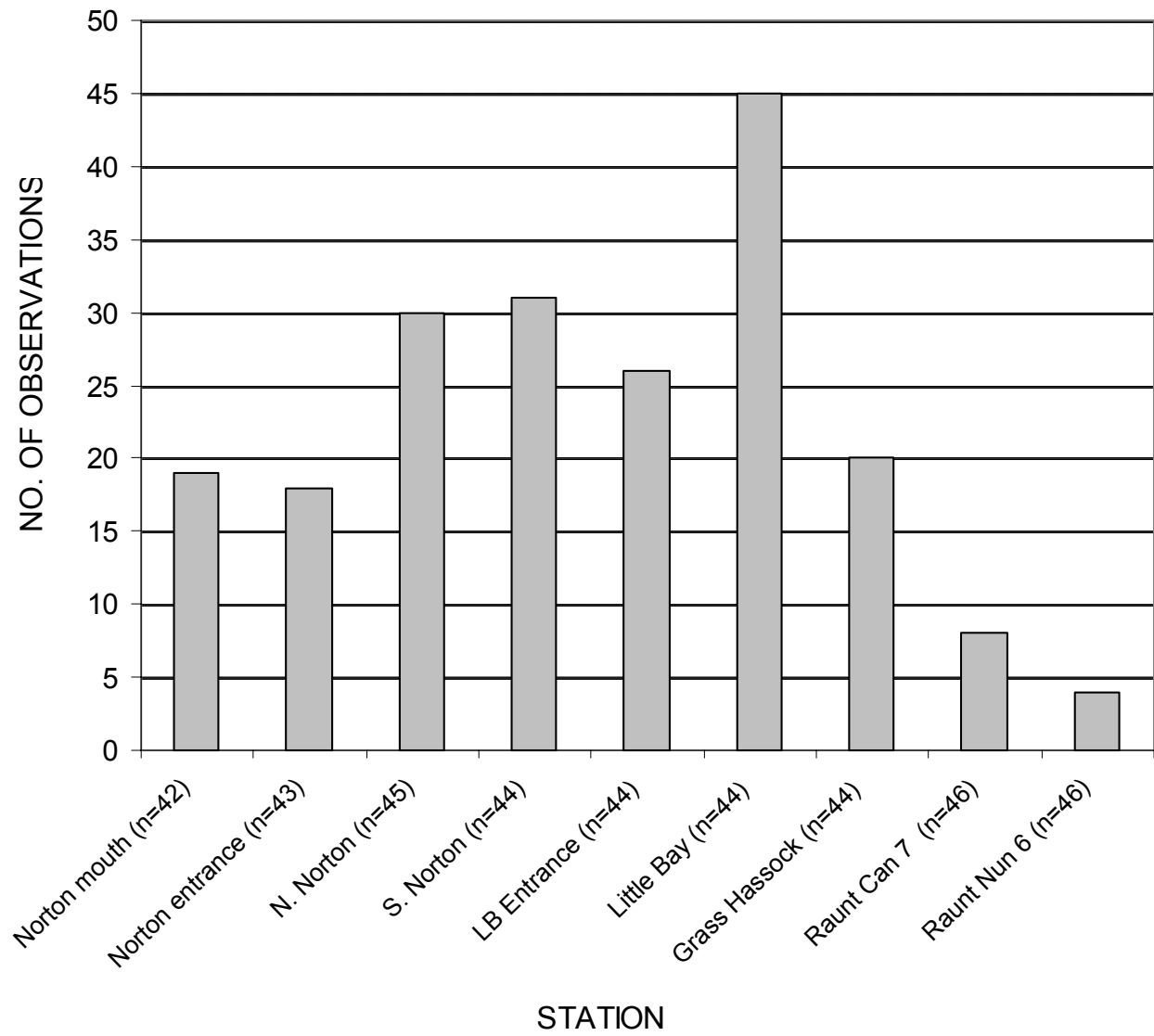
Figure 3a. Number of observations with DO readings <5 mg/l. n= total number of observations at the station
