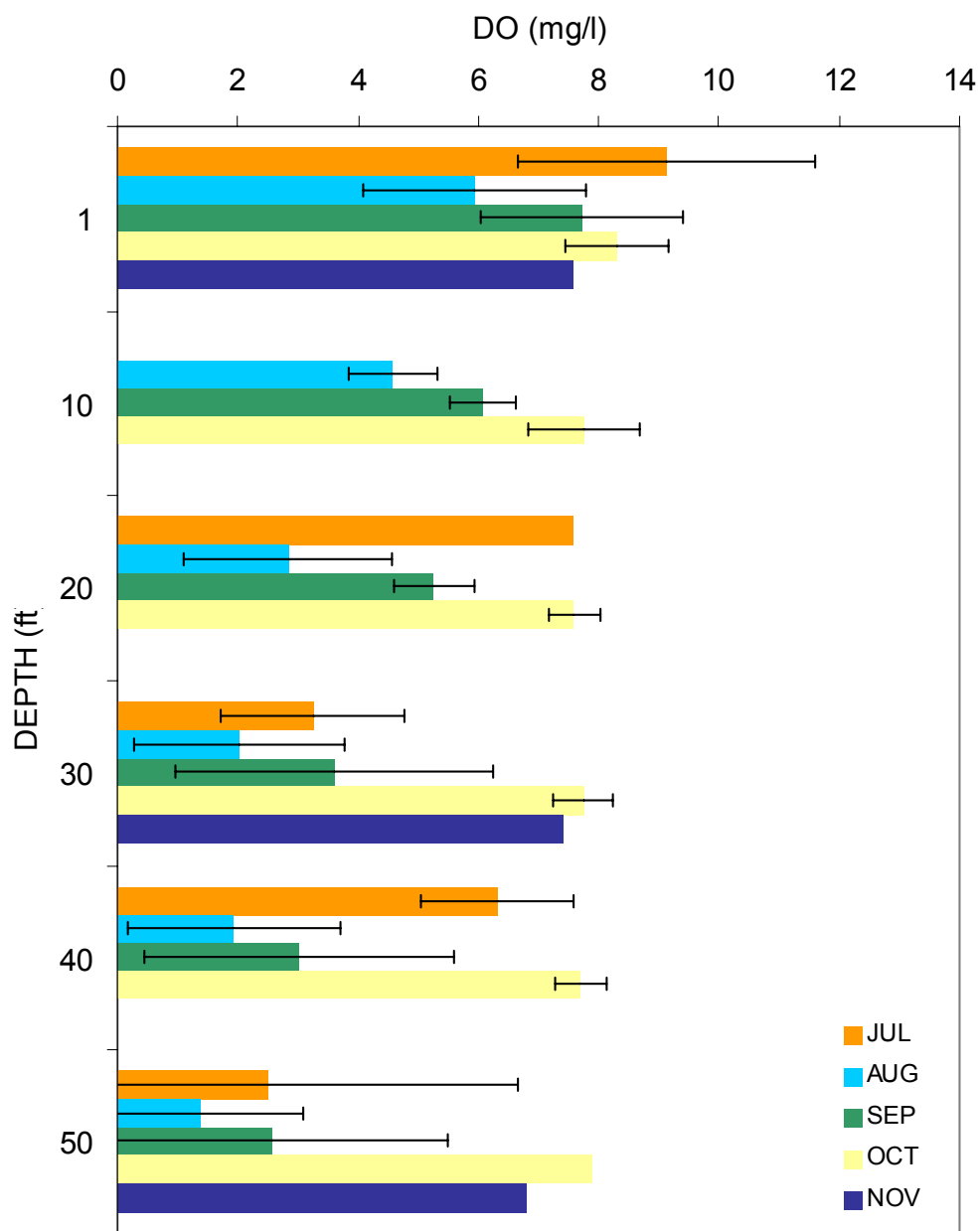
Figure 4d. Average monthly DO (mg/l) v. depth (ft) at North Norton station, 2002
