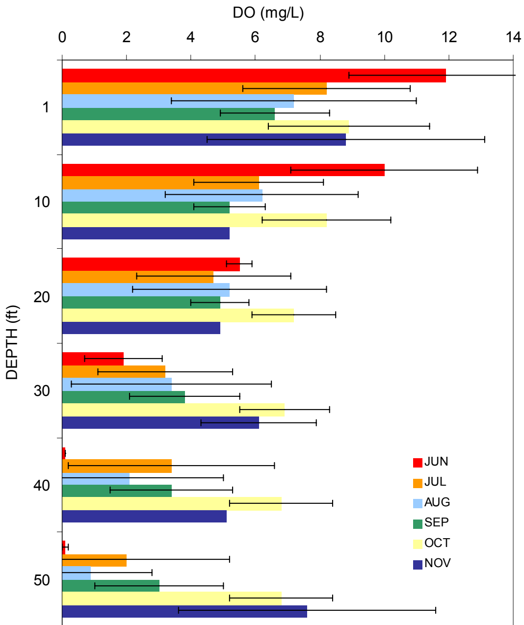
Figure 4a. Average monthly DO (mg/l) v. depth (ft) at North Norton station, 2000 through 2002
