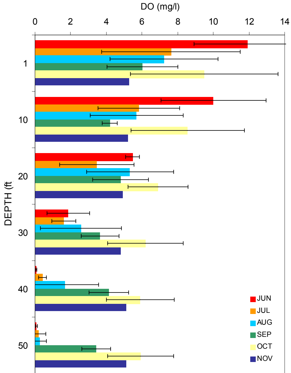
Figure 4c. Average monthly DO (mg/l) v. depth (ft) at North Norton station, 2001
