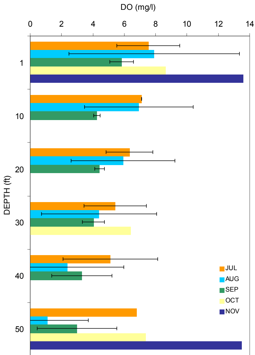
Figure 4b. Average monthly dissolved oxygen (mg/l) v. depth (ft) at North Norton station, 2000
