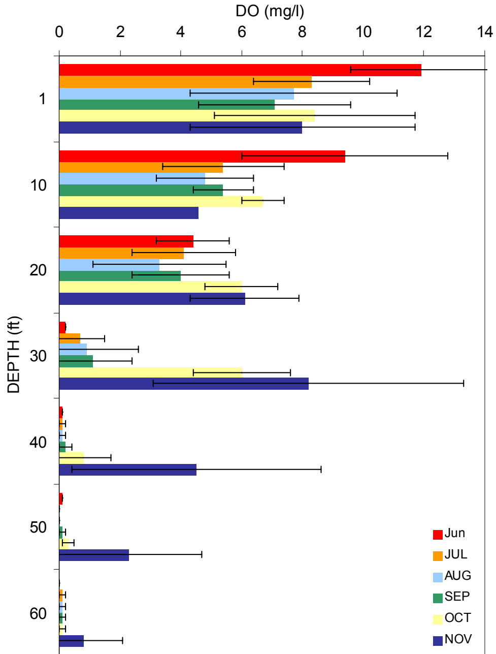
Figure 6. Average monthly DO (mg/l) v. depth (ft) at Little Bay station, 2000 through 2002
