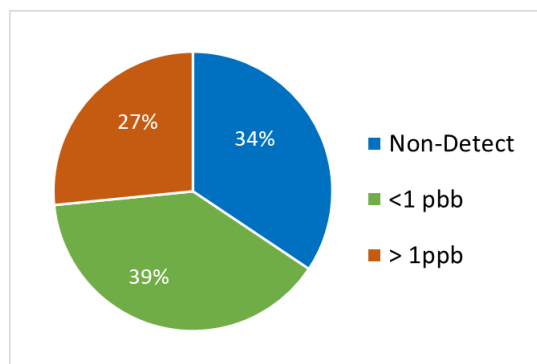
Figure 2.5: Maximum 1,4-Dioxane Concentrations in Groundwater at Sampled Inactive Landfills
