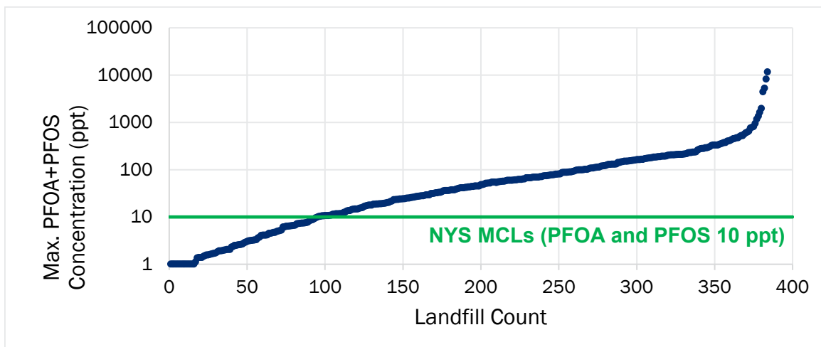
Figure 2.2: Range of Maximum PFOA + PFOS Concentrations in Groundwater at Sampled Inactive Landfills
