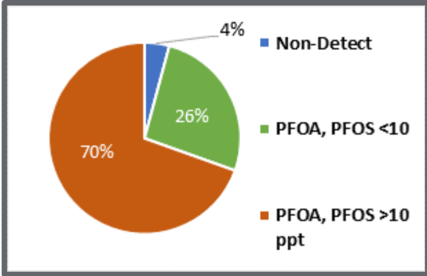
Figure ES.1: Maximum PFOA / PFOS Concentrations in Groundwater at Sampled Inactive Landfills
