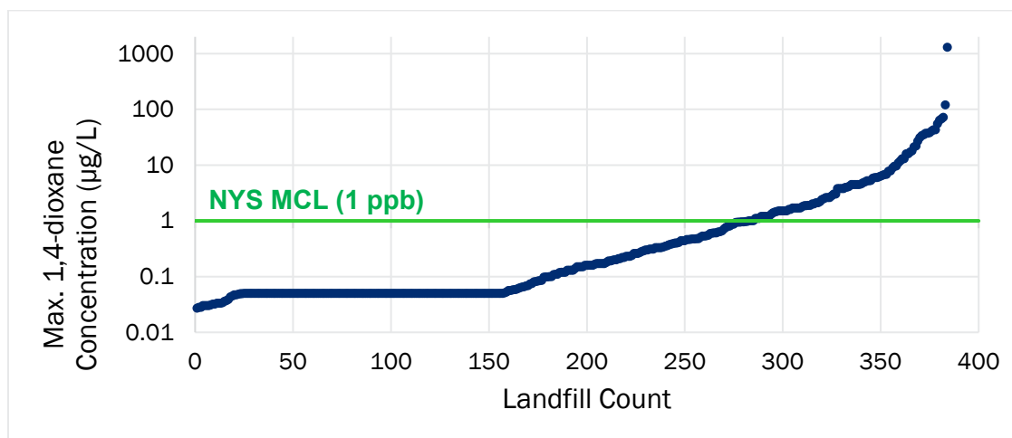
Figure 2.6: Range of Maximum 1,4-Dioxane Concentrations in Groundwater at Sampled Inactive Landfills
