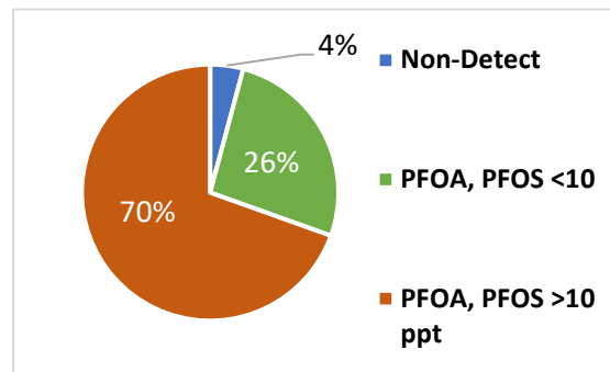
Figure 2.1: Maximum PFOA / PFOS Concentrations in Groundwater at Sampled Inactive Landfills
