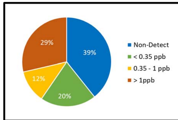
Figure ES.2: Maximum 1,4-Dioxane Concentrations in Groundwater at Sampled Inactive Landfills
