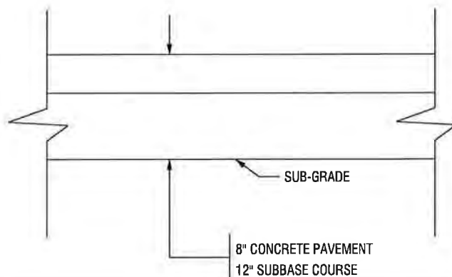
TYPICAL PROPOSED CONCRETE SECTION N.T.S.
