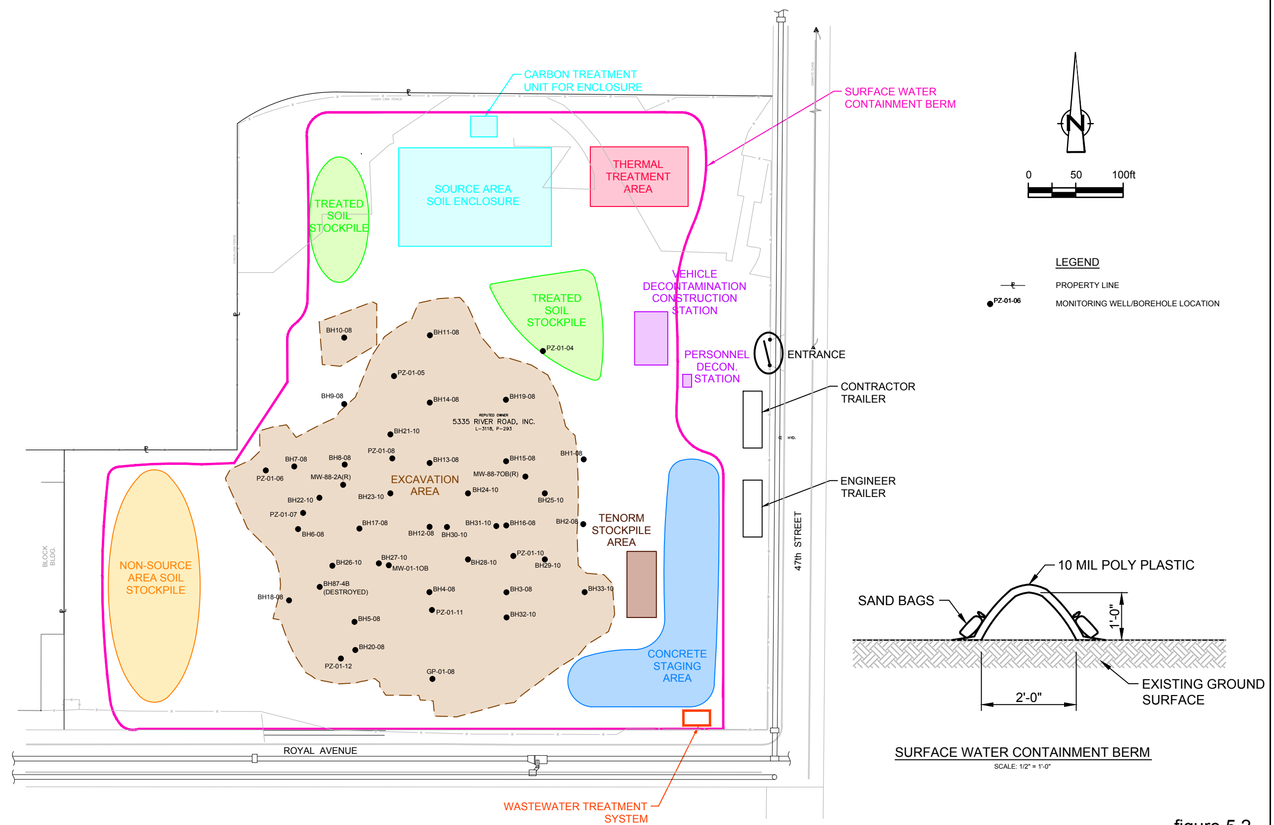
figure 5.2 TEMPORARY (DURING CONSTRUCTION) SURFACE WATER AND SEDIMENT CONTROL PLAN Frontier Chemical Site - Niagara Falls, New York
