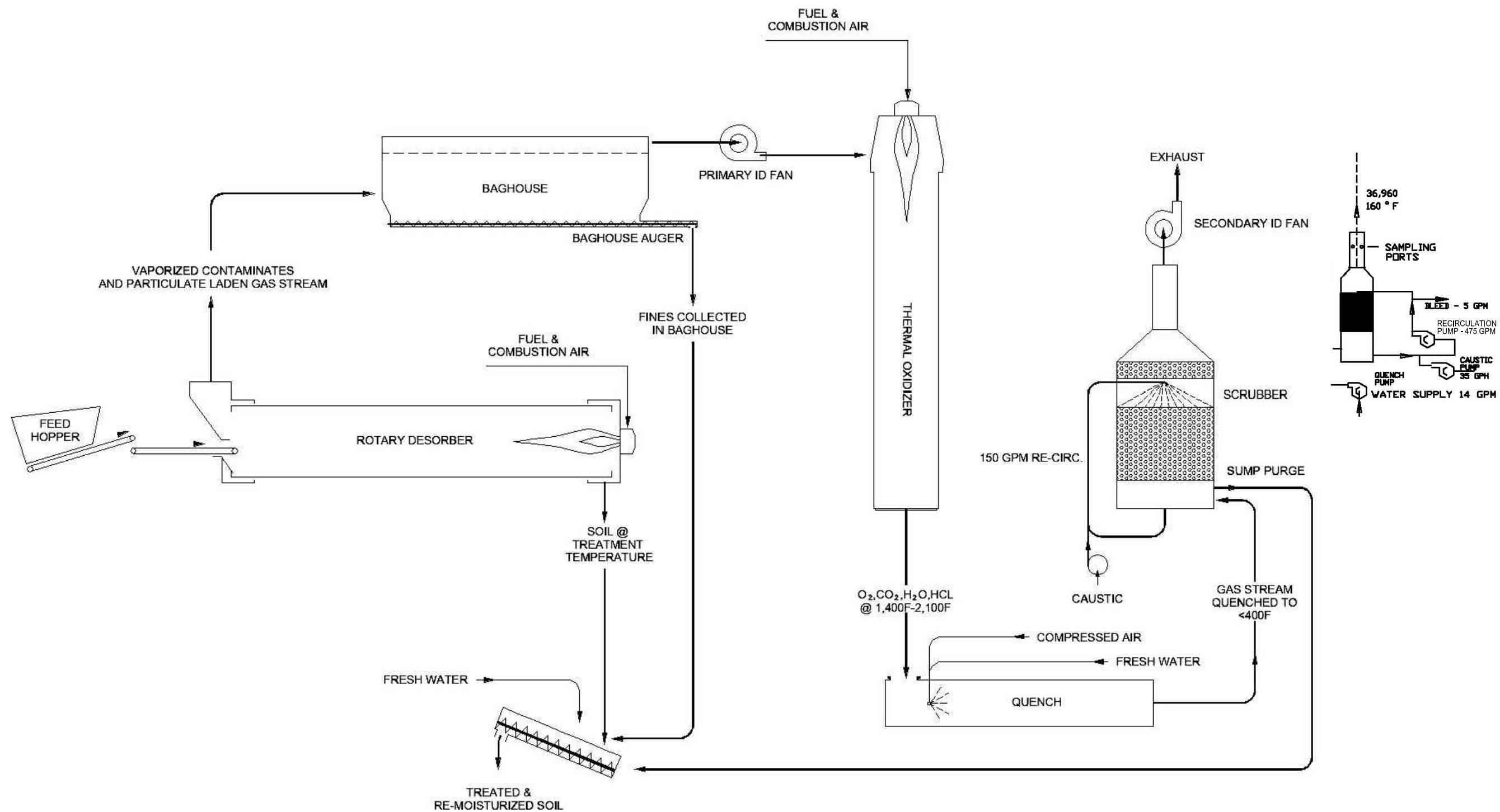
figure 5.10 SCHEMATIC OF THERMAL TREATMENT UNIT FRONTIER CHEMICAL SITE Niagara Falls, New York
