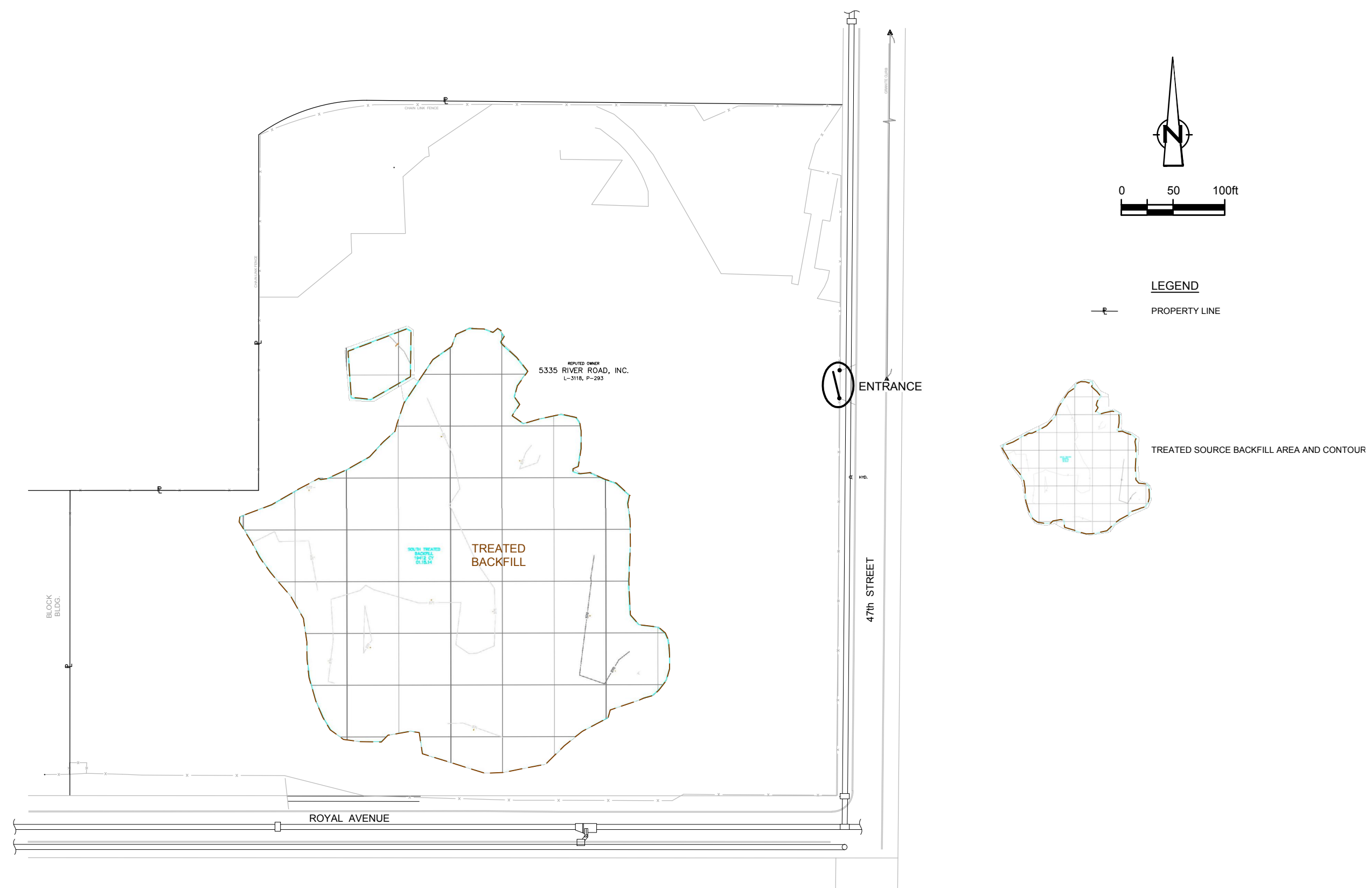
figure 5.5 TREATED SOURCE SOIL BACKFILL CONTOURS Frontier Chemical Site - Niagara Falls, New York
