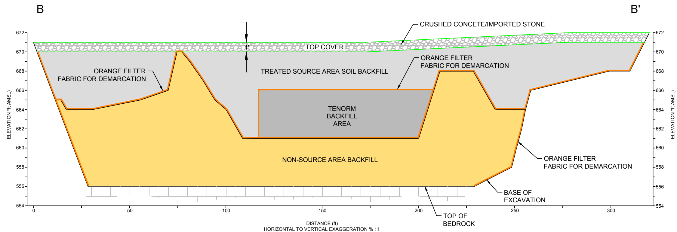
figure 5.8 CROSS-SECTION OF EXCAVATION AND BACKFILL AREAS Frontier Chemical Site - Niagara Falls, New York
