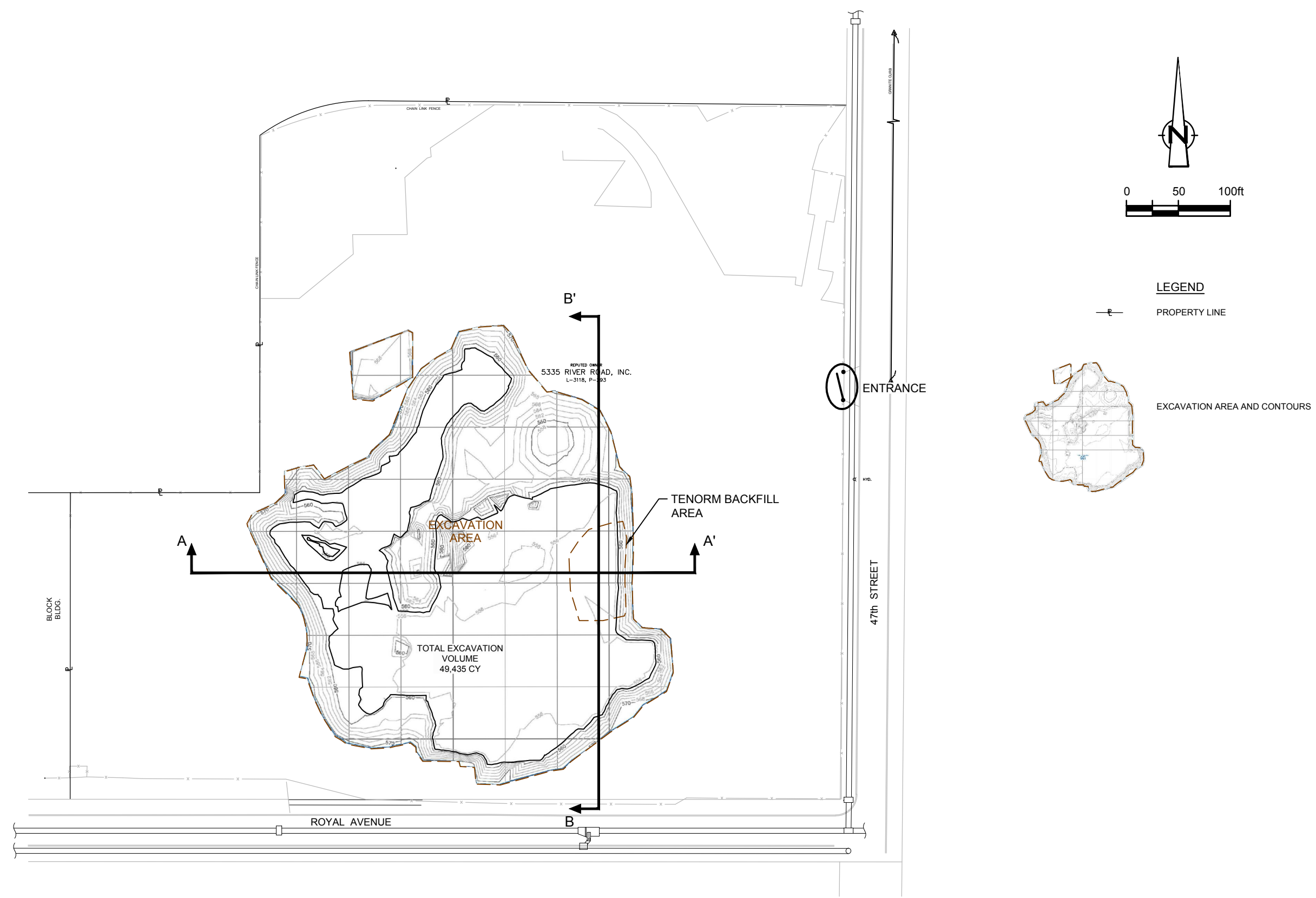
figure 5.9 CROSS-SECTION LOCATION Frontier Chemical Site - Niagara Falls, New York
