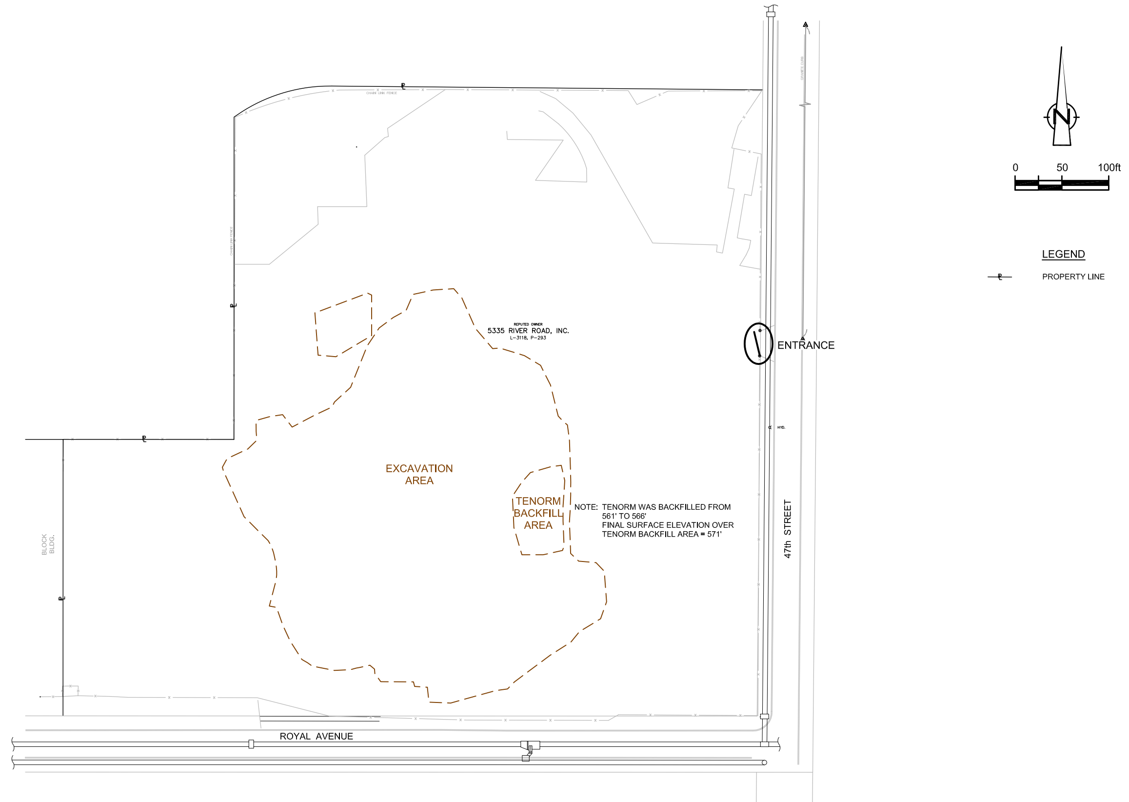
figure 5.7 TENORM BACKFILL AREA Frontier Chemical Site - Niagara Falls, New York
