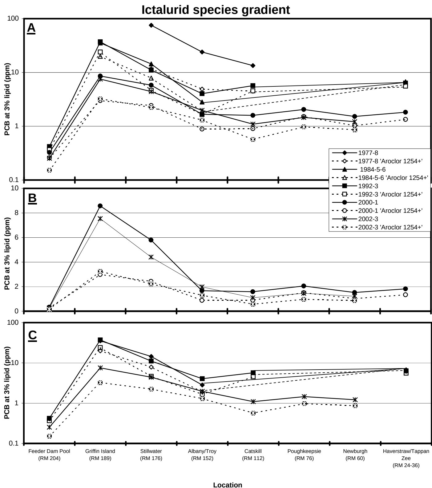
Figure 64. Spatial gradient of PCB concentrations for Ictalurid species collected during selected time periods from the Hudson River. Details of the accompanying ANOVA are provided in Table 47. Graphs are separated and presented on differing scales as noted to provide clarity. A). Gradient across all the selected years. B). Gradient for the most recent years (2000-01 vs. 2002-03). C). Gradients for the middle years (1984,85,86 and 1992,93) vs. 2002-03.
