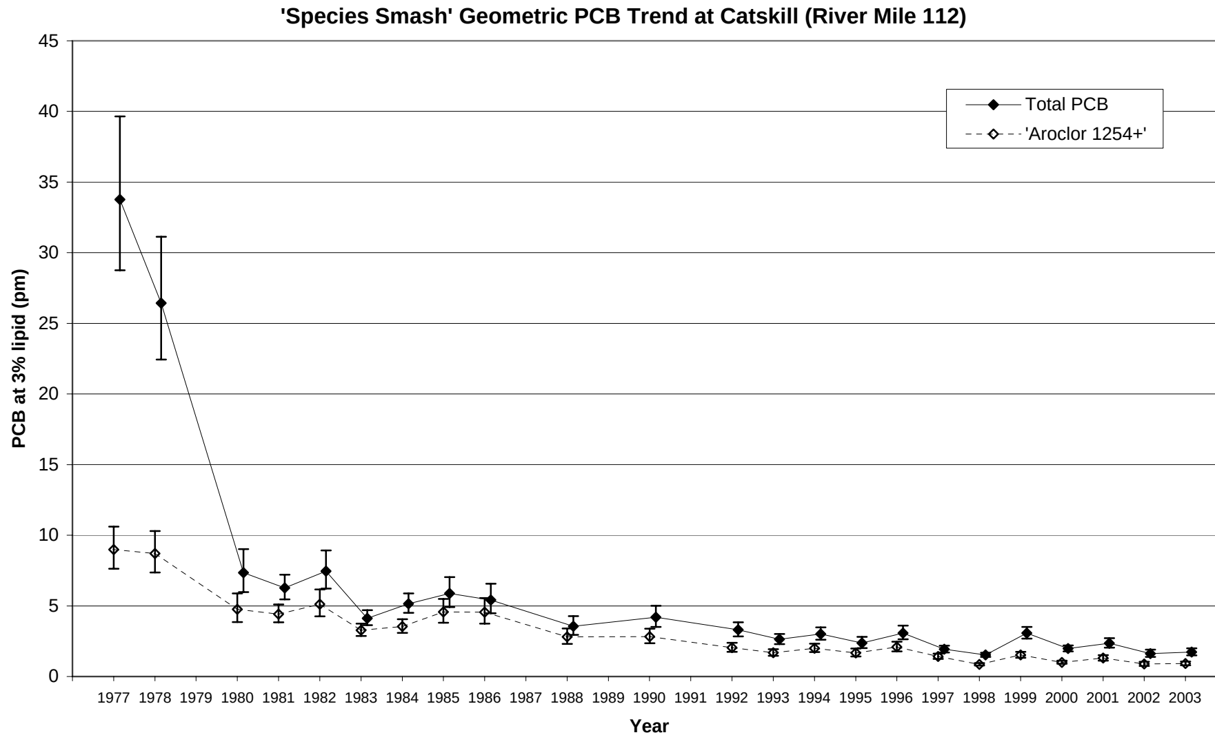
Figure 62. Trend in geometric PCB concentrations at 3% lipid for combined species ('Species Smash') collected at Catskill (River Mile 112). Results shown are least significant difference mean comparisons (95% confidence intervals) for total PCB - solid lines and higher chlorinated 'Aroclor 1254+' fraction - dashed lines.
