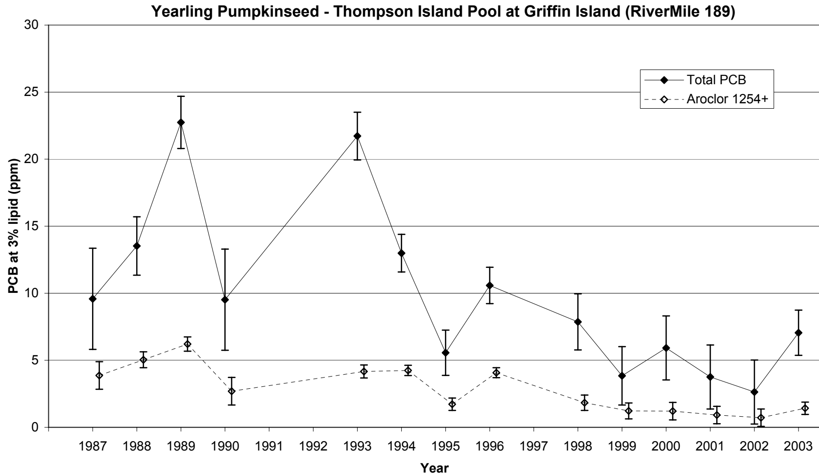
Figure 10. Trend in PCB concentrations at 3% lipid for yearling pumpkinseed collected at Griffin Island in the Thompson Island Pool (River mile 189). Results shown are Least Significant Difference mean comparisons (95% confidence intervals) for total PCB - solid lines, and higher chlorinated 'Aroclor 1254+' fraction - dashed lines.
