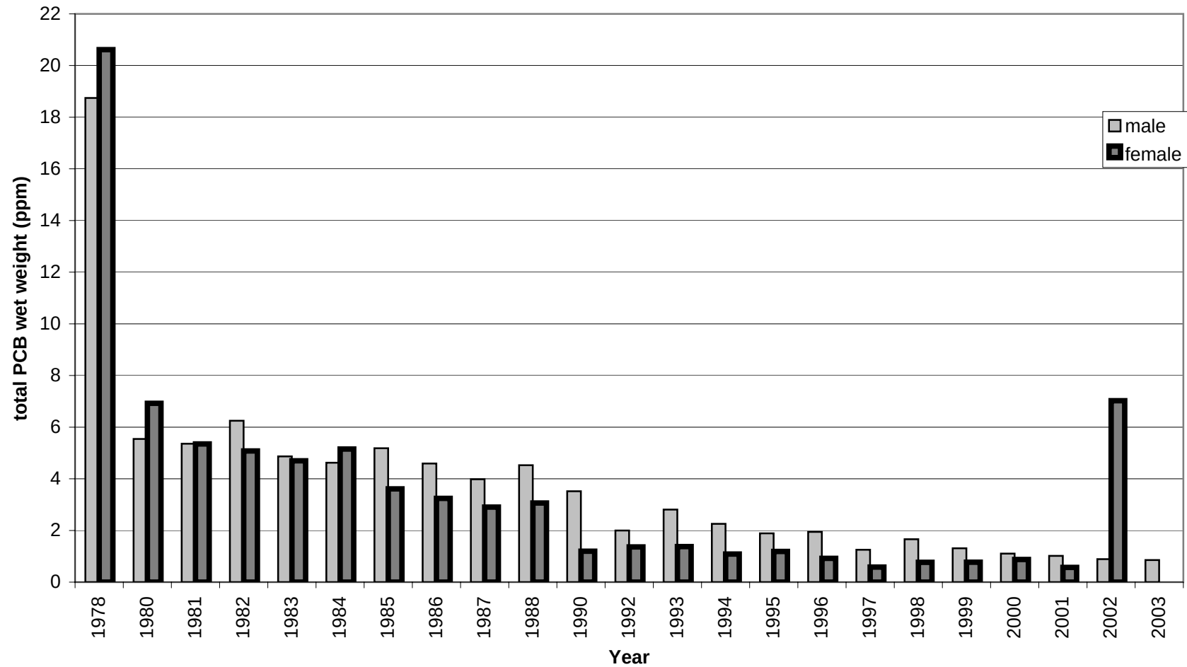
Figure 57A. Trend in wet weight total PCB concentrations in striped bass greater than 450 mm total length for each sex by year collected in the spring from Poughkeepsie to the George Washington Bridge which includes one female in 2002 with a wet weight total PCB concentration of 52.98 ppm. Results of a one-way ANOVA are provided in Table 45A1.
