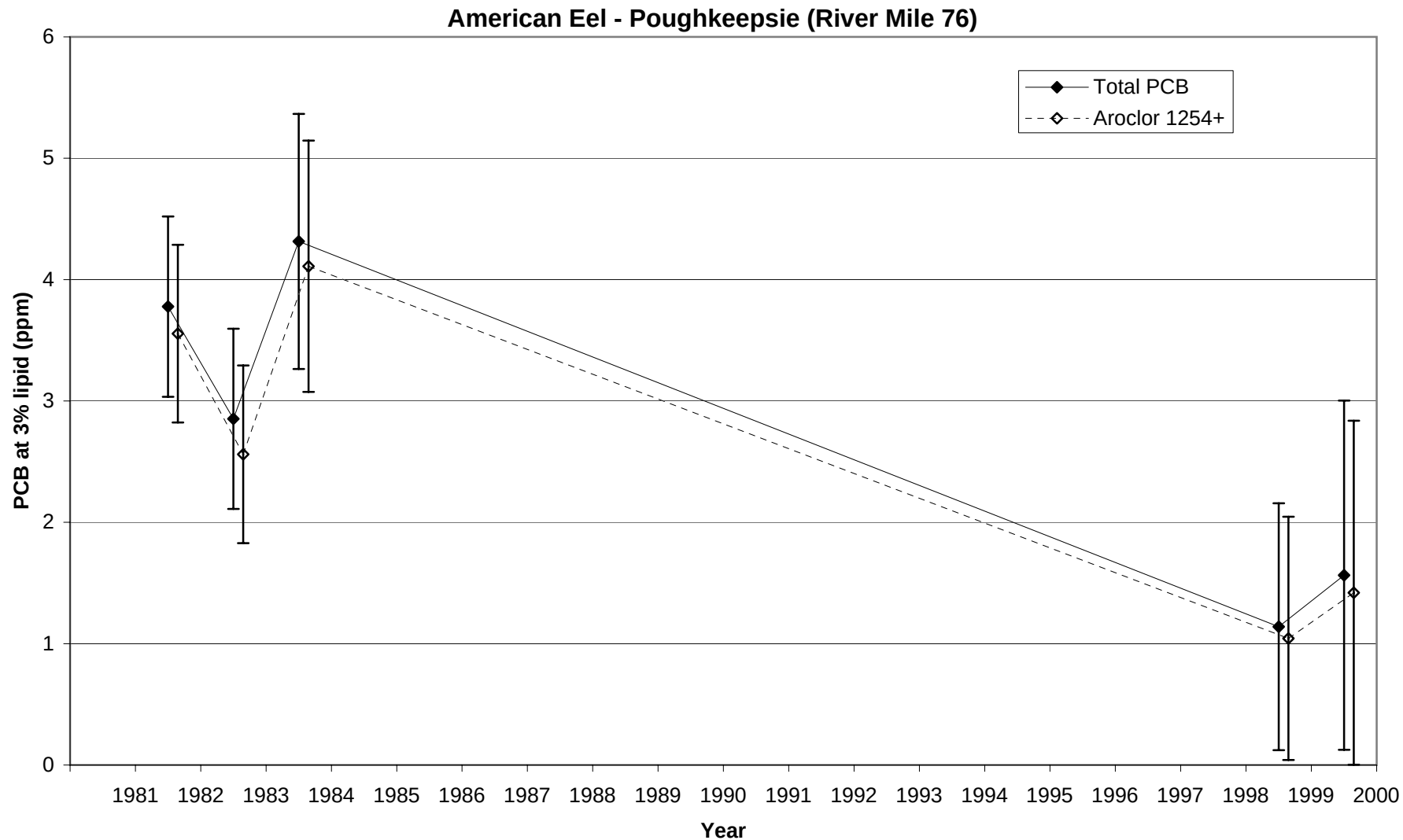
Figure 32. Trend in PCB concentrations at 3% lipid for American eel collected at Poughkeepsie in the lower Hudson River (River mile 76). Results shown are Least Significant Difference mean comparisons (95% confidence intervals) for total PCB - solid lines, and higher chlorinated 'Aroclor 1254+' fraction - dashed lines.
