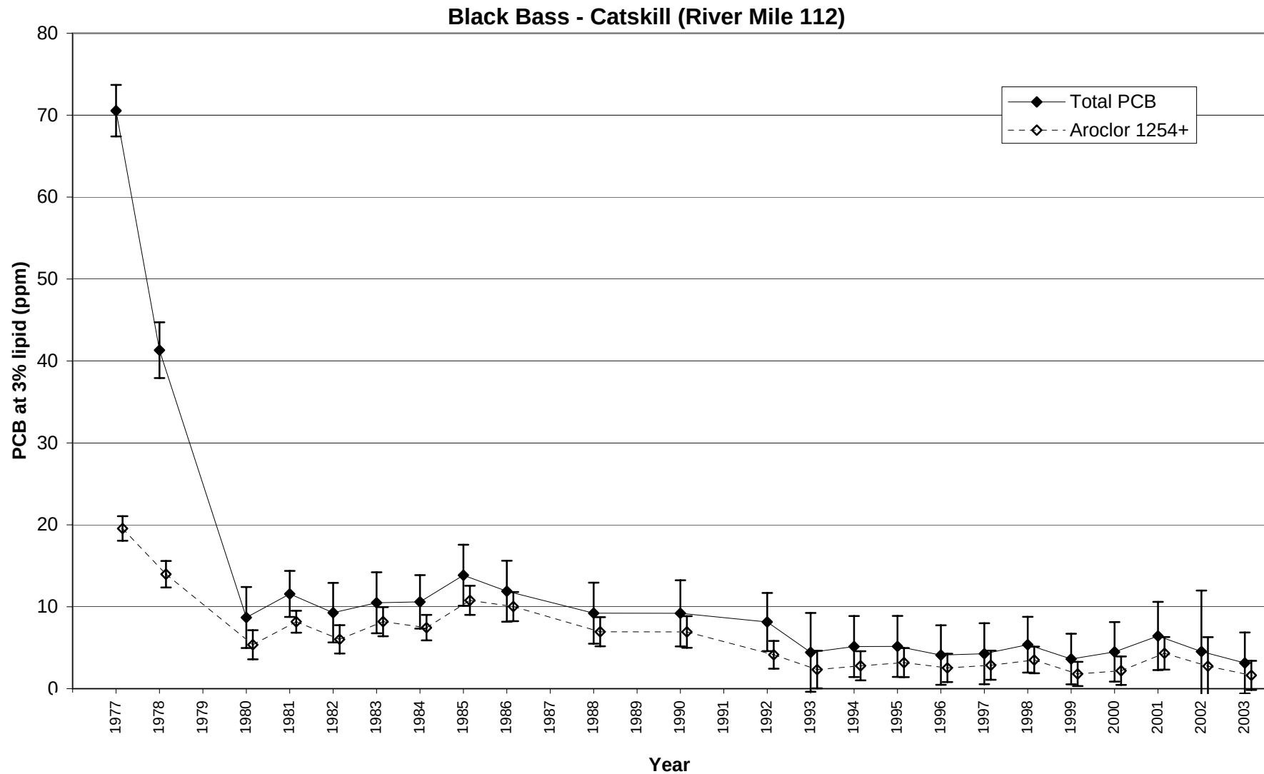
Figure 29A. Trend in PCB concentrations at 3% lipid for black bass collected at Catskill in the lower Hudson River (River mile 112). Results shown are Least Significant Difference mean comparisons (95% confidence intervals) for total PCB - solid lines, and higher chlorinated 'Aroclor 1254+' fraction - dashed lines.
