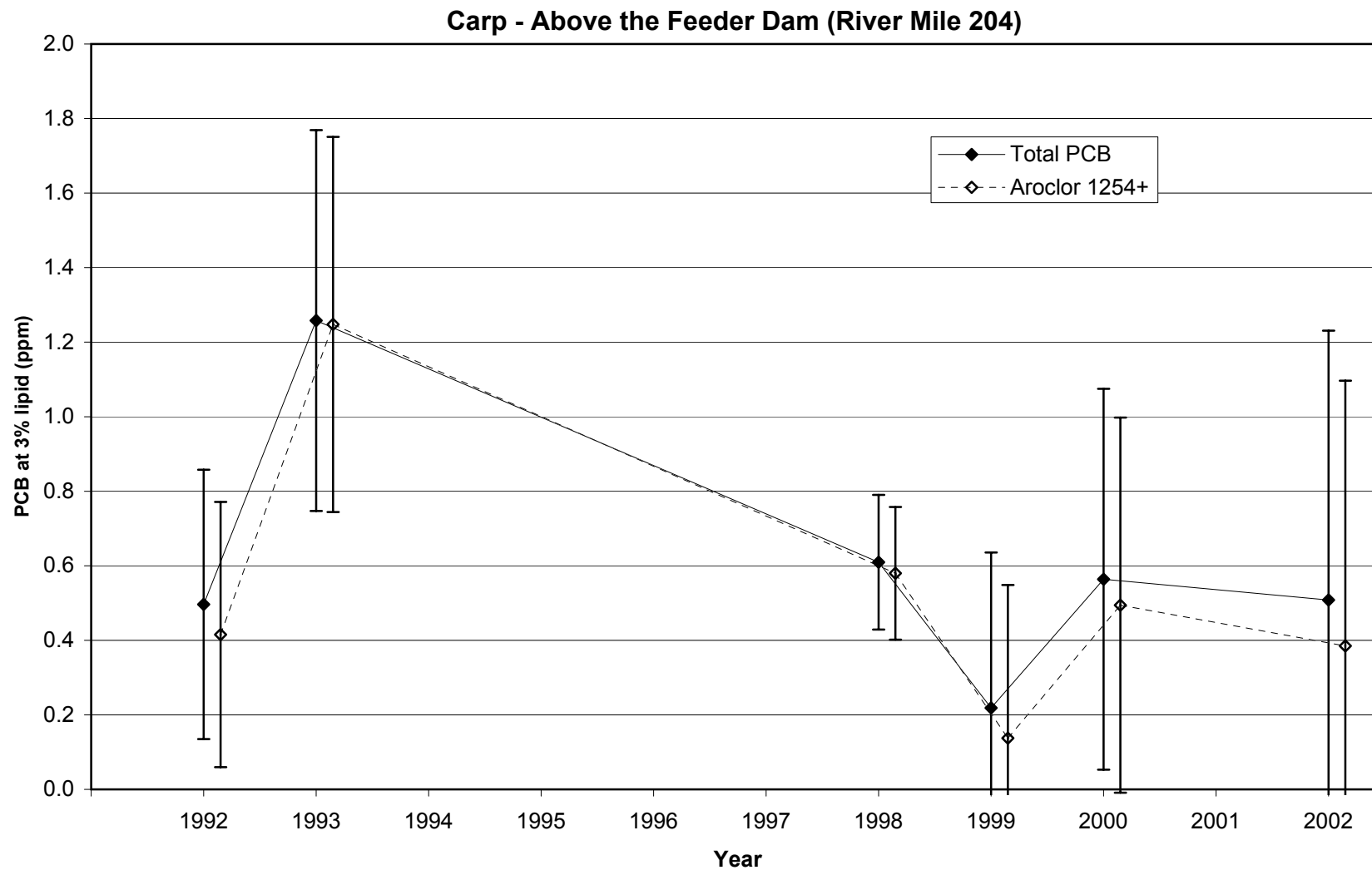
Figure 6. Trend in PCB concentrations at 3% lipid for carp collected above the Feeder Dam (River mile 204). Results shown are Least Significant Difference mean comparisons (95% confidence intervals) for total PCB - solid lines, and higher chlorinated 'Aroclor 1254+' fraction - dashed lines.
