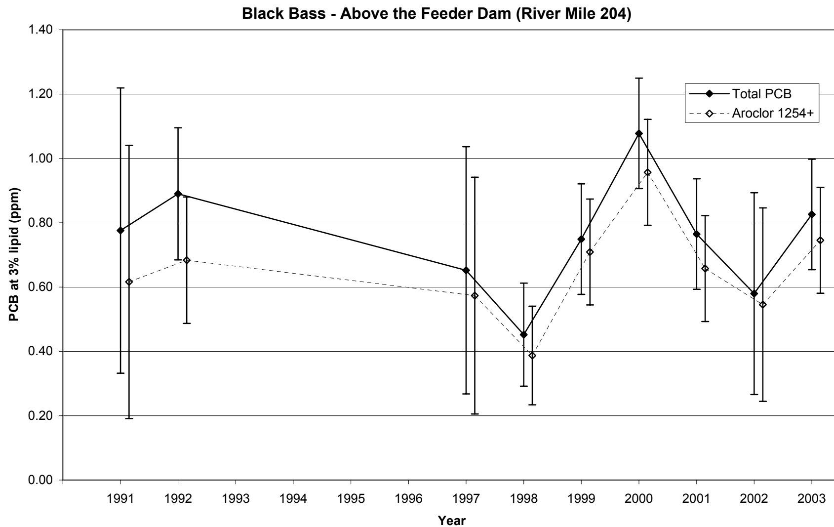
Figure 4. Trend in PCB concentrations at 3% lipid for black bass collected above the Feeder Dam (River mile 204). Results shown are Least Significant Difference mean comparisons (95% confidence intervals) for total PCB - solid lines, and higher chlorinated 'Aroclor 1254+' fraction - dashed lines.
