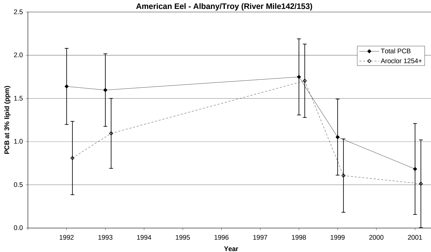
Figure 25. Trend in PCB concentrations at 3% lipid for American eel collected at Albany/Troy in the lower Hudson River (River mile 142/153). Results shown are Least Significant Difference mean comparisons (95% confidence intervals) for total PCB - solid lines, and higher chlorinated 'Aroclor 1254+' fraction - dashed lines.
