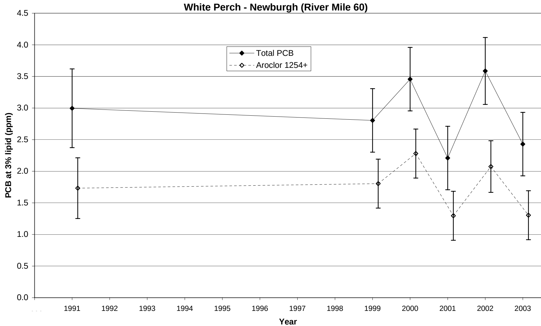
Figure 45. Trend in PCB concentrations at 3% lipid for white perch collected at Newburgh in the lower Hudson River (River mile 60). Results shown are Least Significant Difference mean comparisons (95% confidence intervals) for total PCB - solid lines, and higher chlorinated 'Aroclor 1254+' fraction - dashed lines.
