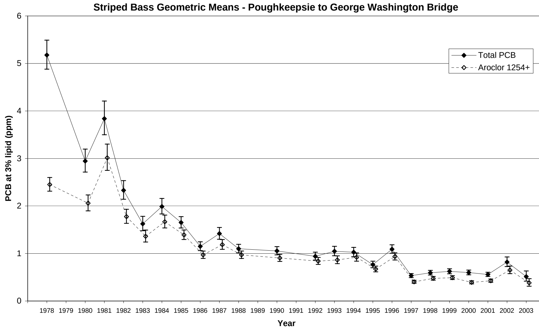
Figure 53. Trend in geometric PCB concentrations at 3% lipid for striped bass collected from Poughkeepsie to the George Washington Bridge in the lower Hudson River (River mile 76-12). Results shown are Least Significant Difference mean comparisons (95% confidence intervals) for total PCB - solid lines, and the higher chlorinated 'Aroclor 1254+' fraction - dashed lines.
