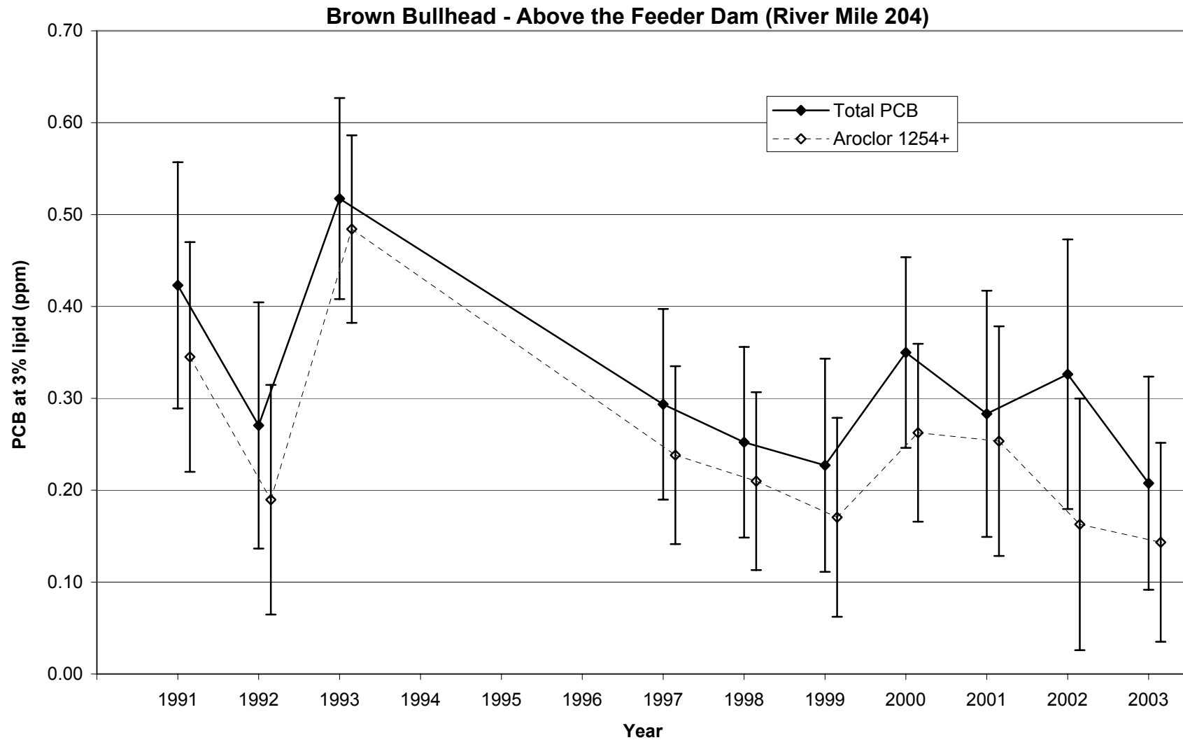
Figure 5. Trend in PCB concentrations at 3% lipid for brown bullhead collected above the Feeder Dam (River mile 204). Results shown are Least Significant Difference mean comparisons (95% confidence intervals) for total PCB - solid lines, and higher chlorinated 'Aroclor 1254+' fraction - dashed lines.
