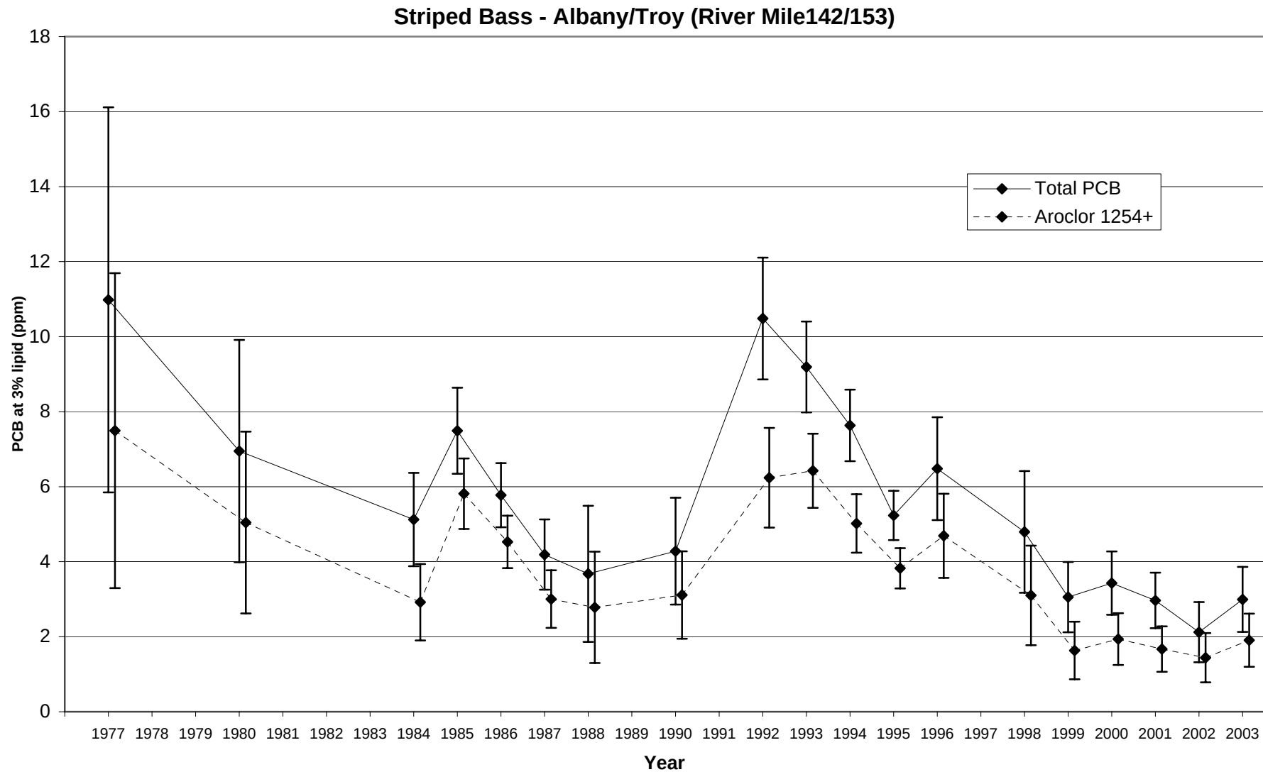
Figure 22. Trend in PCB concentrations at 3% lipid for striped bass collected at Albany/Troy in the lower Hudson River (River mile 142/153). Results shown are Least Significant Difference mean comparisons (95% confidence intervals) for total PCB - solid lines, and higher chlorinated 'Aroclor 1254+' fraction - dashed lines.
