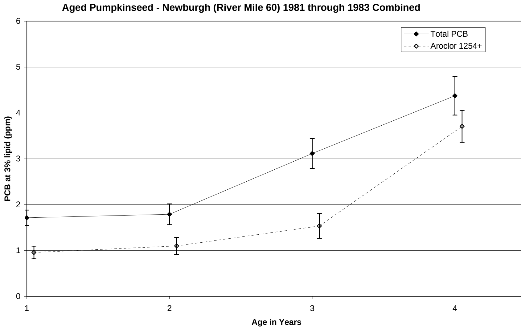
Figure 43. Comparison of PCB concentrations at 3% lipid by age for pumpkinseed collected at Newburgh in the lower Hudson River (River mile 60) for 1981 through 1983 combined. Results shown are Least Significant Difference mean comparisons (95% confidence intervals) for total PCB - solid lines, and the higher chlorinated 'Aroclor 1254+' fraction - dashed lines.
