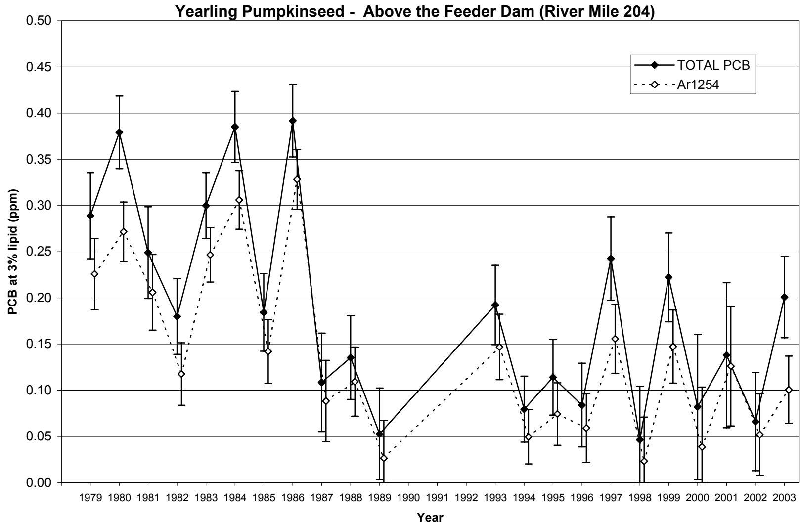
Figure 3. Trend in PCB concentrations at 3% lipid for yearling pumpkinseed collected above the Feeder Dam (River mile 204). Results shown are Least Significant Difference mean comparisons (95% confidence intervals) for total PCB - solid lines, and higher chlorinated 'Aroclor 1254+' fraction - dashed lines.
