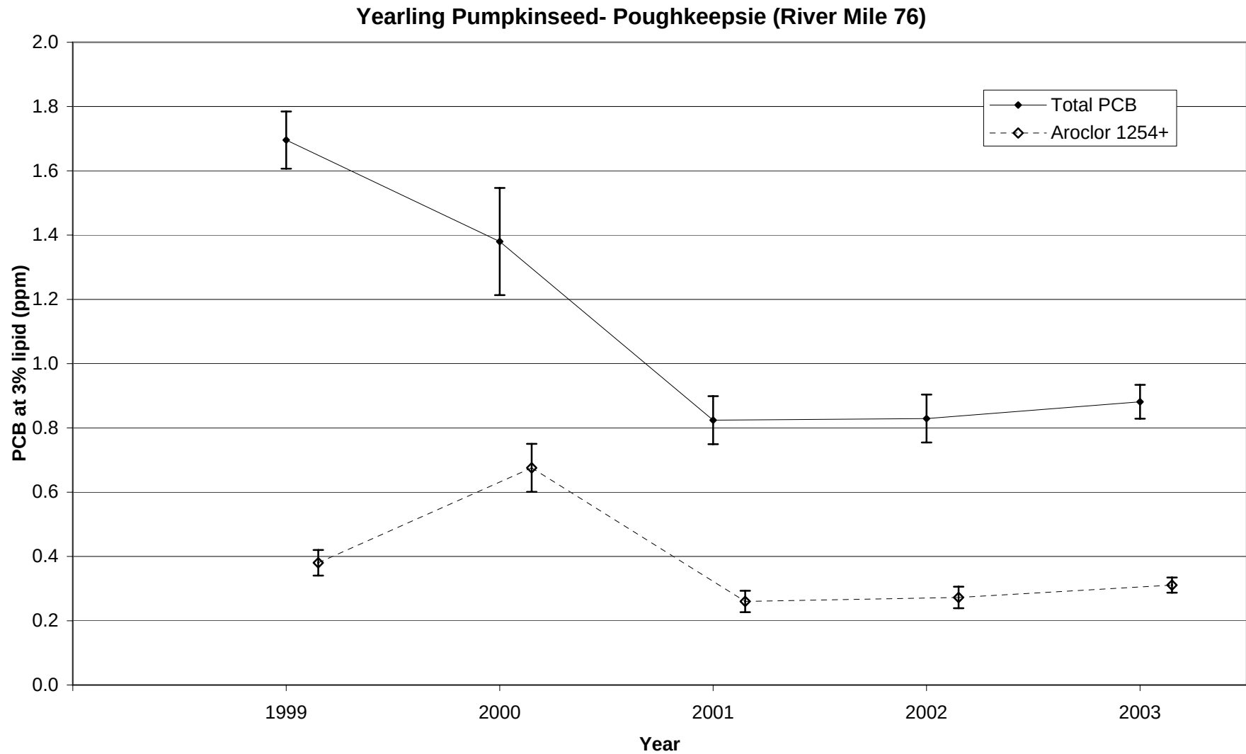
Figure 37. Trend in PCB concentrations at 3% lipid for yearling pumpkinseed collected at Poughkeepsie in the lower Hudson River (River mile 76). Results shown are Least Significant Difference mean comparisons (95% confidence intervals) for total PCB - solid lines, and higher chlorinated 'Aroclor 1254+' fraction - dashed lines.
