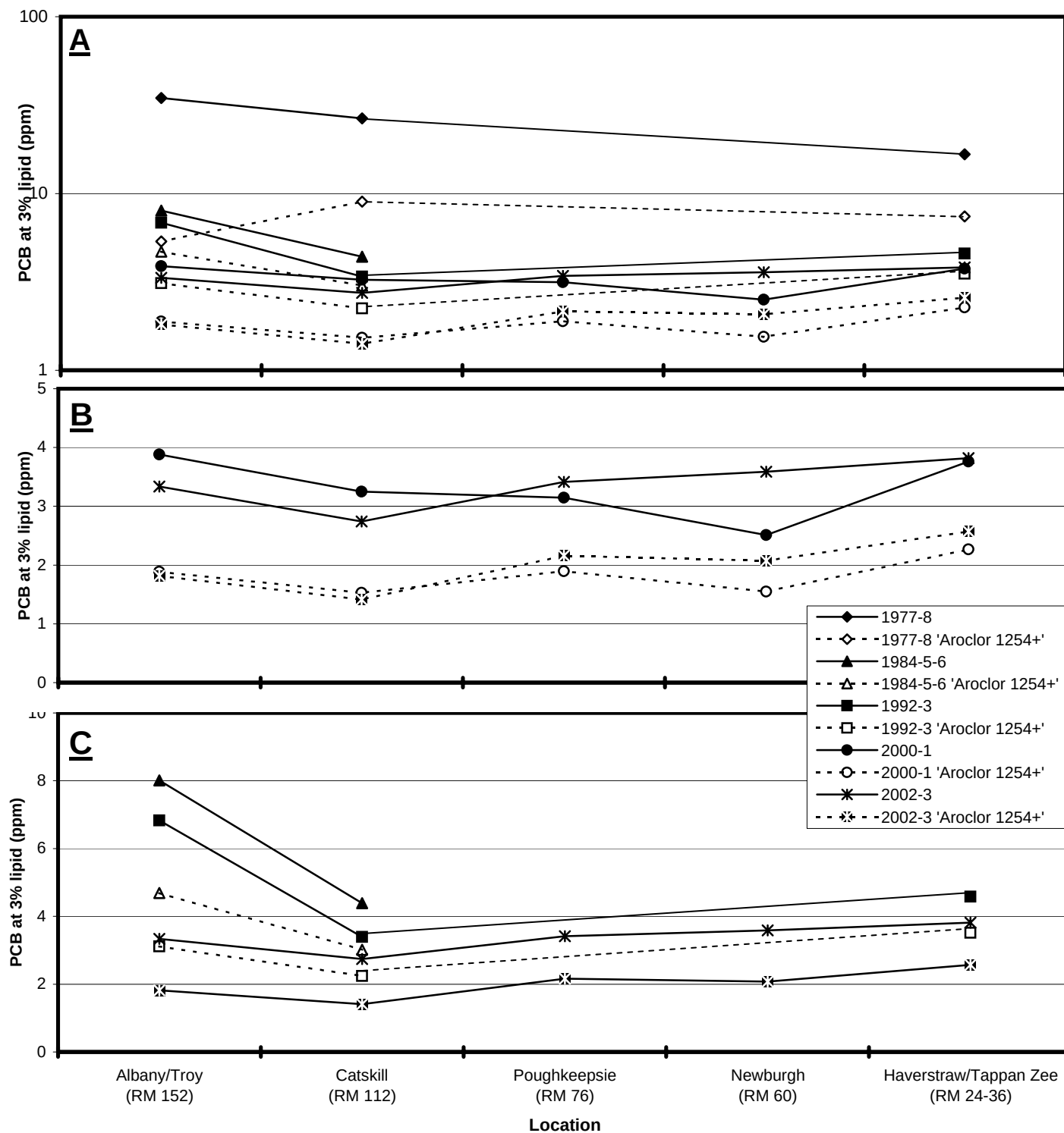
Figure 66. Spatial gradient of PCB concentrations for white perch collected during selected time periods from the Hudson River. Details of the accompanying ANOVA are provided in Table 49. Graphs are separated and presented on differing scales as noted to provide clarity. A). Gradient across all the selected years. B). Gradient for the most recent years (2000-01 vs. 2002-03). C). Gradients for the middle years (1984,85,86 and 1992,93) vs. 2002-03.
