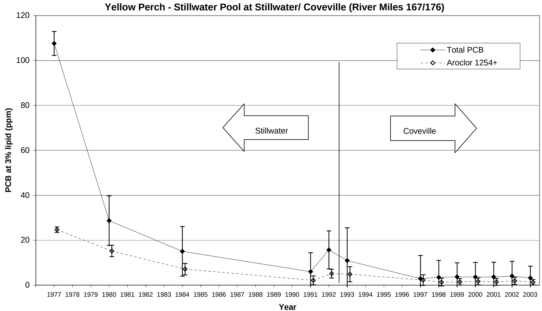
Figure 16. Trend in PCB concentrations at 3% lipid for yellow perch collected at Stillwater/Coveville in the Stillwater Pool (River miles 167/176). Results shown are Least Significant Difference mean comparisons (95% confidence intervals) for total PCB - solid lines, and higher chlorinated 'Aroclor 1254+' fraction - dashed lines.
