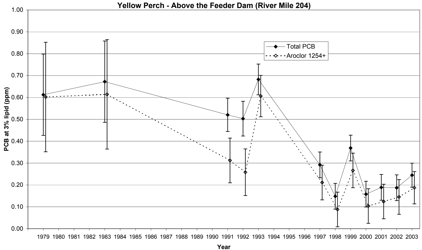
Figure 2. Trend in PCB concentrations at 3% lipid for yellow perch collected above the Feeder Dam (River mile 204). Results shown are Least Significant Difference mean comparisons (95% confidence intervals) for total PCB - solid lines, and higher chlorinated 'Aroclor 1254+' fraction - dashed lines.
