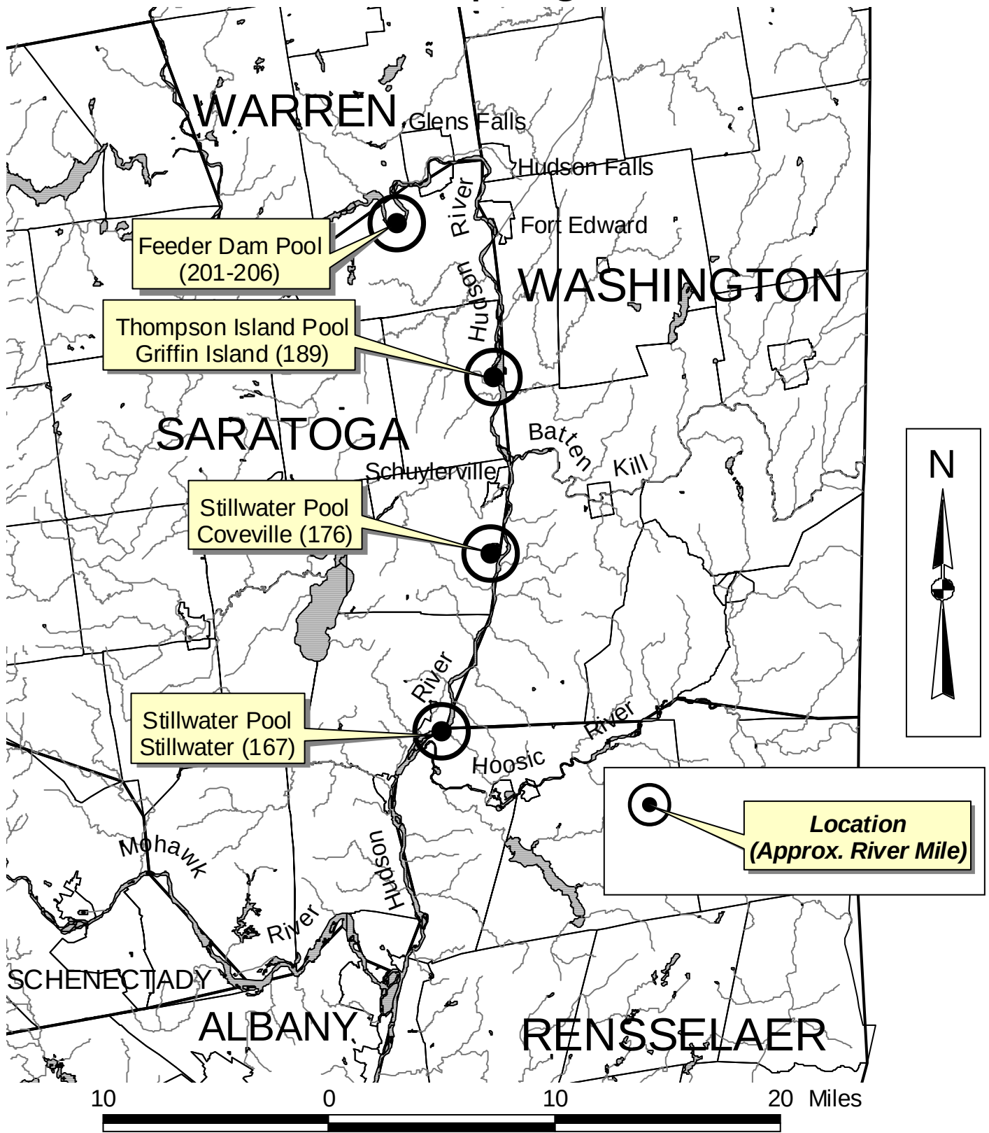
Figure 1A. Fish PCB trend analysis sampling locations in the upper Hudson River above the confluence with the Mohawk River. River miles are measured from Battery Park in New York City (River mile 0).
