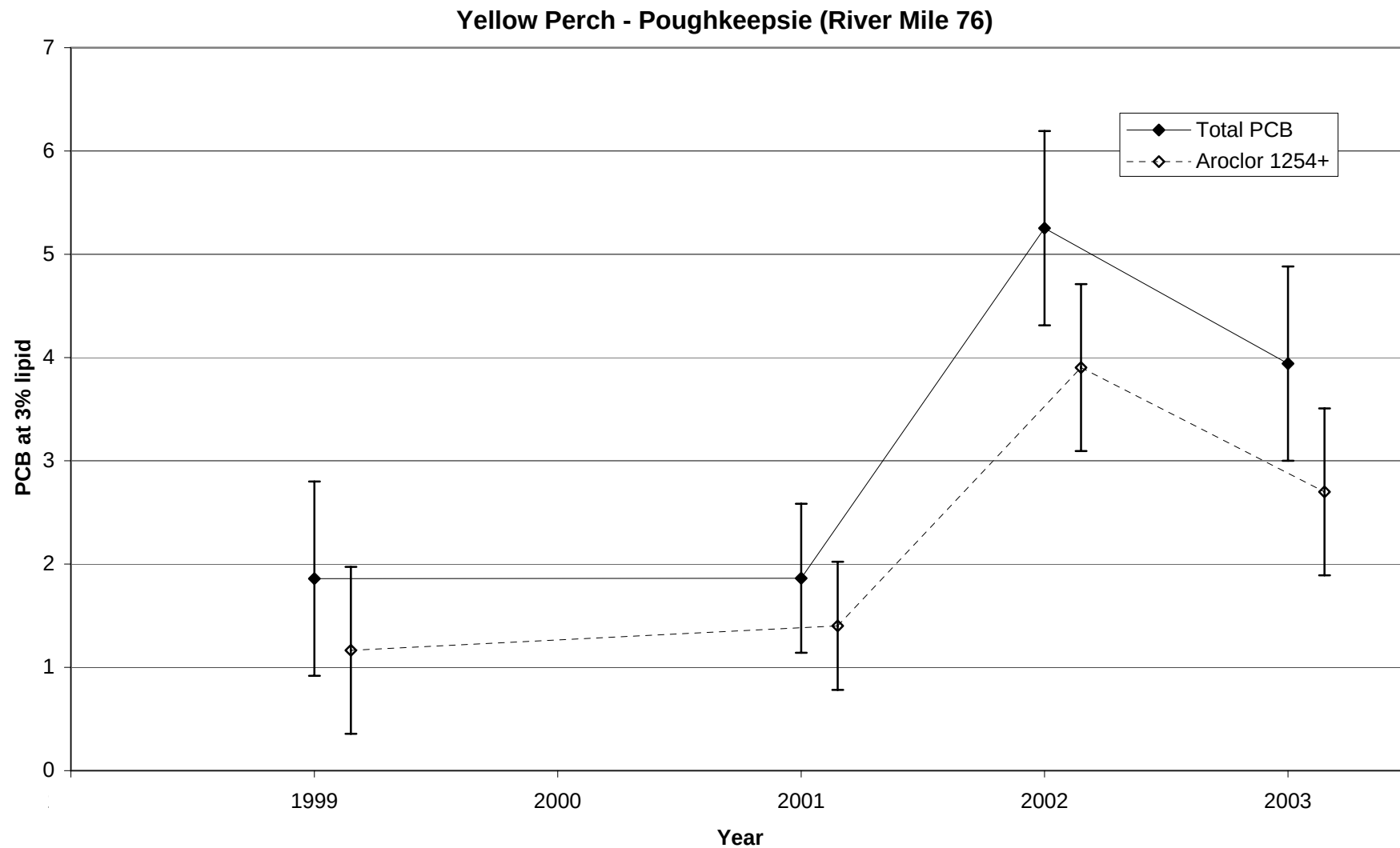
Figure 38. Trend in PCB concentrations at 3% lipid for yellow perch collected at Poughkeepsie in the lower Hudson River (River mile 76). Results shown are Least Significant Difference mean comparisons (95% confidence intervals) for total PCB - solid lines, and higher chlorinated 'Aroclor 1254+' fraction - dashed lines.
