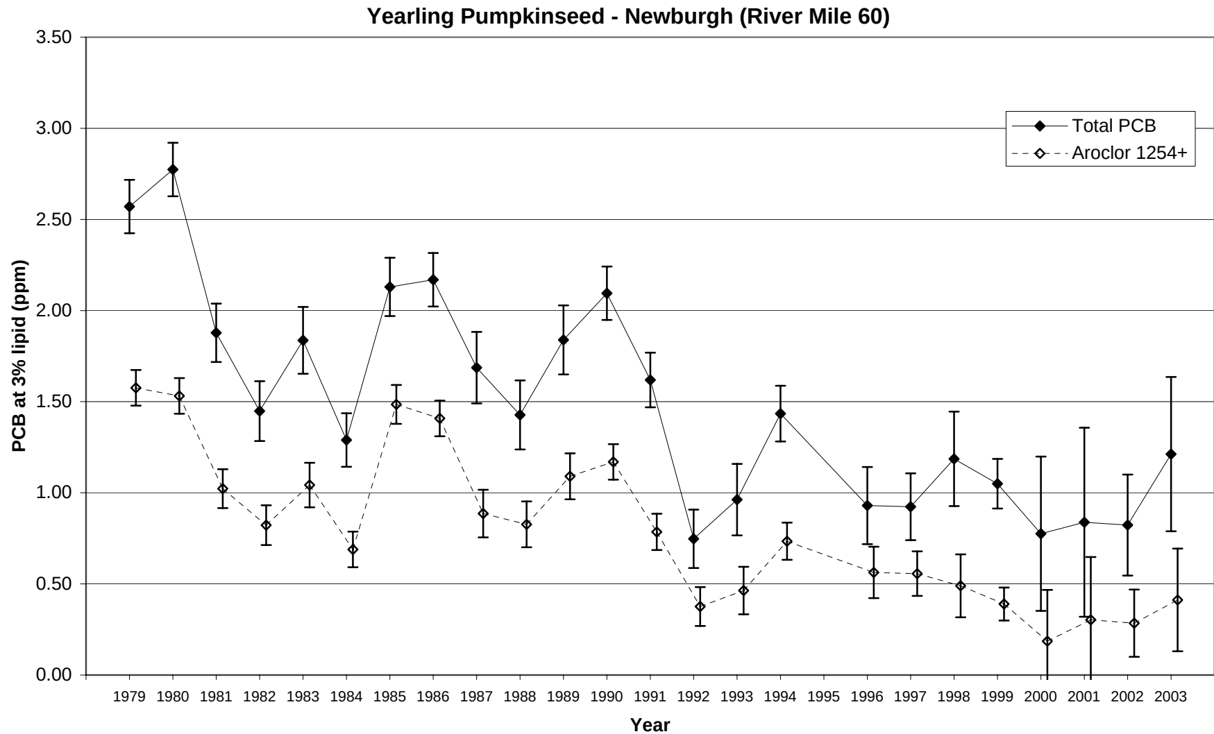
Figure 42. Trend in PCB concentrations at 3% lipid for yearling pumpkinseeds collected at Newburgh in the lower Hudson River (River mile 60). Results shown are Least Significant Difference mean comparisons (95% confidence intervals) for total PCB - solid lines, and higher chlorinated 'Aroclor 1254+' fraction - dashed lines.
