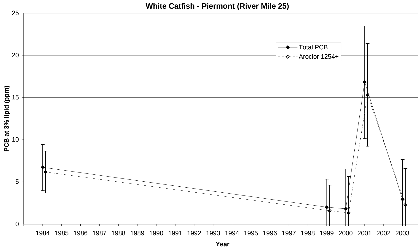
Figure 50. Trend in PCB concentrations at 3% lipid for White Catfish collected near Piermont in the lower Hudson River (River mile 25). Results shown are Least Significant Difference mean comparisons (95% confidence intervals) for total PCB - solid lines, and higher chlorinated 'Aroclor 1254+' fraction - dashed lines.
