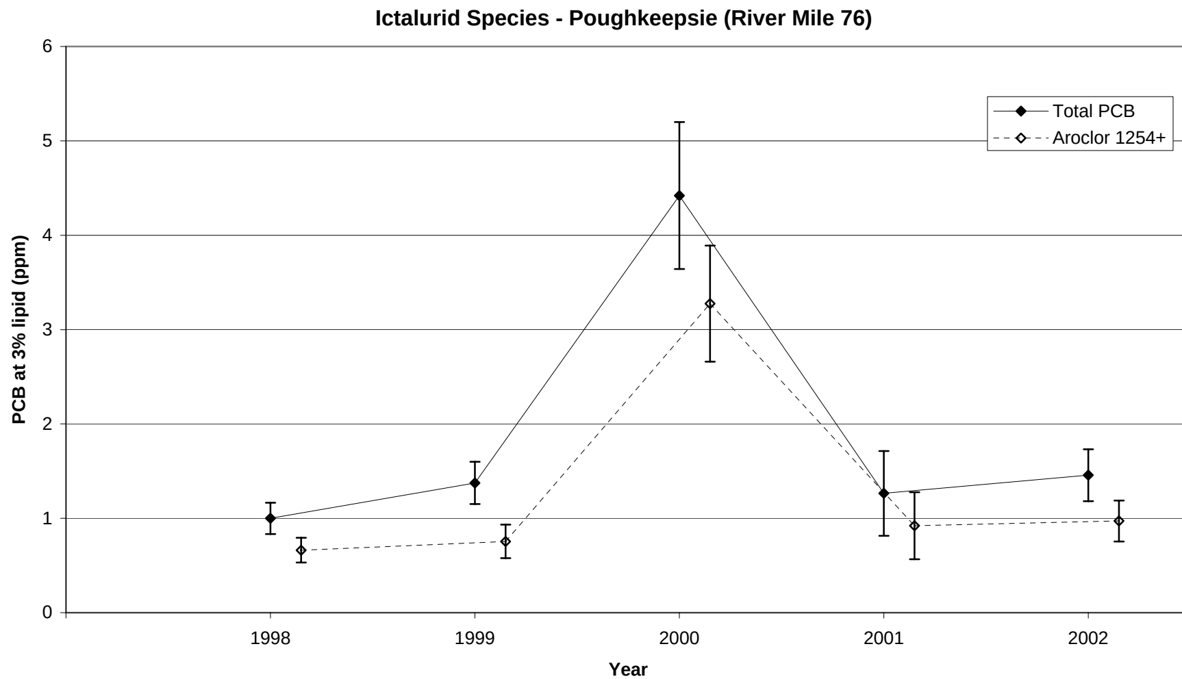
Figure 36. Trend in PCB concentrations at 3% lipid for Ictalurid species collected at Poughkeepsie in the lower Hudson River (River mile 76). Results shown are Least Significant Difference mean comparisons (95% confidence intervals) for total PCB - solid lines, and higher chlorinated 'Aroclor 1254+' fraction - dashed lines.
