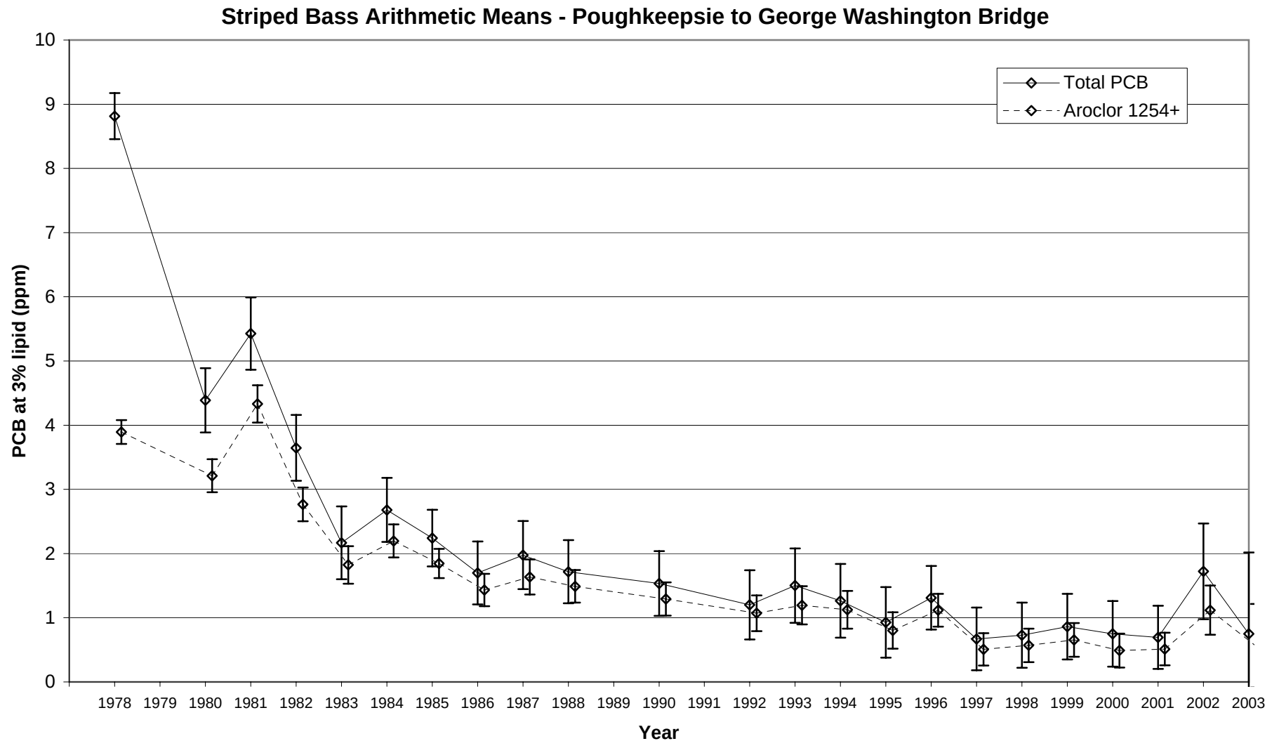
Figure 52. Trend in arithmetic PCB concentrations at 3% lipid for striped bass collected from Poughkeepsie to George Washington Bridge in the lower Hudson River (River mile 76-12). Results shown are Least Significant Difference mean comparisons (95% confidence intervals) for total PCB - solid lines, and the higher chlorinated 'Aroclor 1254+' fraction - dashed lines.
