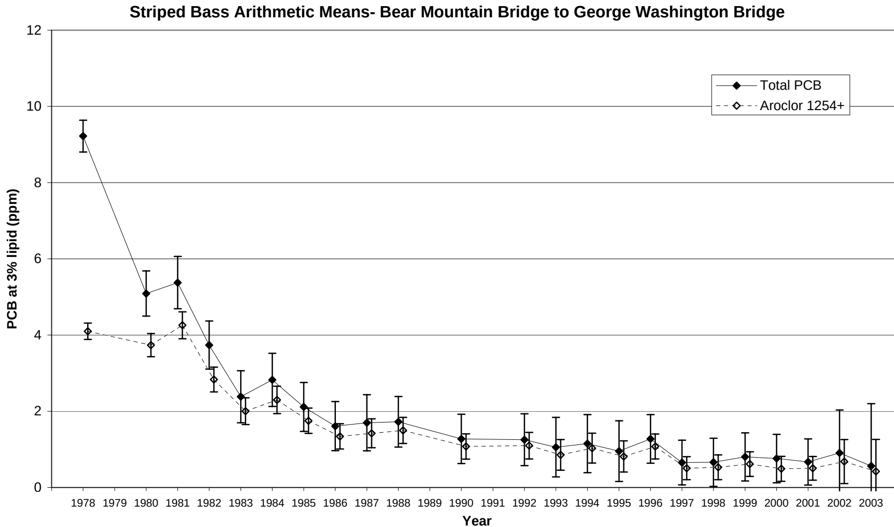
Figure 54. Trend in arithmetic PCB concentrations at 3% lipid for striped bass collected from the Bear Mountain Bridge to the George Washington Bridge in the lower Hudson River (River miles 47-12). Results shown are Least Significant Difference mean comparisons (95% confidence intervals) for total PCB - solid lines, and the higher chlorinated 'Aroclor 1254+' fraction - dashed lines.
