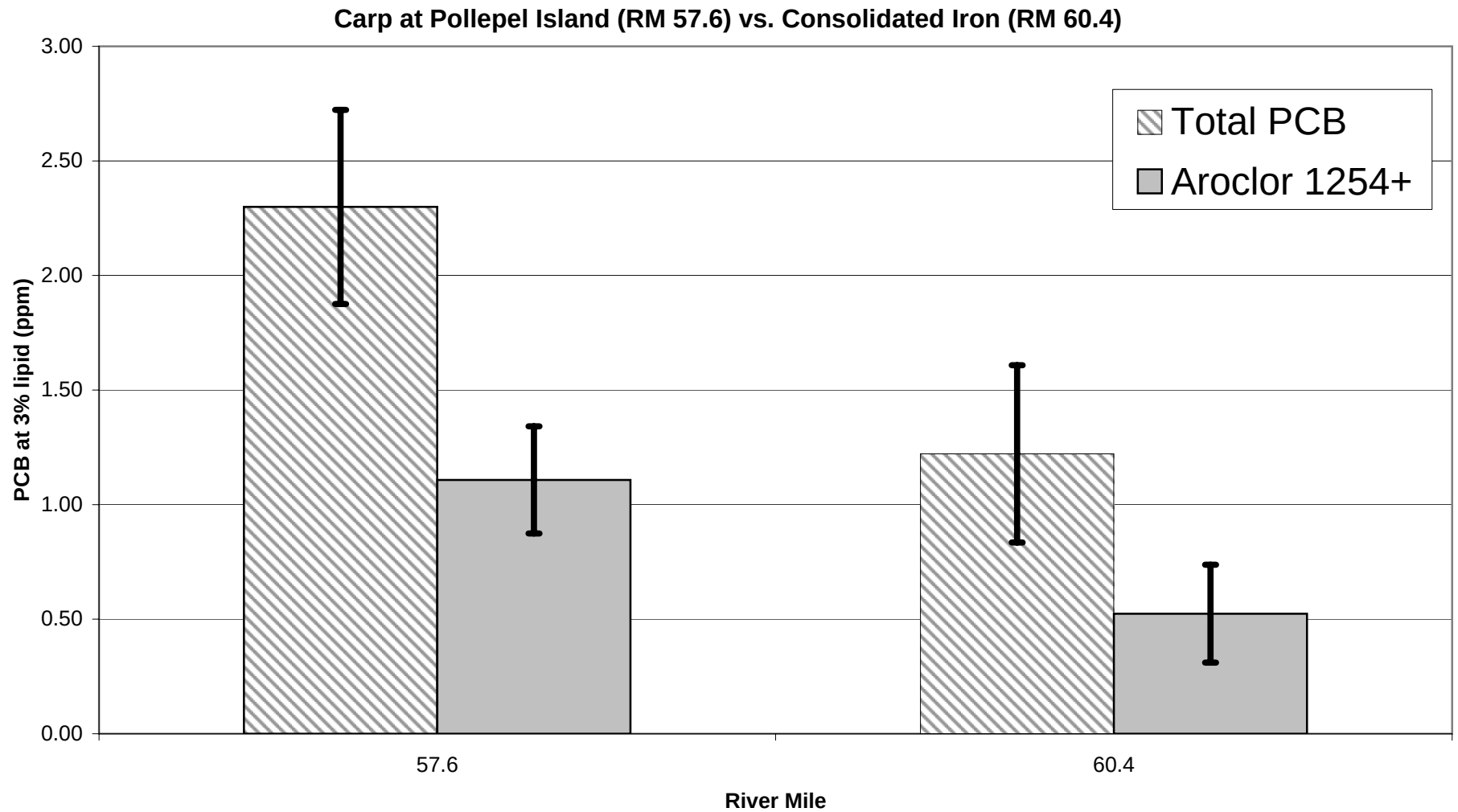
Figure 47. Comparison of PCB concentrations at 3% lipid for carp collected at two locations near Newburgh in the lower Hudson River (River mile 60). Results shown are Least Significant Difference mean comparisons (95% confidence intervals) for total PCB - diagonal lines, and the higher chlorinated 'Aroclor 1254+' fraction - solid fill.
