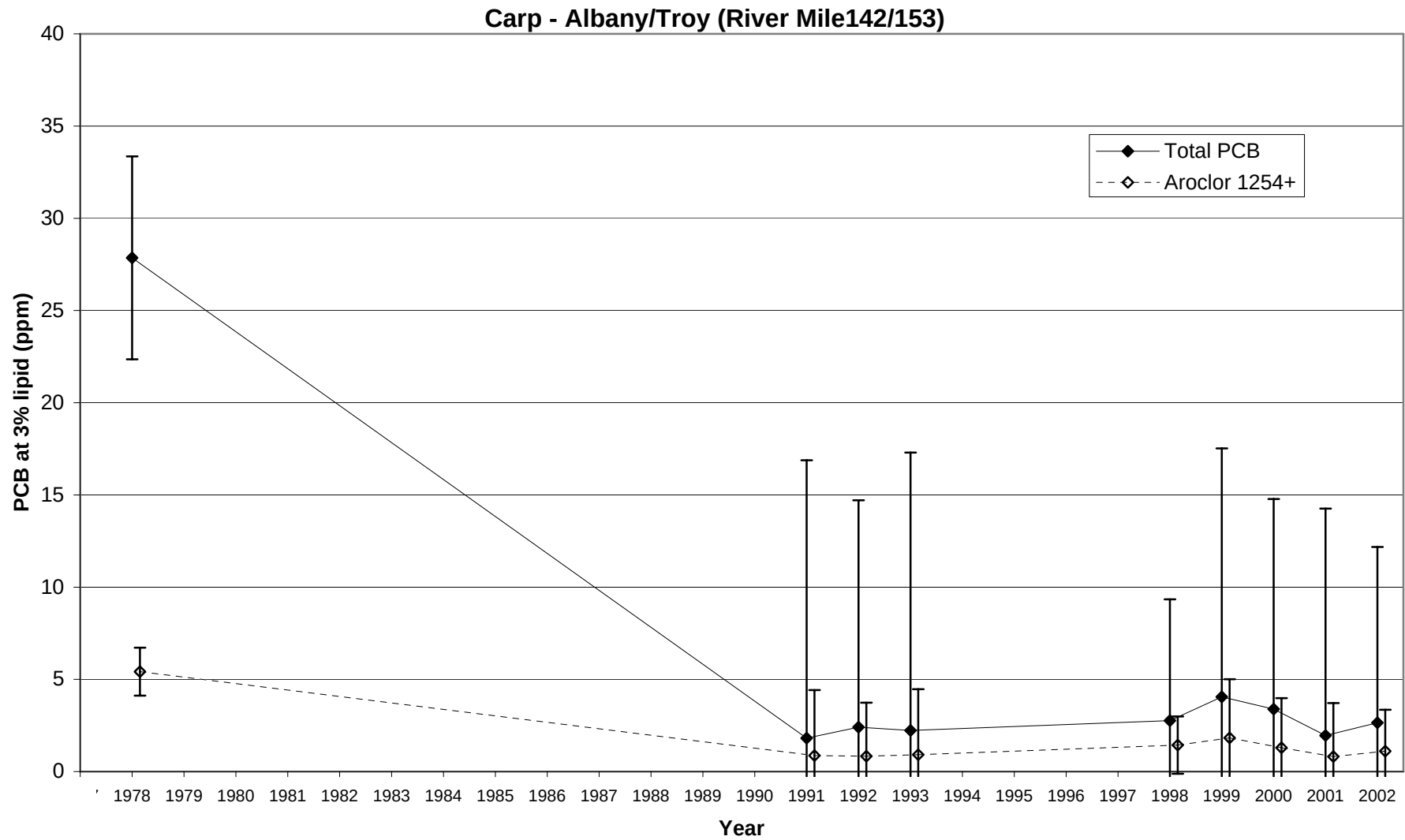
Figure 24. Trend in PCB concentrations at 3% lipid for carp collected at Albany/Troy in the lower Hudson River (River mile 142/153). Results shown are Least Significant Difference mean comparisons (95% confidence intervals) for total PCB - solid lines, and higher chlorinated 'Aroclor 1254+' fraction - dashed lines.
