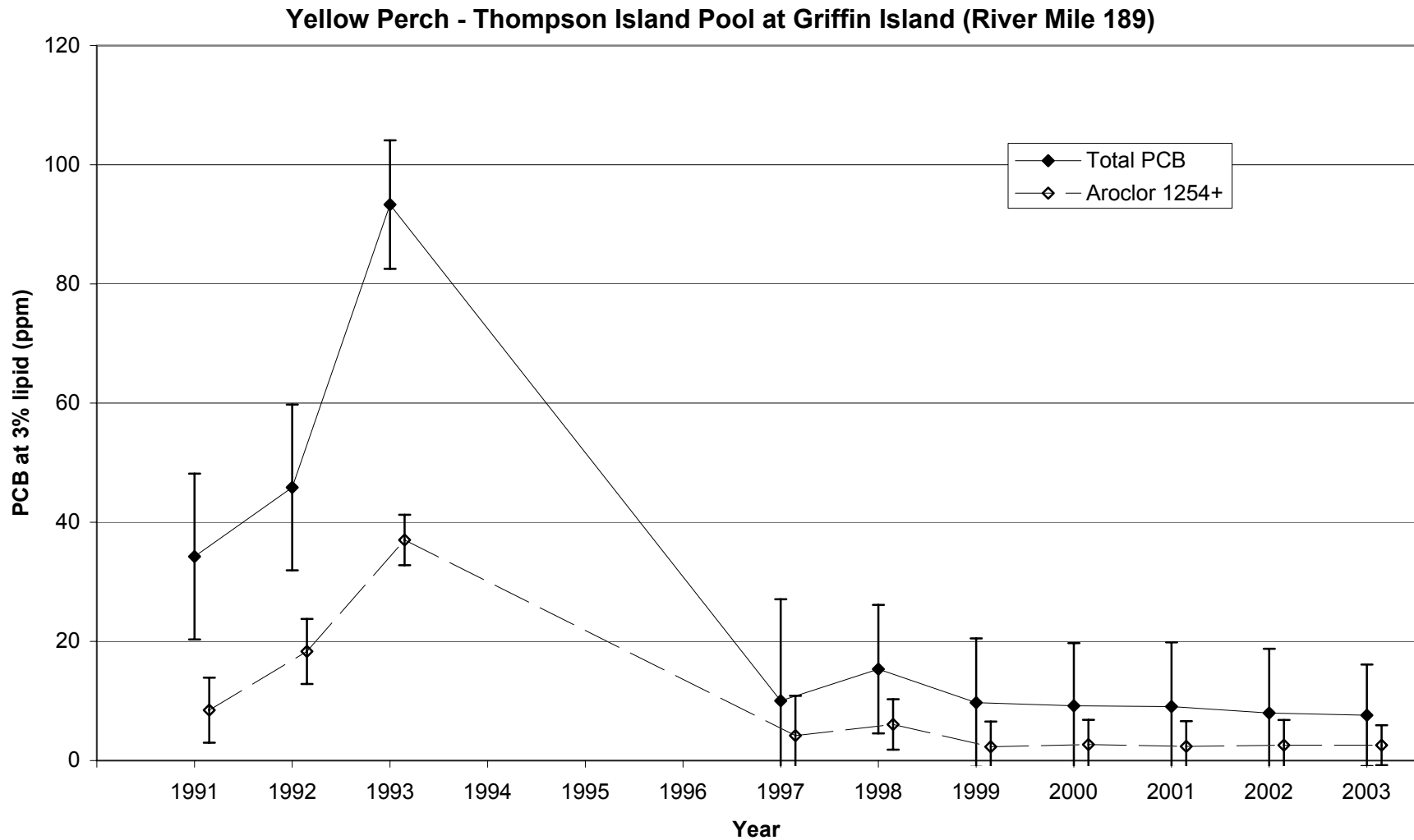
Figure 11. Trend in PCB concentrations at 3% lipid for yellow perch collected at Griffin Island in the Thompson Island Pool (River mile 189). Results shown are Least Significant Difference mean comparisons (95% confidence intervals) for total PCB - solid lines, and higher chlorinated 'Aroclor 1254+' fraction - dashed lines.
