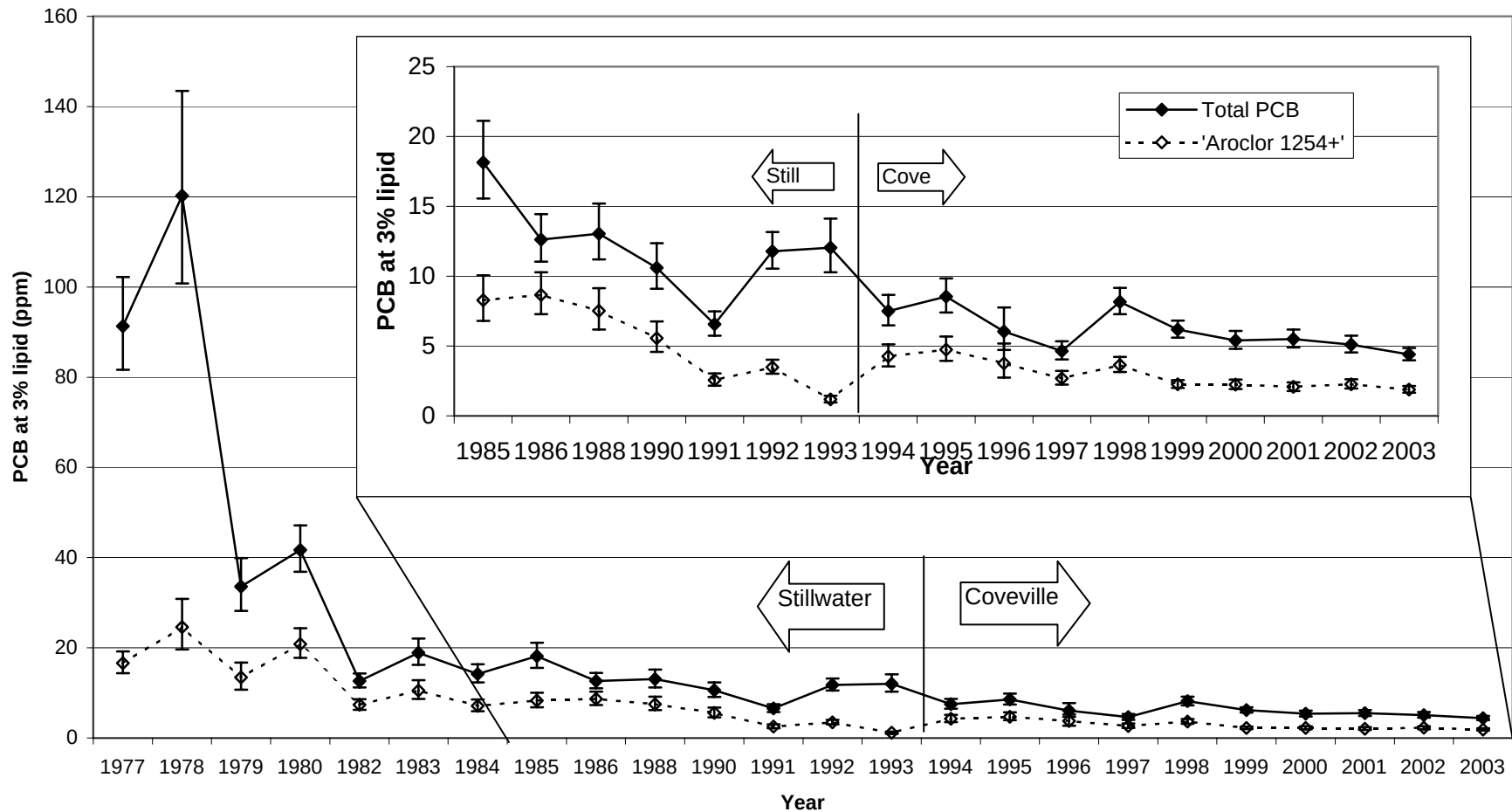
Figure 60. Trend in geometric PCB concentrations at 3% lipid for combined species ('Species Smash') collected at Stillwater Pool (River Mile 167/176). Results shown are least significant difference mean comparisons (95% confidence intervals) for total PCB - solid lines and higher chlorinated 'Aroclor 1254+' fraction - dashed lines.
