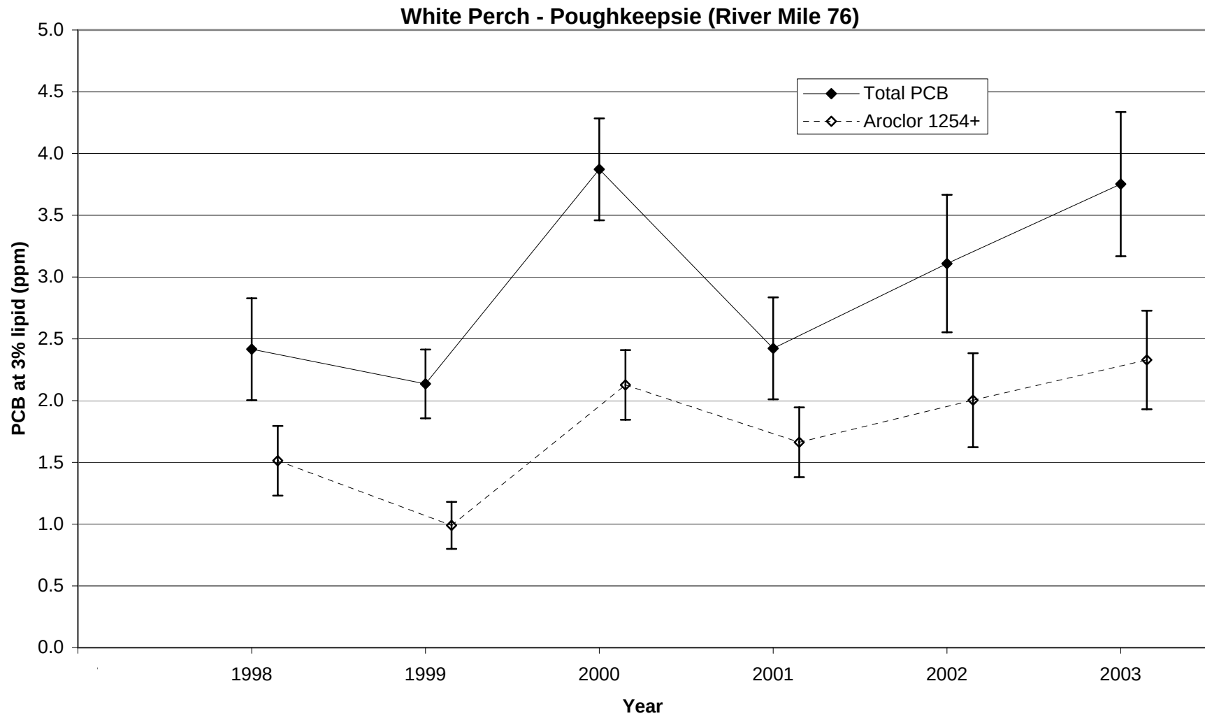
Figure 35. Trend in PCB concentrations at 3% lipid for white perch collected at Poughkeepsie in the lower Hudson River (River mile 76).. Results shown are Least Significant Difference mean comparisons (95% confidence intervals) for total PCB - solid lines, and higher chlorinated 'Aroclor 1254+' fraction - dashed lines.
