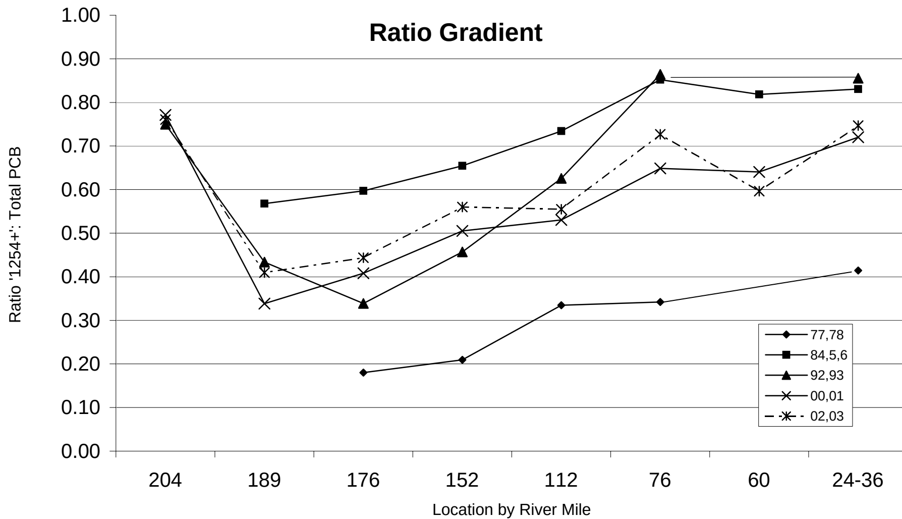
Figure 70. Spatial gradient of the ratio of 'Aroclor 1254+' to total PCB for a 'species smash' of fish collected in the spring during selected time periods from the Hudson River. Details of the accompanying ANOVA are provided in Table 53.
