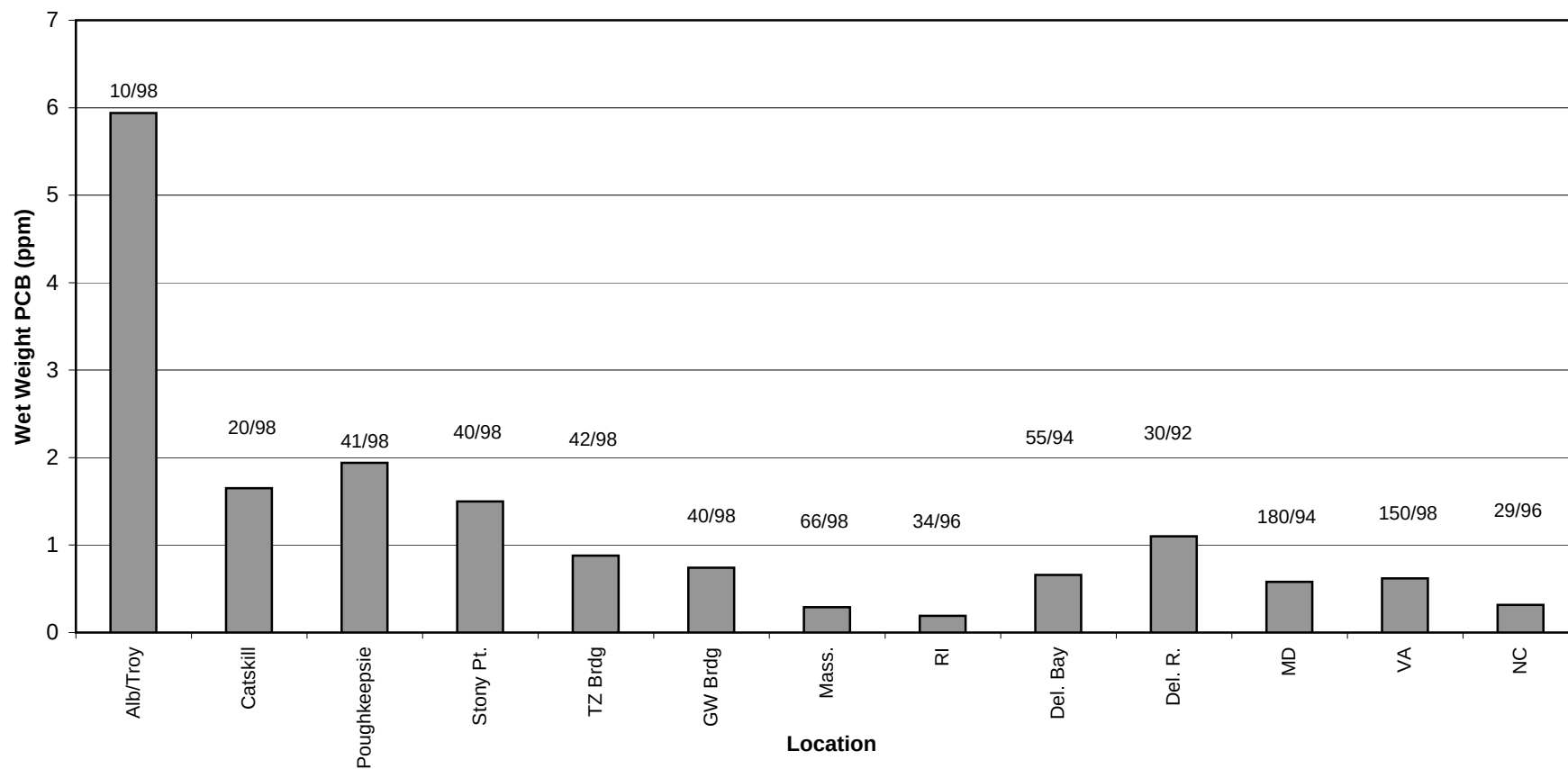
Figure 56. Average wet weight PCB concentrations in striped bass from other states in comparison to those collected in the spring of 1998 at several Hudson River locations. Hudson River locations are ordered upstream to downstream.
