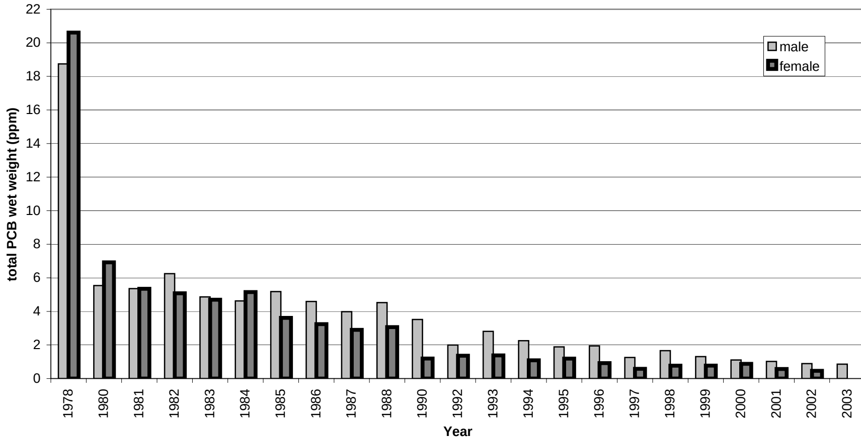
Figure 57B. Trend in wet weight total PCB concentrations in striped bass greater than 450 mm total length for each sex by year collected in the spring from Poughkeepsie to the George Washington Bridge which excludes one female in 2002 with a wet weight total PCB concentration of 52.98 ppm. Results of a one-way ANOVA are provided in Table 45A1.
