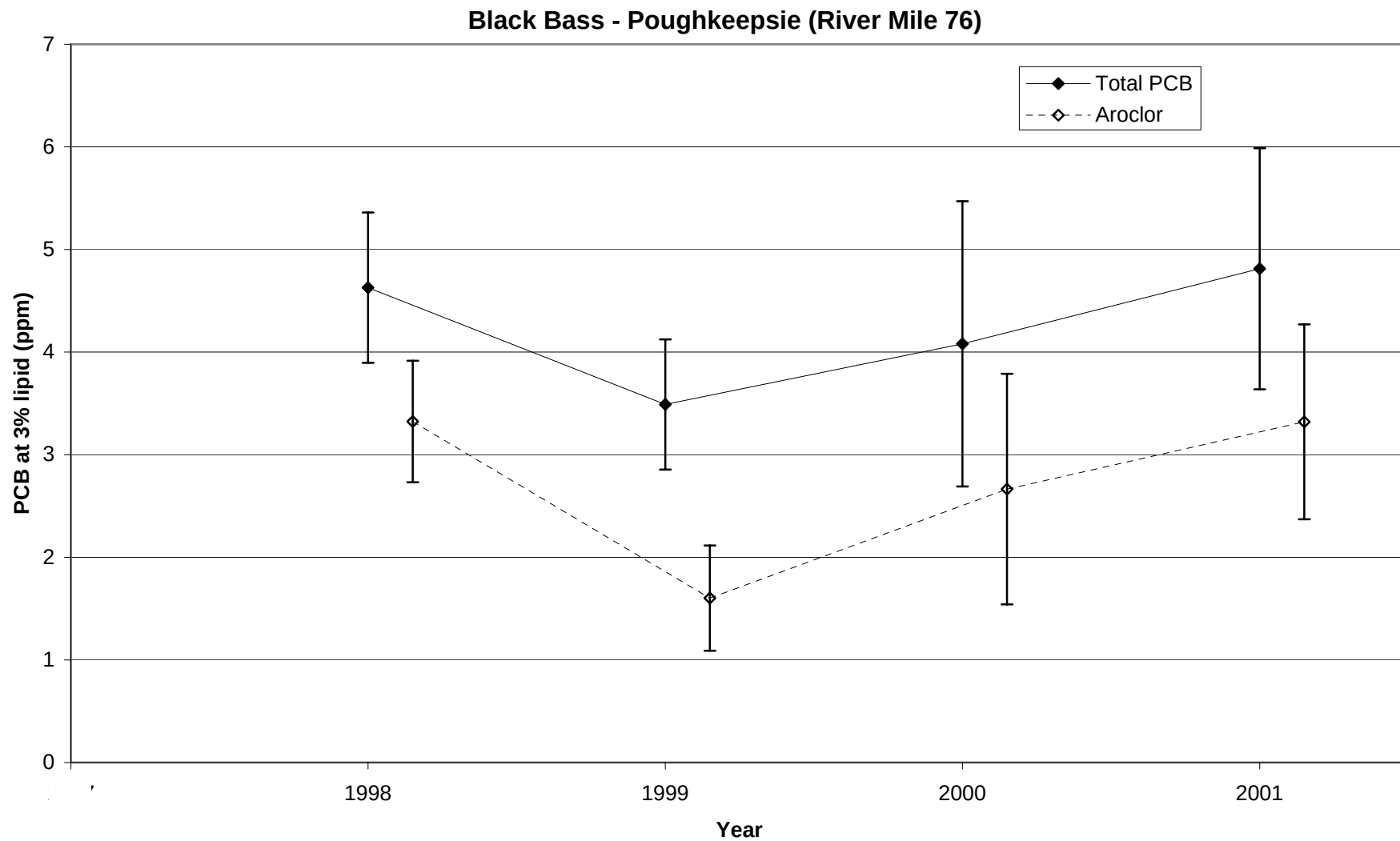
Figure 34. Trend in PCB concentrations at 3% lipid for black bass collected at Poughkeepsie in the lower Hudson River (River mile 76). Results shown are Least Significant Difference mean comparisons (95% confidence intervals) for total PCB - solid lines, and higher chlorinated 'Aroclor 1254+' fraction - dashed lines.
