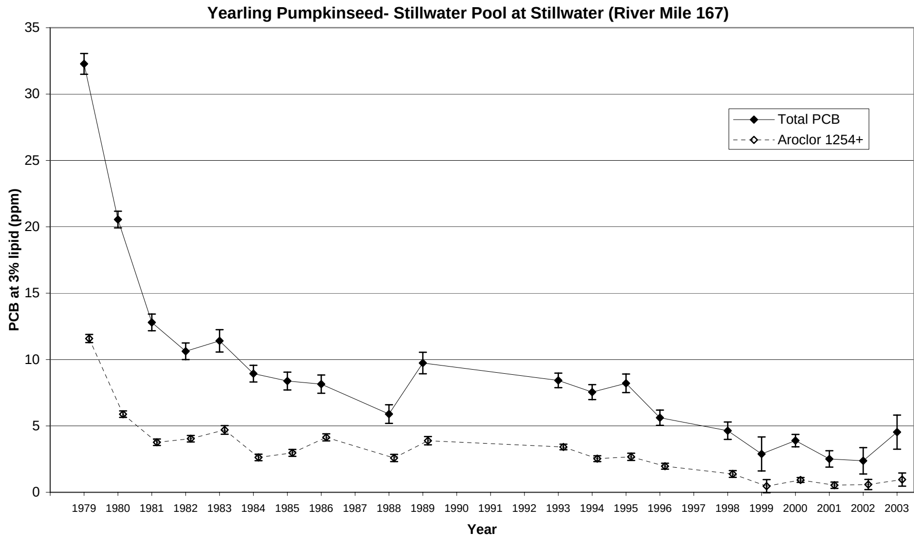
Figure 17. Trend in PCB concentrations at 3% lipid for yearling pumpkinseed collected at Stillwater in the Stillwater Pool (River mile 167). Results shown are Least Significant Difference mean comparisons (95% confidence intervals) for total PCB - solid lines, and higher chlorinated 'Aroclor 1254+' fraction - dashed lines.
