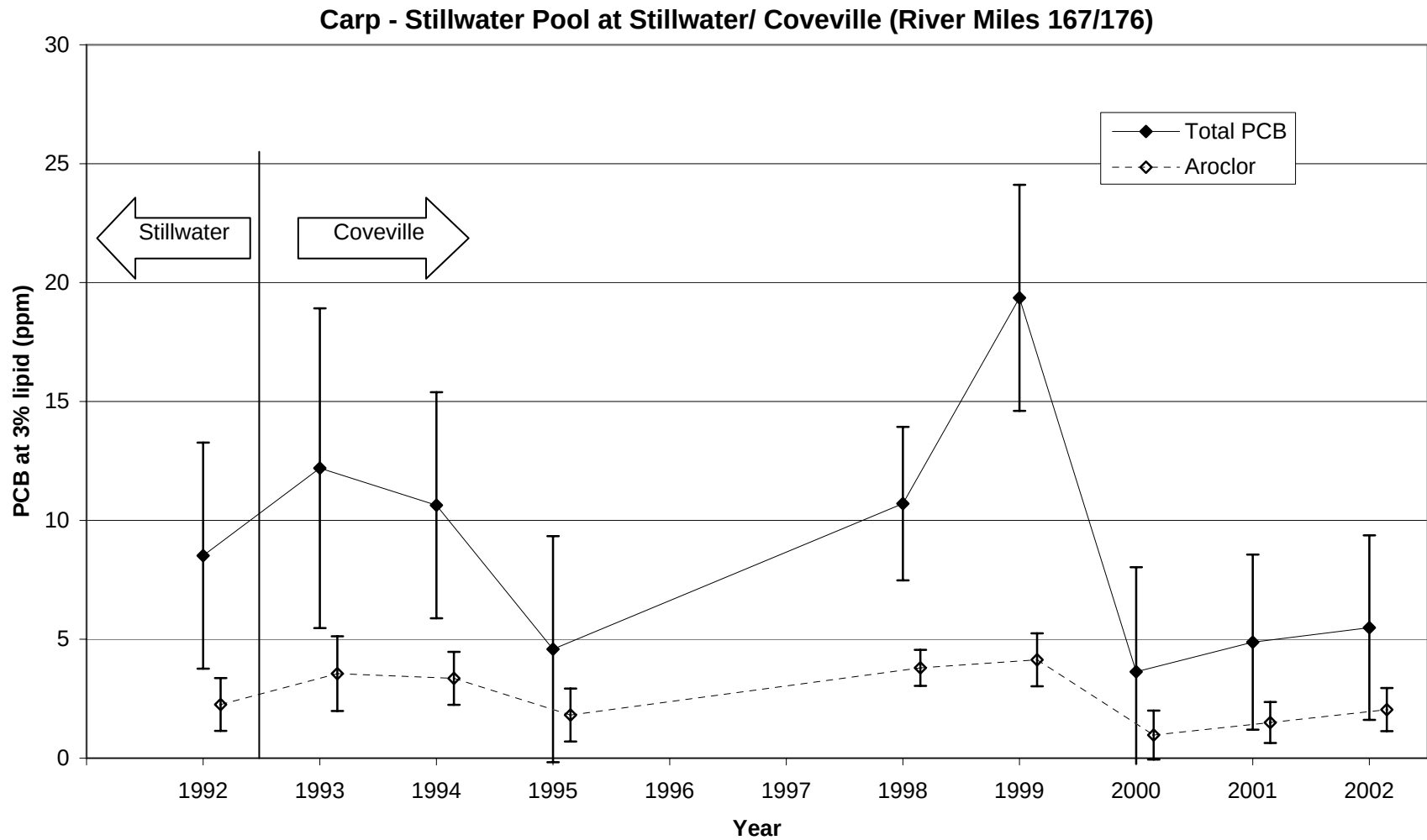
Figure 18. Trend in PCB concentrations at 3% lipid for carp collected at Stillwater/Coveville in the Stillwater Pool (River miles 167/176). Results shown are Least Significant Difference mean comparisons (95% confidence intervals) for total PCB - solid lines, and higher chlorinated 'Aroclor 1254+' fraction - dashed lines.
