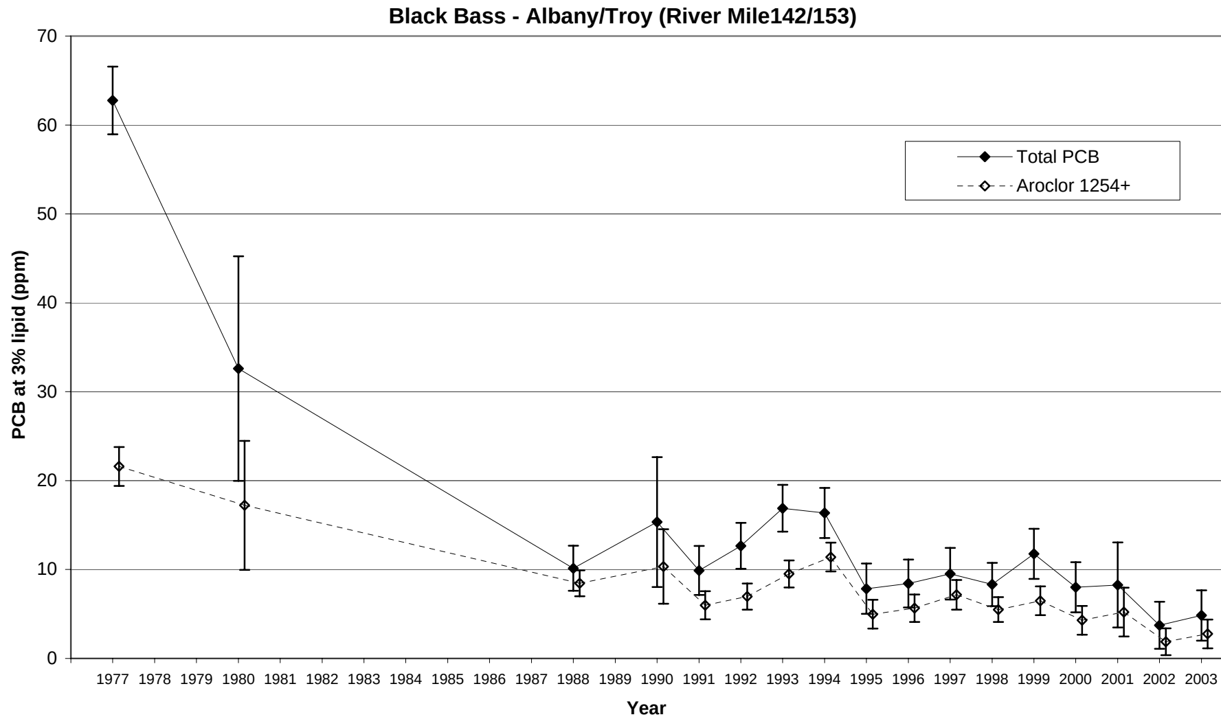
Figure 19B. Trend in PCB concentrations at 3% lipid for black bass collected at Albany/Troy in the lower Hudson River (River mile 142/153). Results shown are Least Significant Difference mean comparisons (95% confidence intervals) for total PCB - solid lines, and higher chlorinated 'Aroclor 1254+' fraction - dashed lines.
