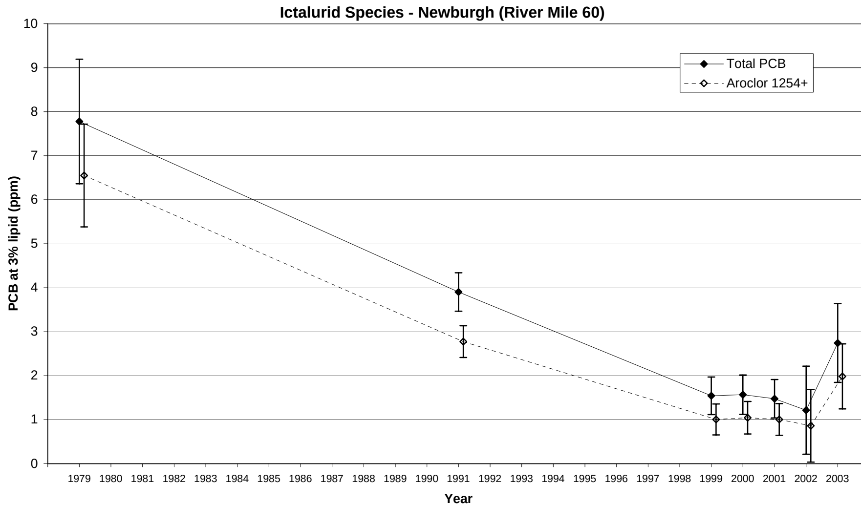
Figure 41. Trend in PCB concentrations at 3% lipid for Ictalurid species collected at Newburgh in the lower Hudson River (River mile 60). Results shown are Least Significant Difference mean comparisons (95% confidence intervals) for total PCB - solid lines, and higher chlorinated 'Aroclor 1254+' fraction - dashed lines.
