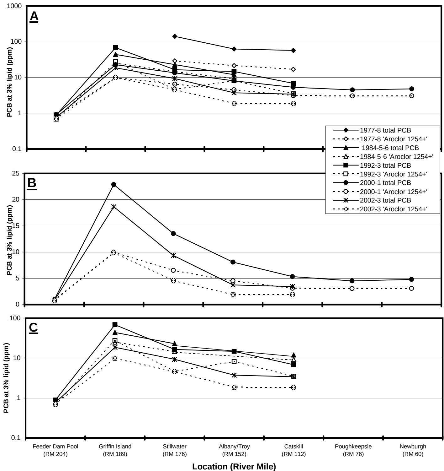
Figure 63. Spatial gradient of PCB concentrations for black bass collected during selected time periods from the Hudson River. Details of the accompanying ANOVA are provided in Table 46. Graphs are separated and presented on differing scales as noted to provide clarity. A). Gradient across all the selected years - logarithmic scale. B). Gradient for the most recent years (2000-01 vs. 2002-03) - arithmetic scale. C). Gradients for the middle years (1984,85,86 and 1992,93) vs. 2002-03 - logarithmic scale.
