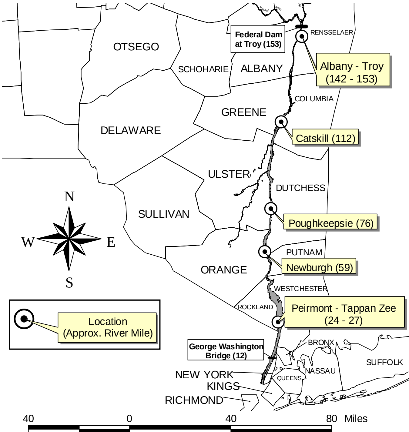
Figure 1B. Fish PCB trend analysis sampling locations in the lower Hudson River below the confluence with the Mohawk River and the Federal Dam at Troy. The Hudson River is a tidal estuary from the mouth to the Federal Dam. The upper estuary extends from Poughkeepsie to the Federal Dam. The lower estuary includes the reach from Battery Park in New York City to Poughkeepsie.
