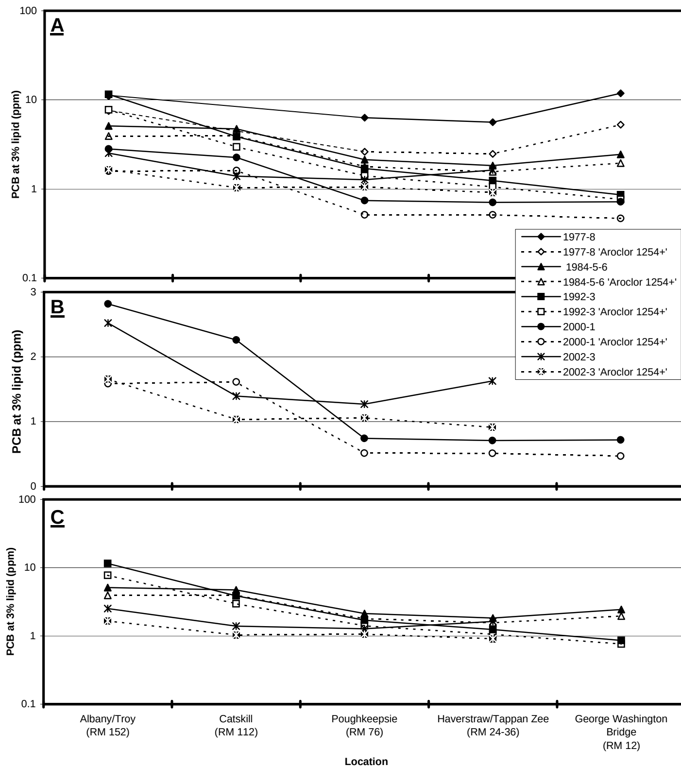
Figure 68. Spatial gradient of PCB concentrations for striped bass collected during selected time periods from the Hudson River. Details of the accompanying ANOVA are provided in Table 51. Graphs are separated and presented on differing scales as noted to provide clarity. A). Gradient across all the selected years. B). Gradient for the most recent years (2000-01 vs. 2002-03). C). Gradients for the middle years (1984,85,86 and 1992,93) vs. 2002-03.
