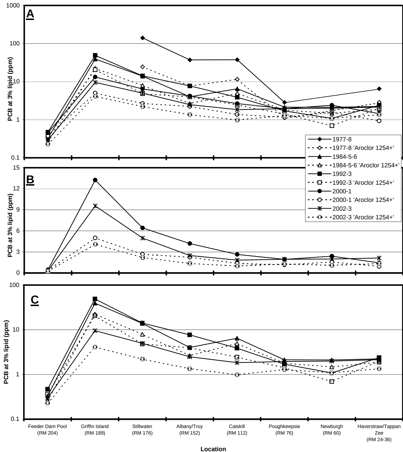
Figure 69. Spatial gradient of PCB concentrations for a 'species smash' collected during selected time periods from the Hudson River. Details of the accompanying ANOVA are provided in Table 52. Graphs are separated and presented on differing scales as noted to provide clarity. A). Gradient across all the selected years. B). Gradient for the most recent years (2000-01 vs. 2002-03). C). Gradients for the middle years (1984,85,86 and 1992,93) vs. 2002-03.
