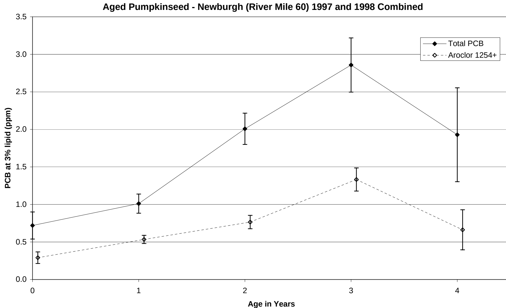
Figure 44. Comparison of PCB concentrations at 3% lipid by age for pumpkinseed collected at Newburgh in the lower Hudson River (River mile 60) for 1997 and 1998 combined. Results shown are Least Significant Difference mean comparisons (95% confidence intervals) for total PCB - solid lines, and the higher chlorinated 'Aroclor 1254+' fraction - dashed lines.
