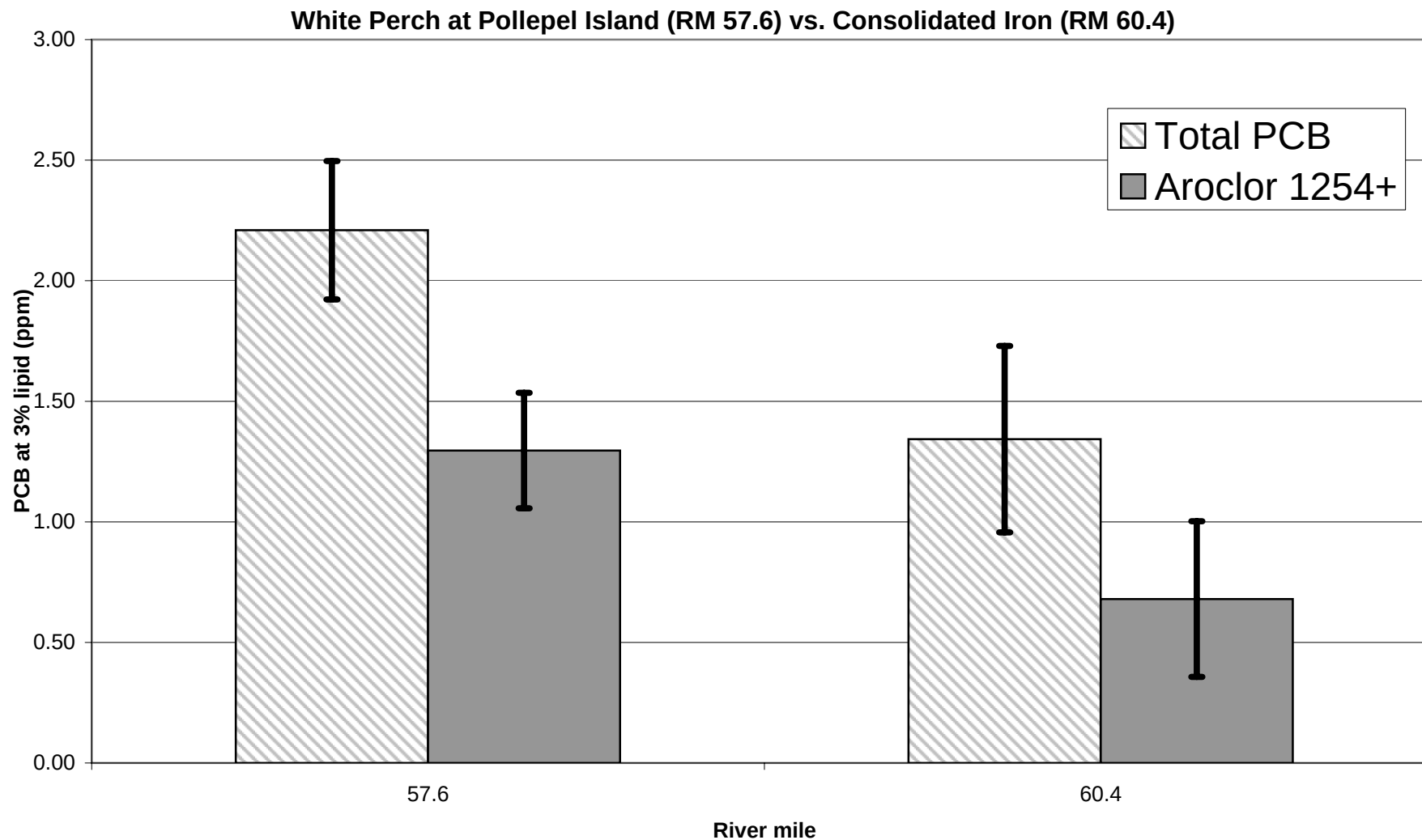
Figure 46. Comparison of PCB concentrations at 3% lipid for white perch collected at two locations near Newburgh in the lower Hudson River (River mile 60). Results shown are Least Significant Difference mean comparisons (95% confidence intervals) for total PCB - diagonal lines, and the higher chlorinated 'Aroclor 1254+' fraction - solid fill.
