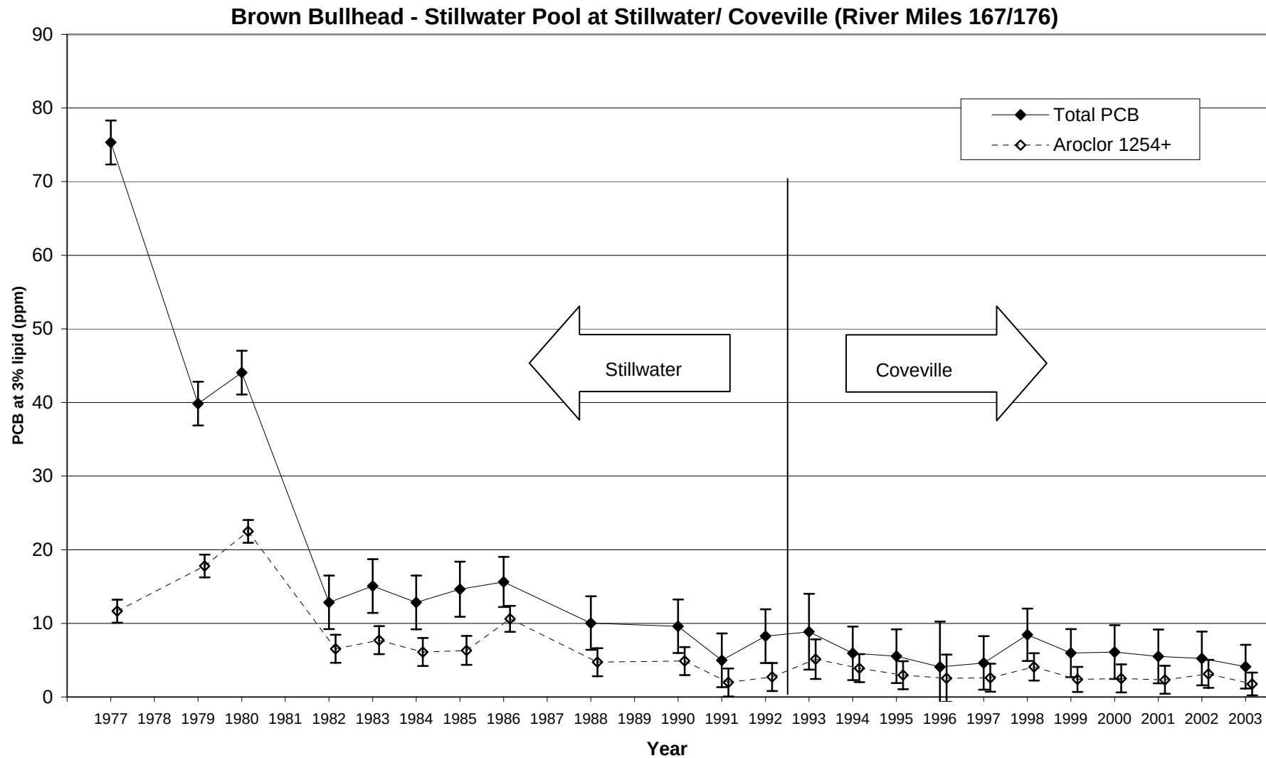
Figure 14. Trend in PCB concentrations at 3% lipid for brown bullhead collected at Stillwater/Coveville in the Stillwater Pool (River miles 167/176). Results shown are Least Significant Difference mean comparisons (95% confidence intervals) for total PCB - solid lines, and higher chlorinated 'Aroclor 1254+' fraction - dashed lines.
