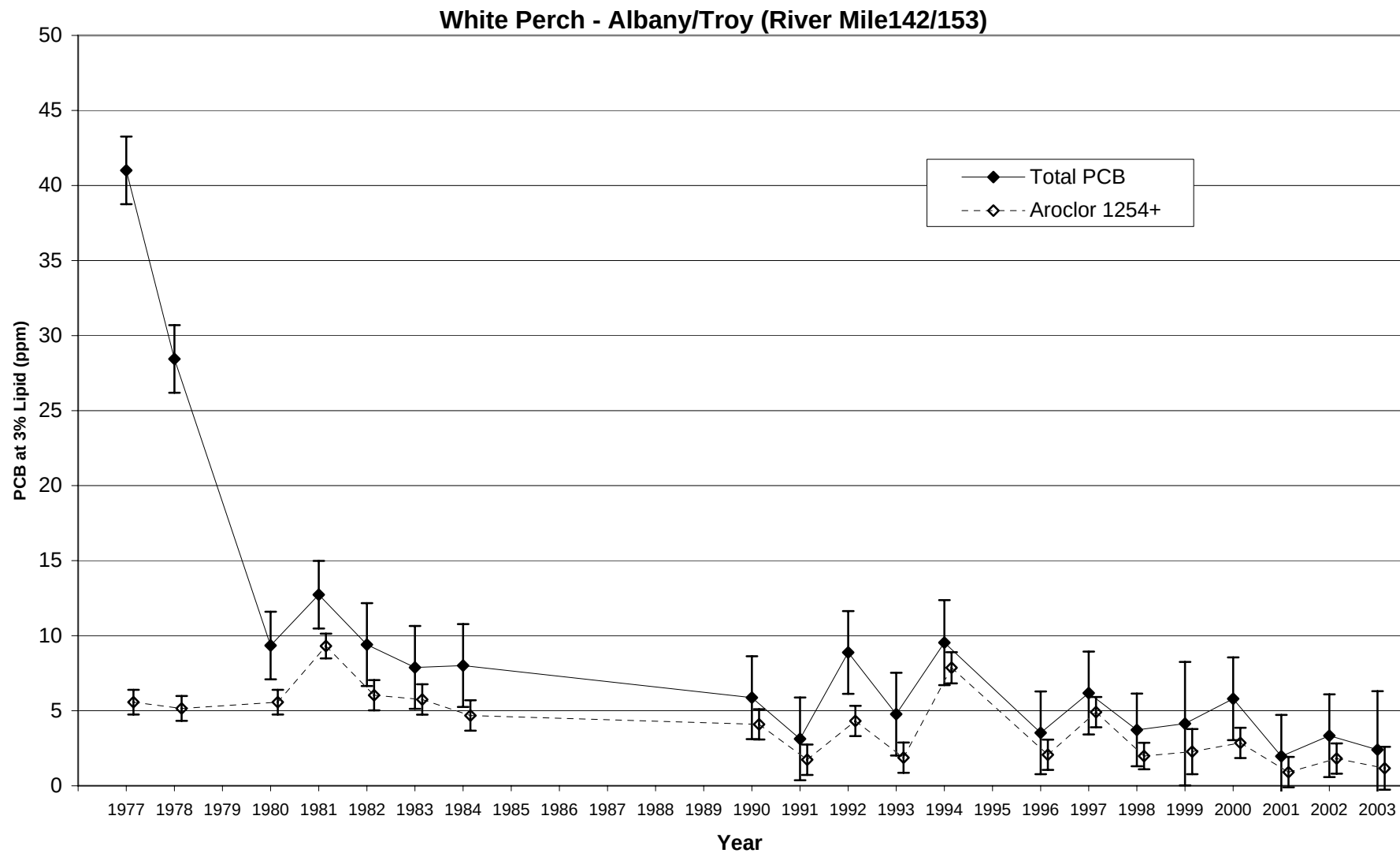
Figure 21. Trend in PCB concentrations at 3% lipid for white perch collected at Albany/Troy in the lower Hudson River (River mile 142/153). Results shown are Least Significant Difference mean comparisons (95% confidence intervals) for total PCB - solid lines, and higher chlorinated 'Aroclor 1254+' fraction - dashed lines.
