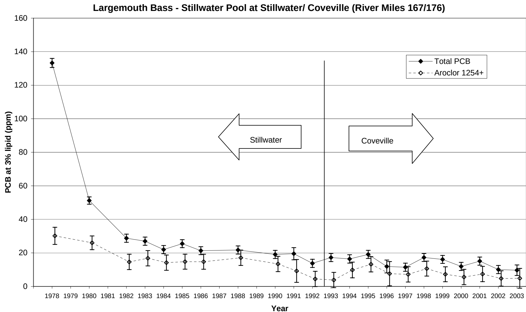
Figure 15. Trend in PCB concentrations at 3% lipid for largemouth bass collected at Stillwater/Coveville in the Stillwater Pool (River miles 167/176). Results shown are Least Significant Difference mean comparisons (95% confidence intervals) for total PCB - solid lines, and higher chlorinated 'Aroclor 1254+' fraction - dashed lines.
