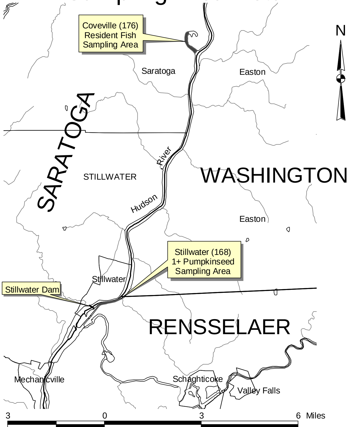
Figure 13 Fish PCB trend analysis sampling locations in the Stillwater Pool of the Hudson River at Stillwater (River mile 168 and Coveville (River mile 176).
