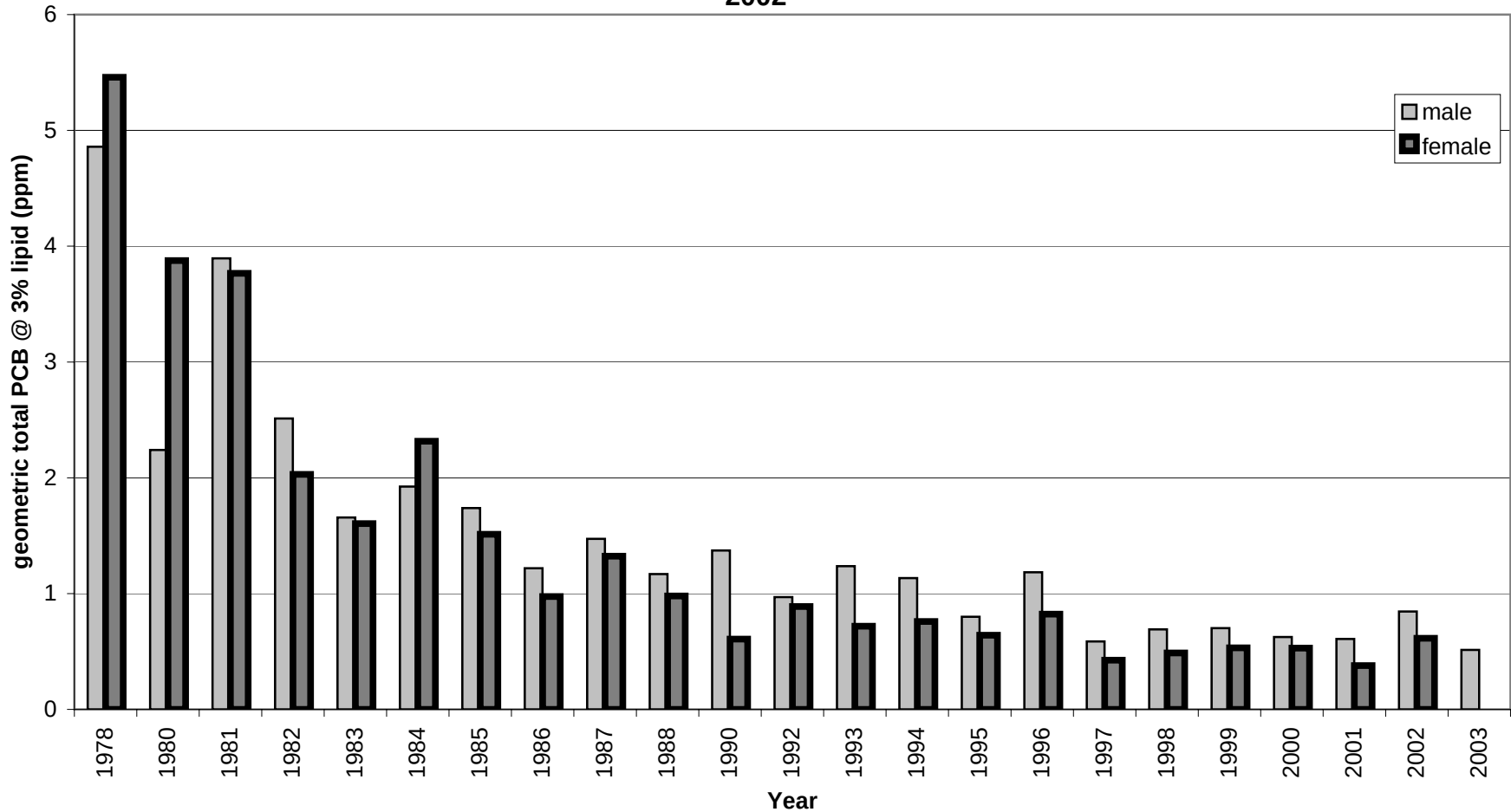
Figure 57D. Geometric trend in total PCB (ppm) log10-transformed at 3 % lipid for striped bass greater than 450 mm total length for each sex by year collected in the spring from Poughkeepsie to the George Washington Bridge which excludes one female in 2002 with a wet weight total PCB concentration of 52.98 ppm. Results of a one-way ANOVA are provided in Table 45A2.
