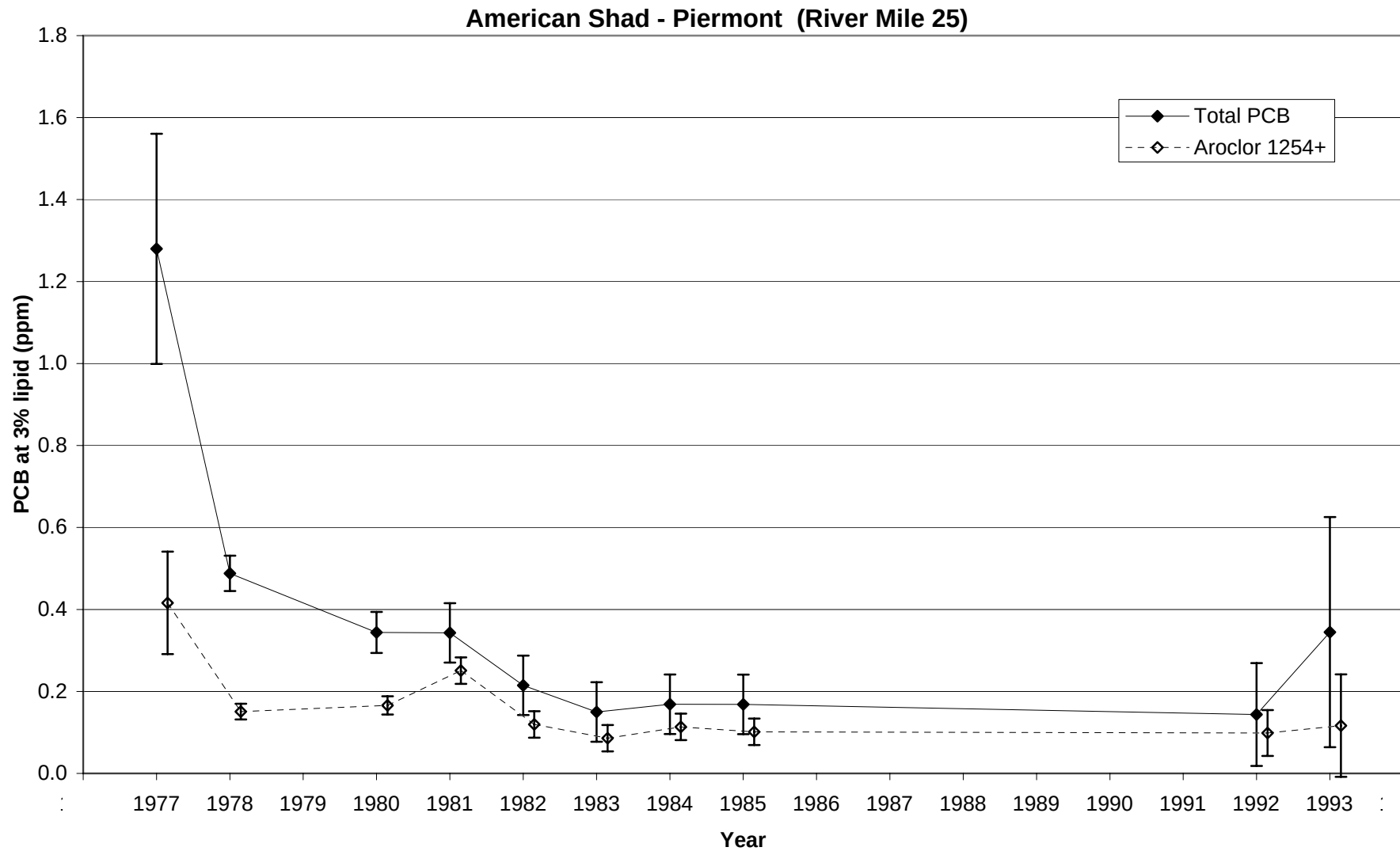
Figure 51. Trend in PCB concentrations at 3% lipid for American shad collected near Piermont in the lower Hudson River (River mile 25). Results shown are Least Significant Difference mean comparisons (95% confidence intervals) for total PCB - solid lines, and higher chlorinated 'Aroclor 1254+' fraction - dashed lines.
