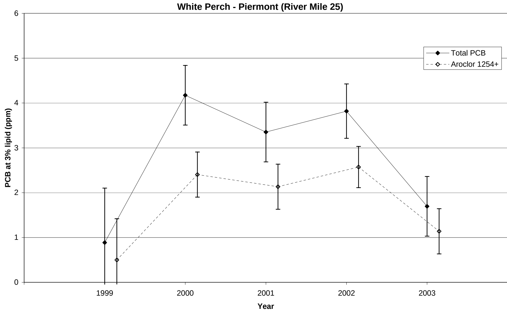
Figure 48. Trend in PCB concentrations at 3% lipid for white perch collected near Piermont in the lower Hudson River (River mile 25). Results shown are Least Significant Difference mean comparisons (95% confidence intervals) for total PCB - solid lines, and higher chlorinated 'Aroclor 1254+' fraction - dashed lines.
