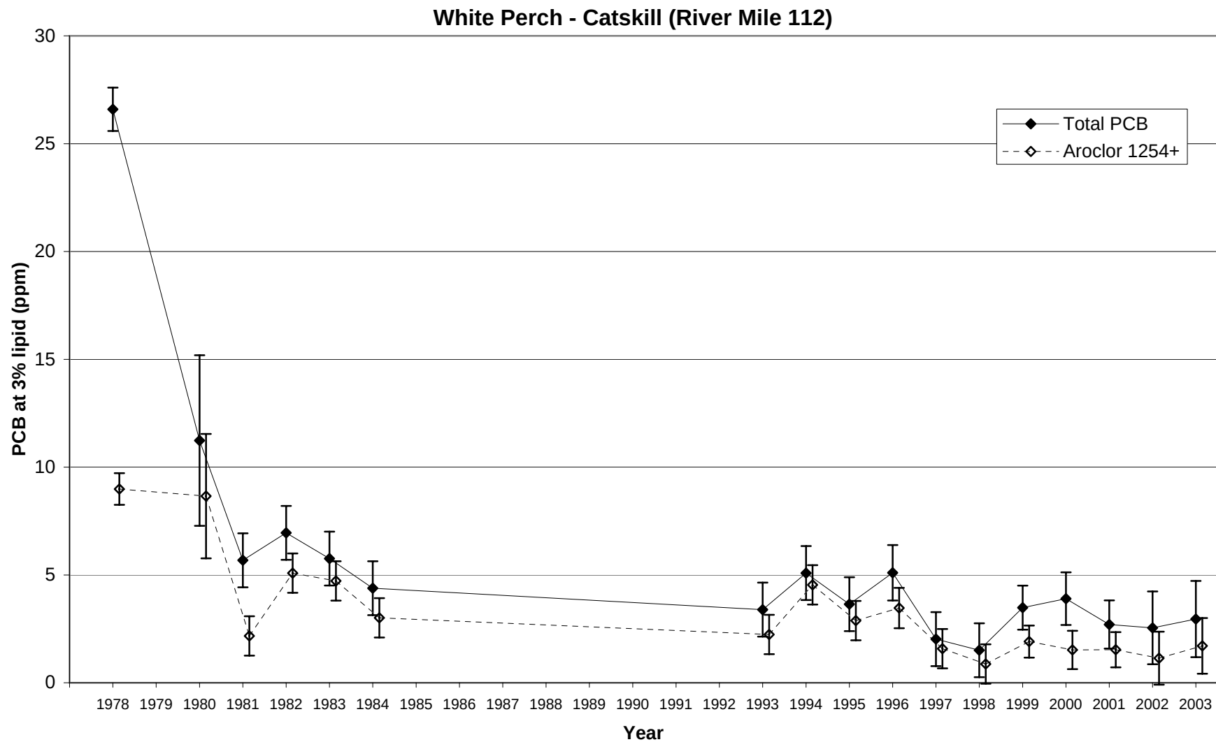
Figure 29B. Trend in PCB concentrations at 3% lipid for white perch collected at Catskill in the lower Hudson River (River mile 112). Results shown are Least Significant Difference mean comparisons (95% confidence intervals) for total PCB - solid lines, and higher chlorinated 'Aroclor 1254+' fraction - dashed lines.
