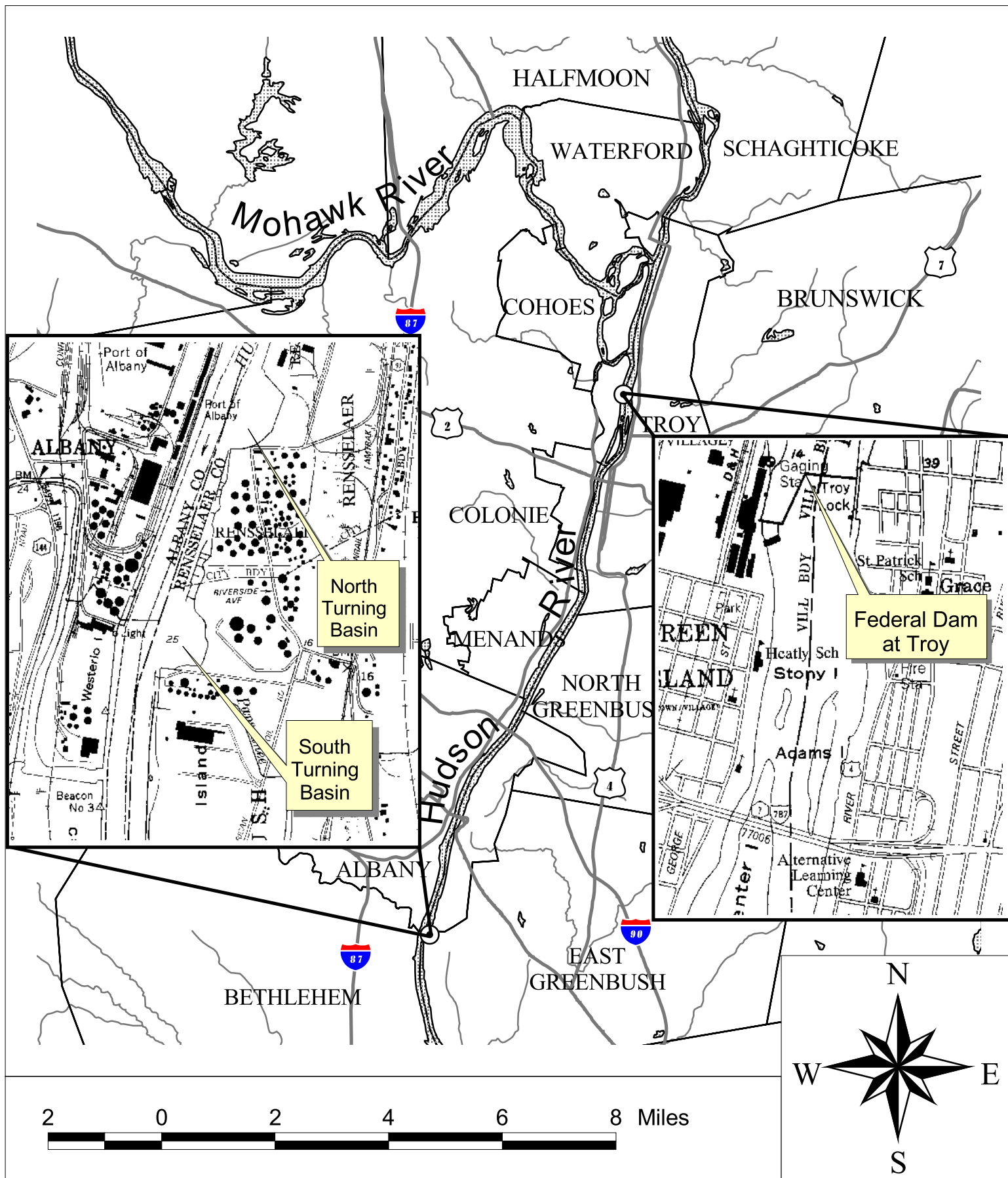
Figure 19A. Sampling locations in the vicinity of Albany and Troy. Inset maps show greater detail of the areas around the Federal Dam at Troy and the South Turning Basin at Albany.
