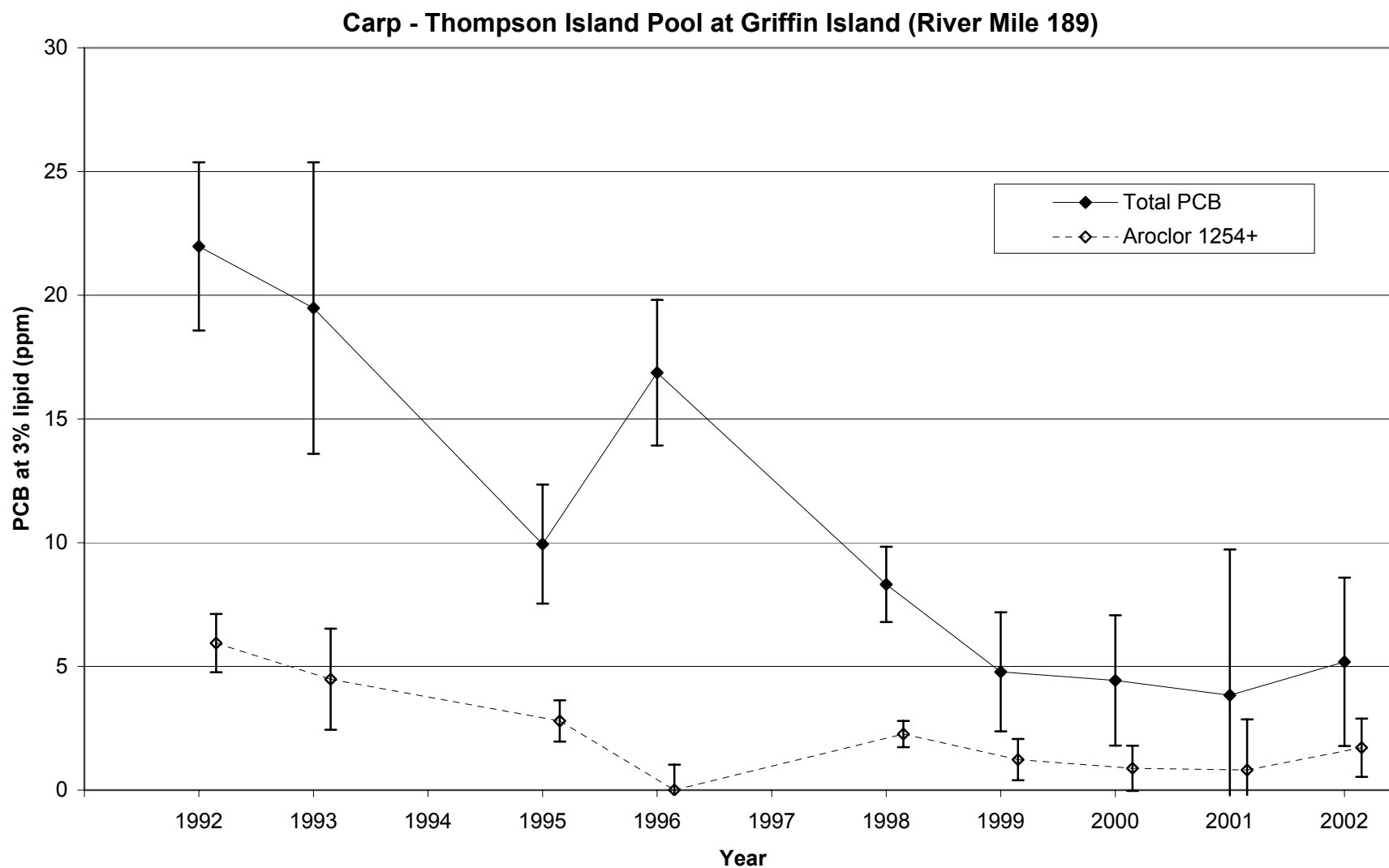
Figure 12. Trend in PCB concentrations at 3% lipid for carp collected at Griffin Island in the Thompson Island Pool (River mile 189). Results shown are Least Significant Difference mean comparisons (95% confidence intervals) for total PCB - solid lines, and higher chlorinated 'Aroclor 1254+' fraction - dashed lines.
