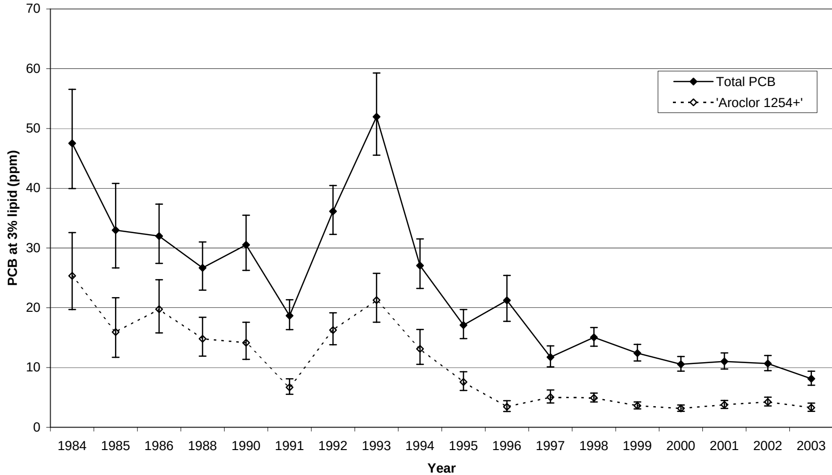
Figure 59. Trend in geometric PCB concentrations at 3% lipid for combined species ('Species Smash') collected at Griffin Island (River Mile 189). Results shown are least significant difference mean comparisons (95% confidence intervals) for total PCB - solid lines and higher chlorinated 'Aroclor 1254+' fraction - dashed lines.
