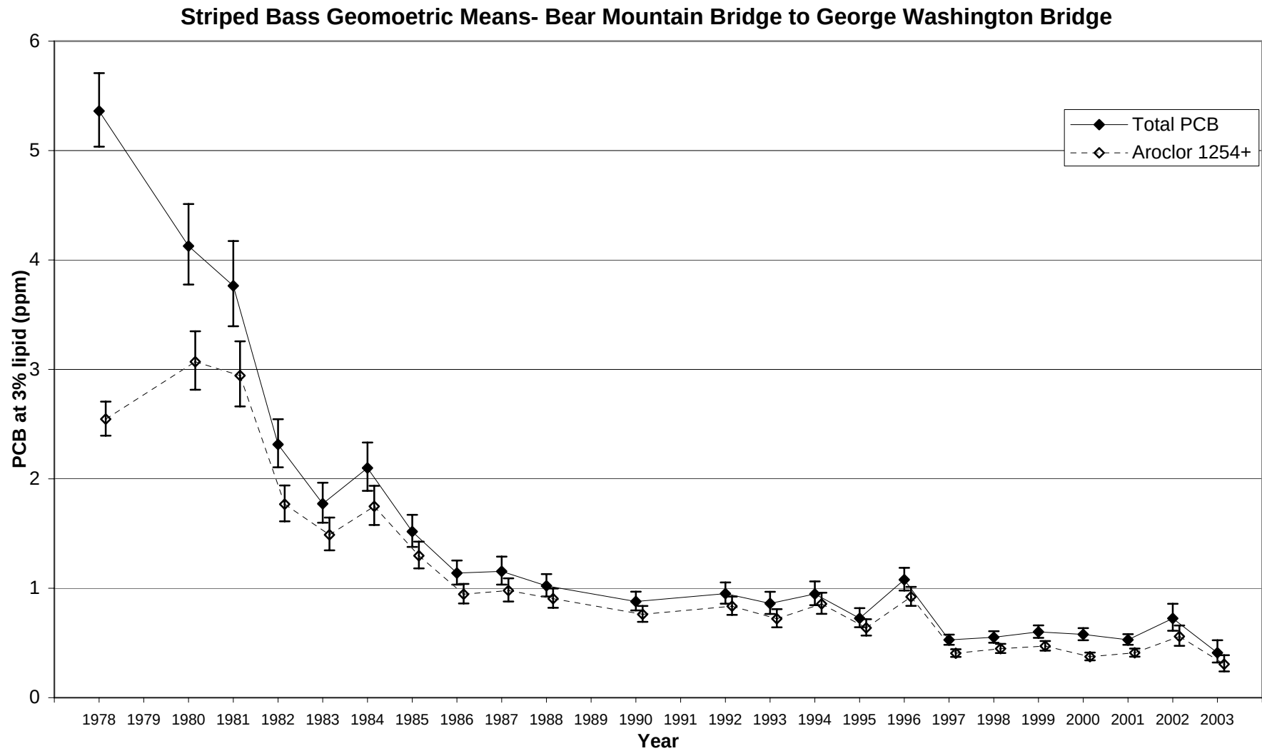
Figure 55. Trend in geometric PCB concentrations at 3% lipid for striped bass collected from the Bear Mountain Bridge to the George Washington Bridge in the lower Hudson River (River miles 47-12). Results shown are Least Significant Difference mean comparisons (95% confidence intervals) for total PCB - solid lines, and the higher chlorinated 'Aroclor 1254+' fraction - dashed lines.
