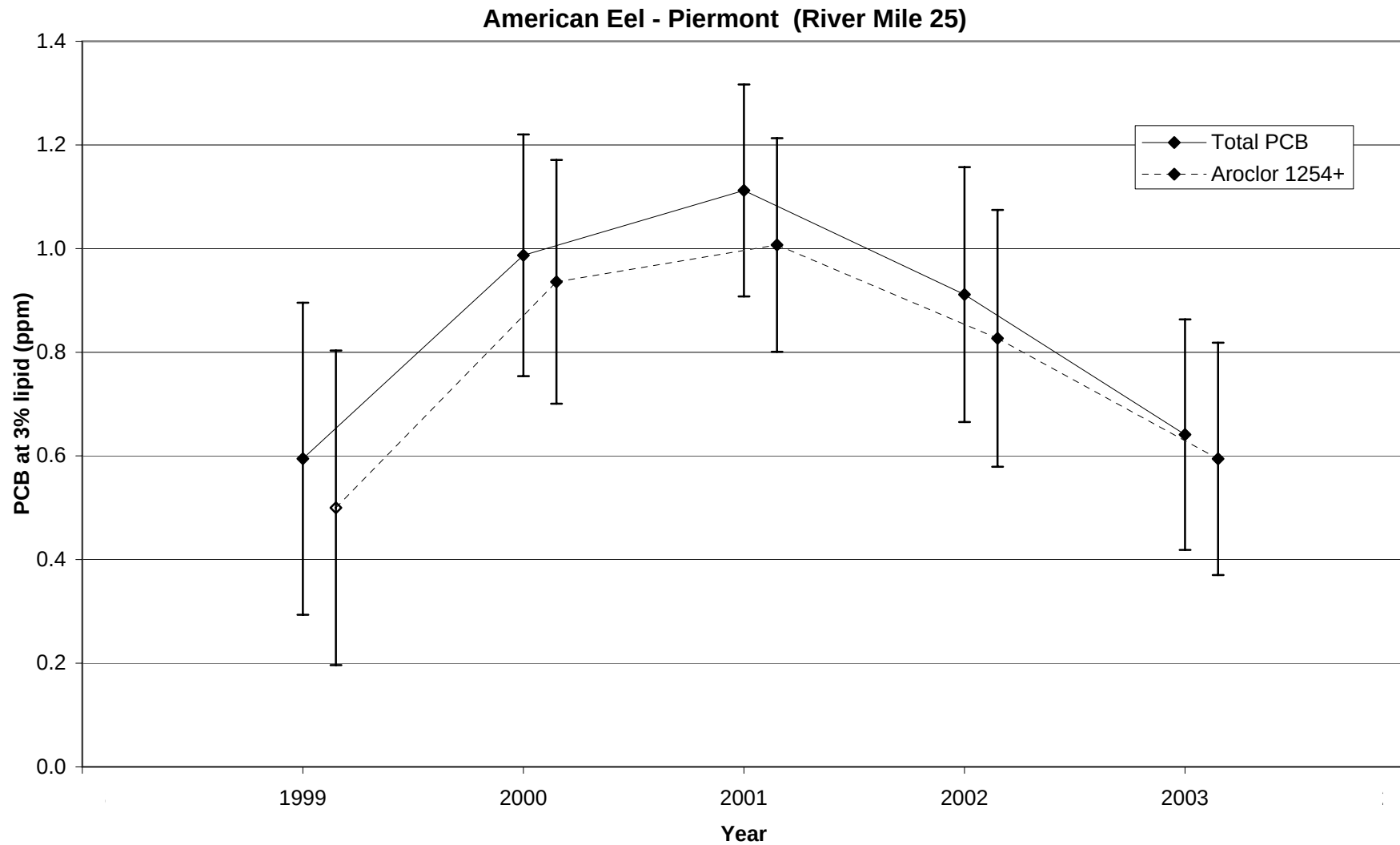
Figure 49. Trend in PCB concentrations at 3% lipid for American eel collected near Piermont in the lower Hudson River (River mile 25). Results shown are Least Significant Difference mean comparisons (95% confidence intervals) for total PCB - solid lines, and higher chlorinated 'Aroclor 1254+' fraction - dashed lines.
