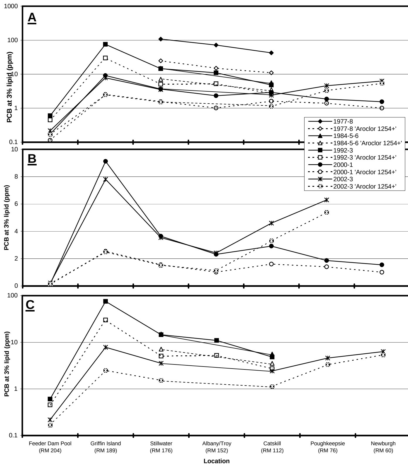
Figure 65. Spatial gradient of PCB concentrations for yellow perch collected during selected time periods from the Hudson River. Details of the accompanying ANOVA are provided in Table 48. Graphs are separated and presented on differing scales as noted to provide clarity. A). Gradient across all the selected years. B). Gradient for the most recent years (2000-01 vs. 2002-03). C). Gradients for the middle years (1984,85,86 and 1992,93) vs. 2002-03.
