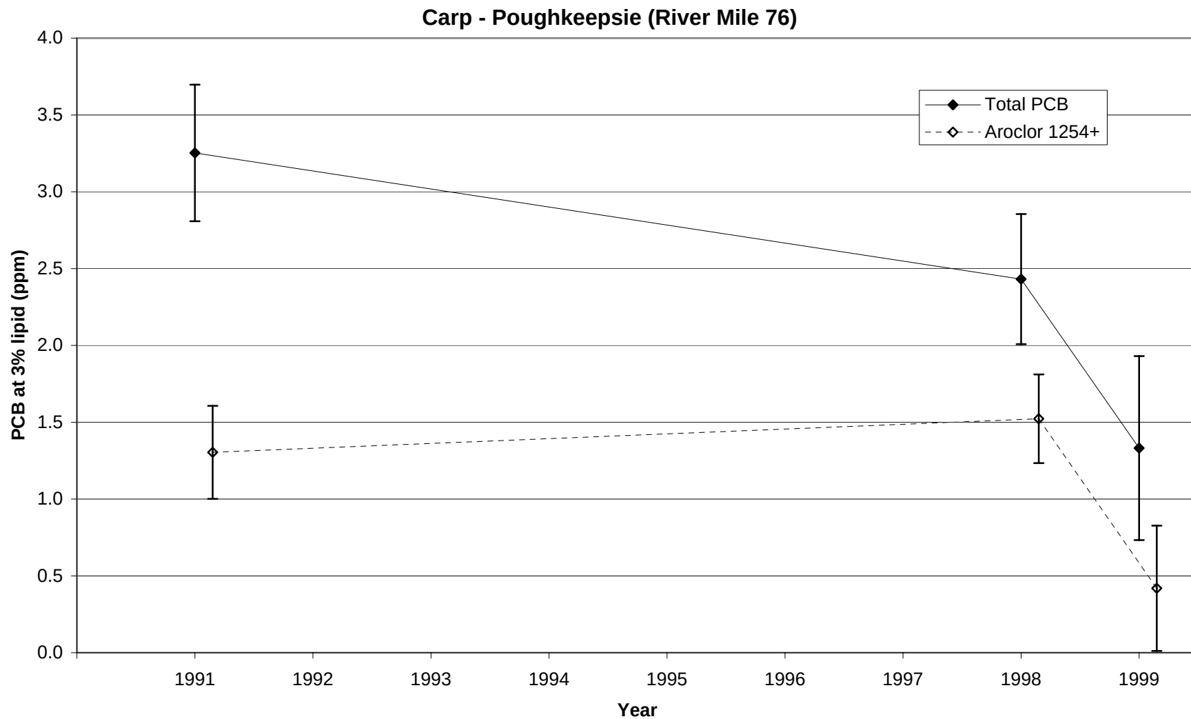
Figure 33. Trend in PCB concentrations at 3% lipid for carp collected at Poughkeepsie in the lower Hudson River (River mile 76). Results shown are Least Significant Difference mean comparisons (95% confidence intervals) for total PCB - solid lines, and higher chlorinated 'Aroclor 1254+' fraction - dashed lines.
