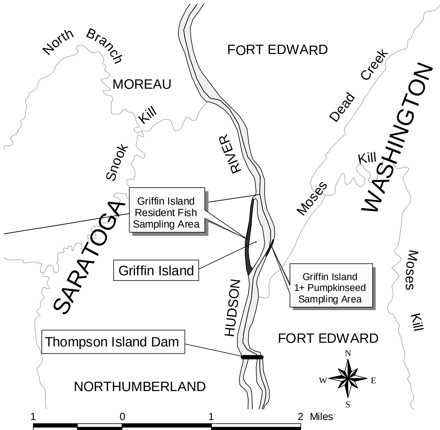
Figure 7. Fish PCB trend analysis sampling locations in the Thompson Island Pool of the Hudson River near Griffin Island (River mile 189).
