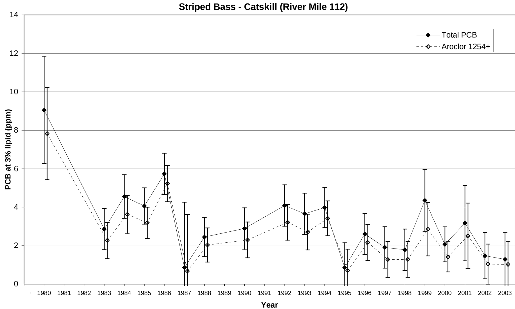
Figure 30. Trend in lipid Based PCB concentrations at 3% lipid for striped bass collected at Catskill in the lower Hudson River (River mile 112). Results shown are Least Significant Difference mean comparisons (95% confidence intervals) for total PCB - solid lines, and higher chlorinated 'Aroclor 1254+' fraction - dashed lines.
