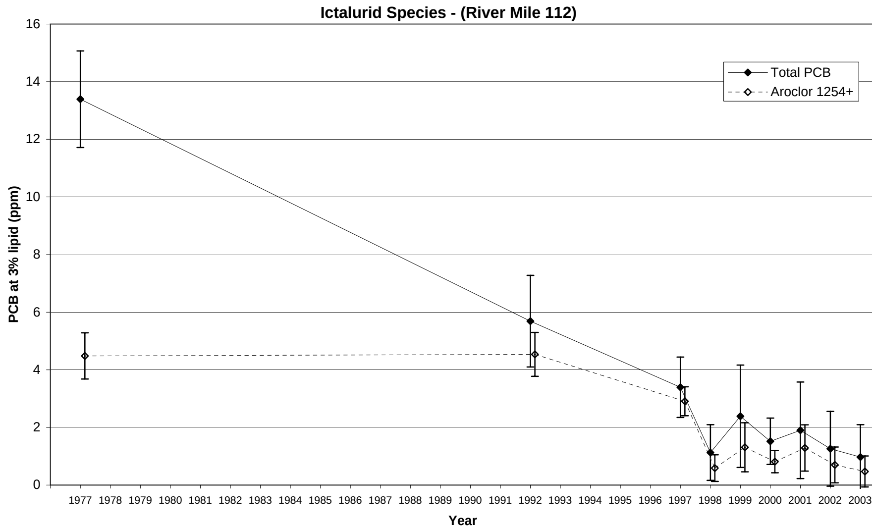
Figure 27. Trend in PCB concentrations at 3% lipid for Ictalurid species collected at Catskill in the lower Hudson River (River mile 112). Results shown are Least Significant Difference mean comparisons (95% confidence intervals) for total PCB - solid lines, and higher chlorinated 'Aroclor 1254+' fraction - dashed lines.
