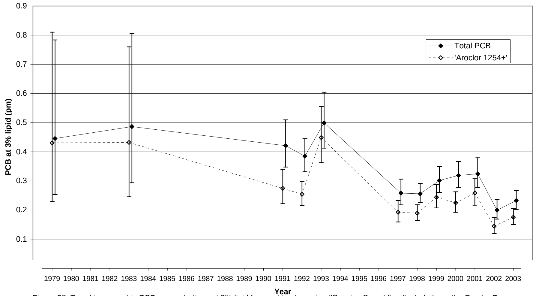
Figure 58. Trend in geometric PCB concentrations at 3% lipid for combined species ('Species Smash') collected above the Feeder Dam (River Mile 204). Results shown are least significant difference mean comparisons (95% confidence intervals) for total PCB - solid lines and higher chlorinated 'Aroclor 1254+' fraction - dashed lines.
