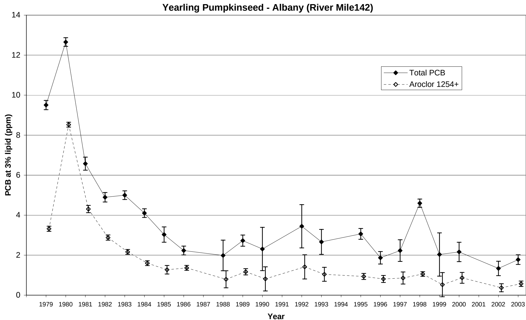
Figure 23. Trend in PCB concentrations at 3% lipid for yearling pumpkinseed collected at Albany in the lower Hudson River (River mile 142). Results shown are Least Significant Difference mean comparisons (95% confidence intervals) for total PCB - solid lines, and higher chlorinated 'Aroclor 1254+' fraction - dashed lines.
