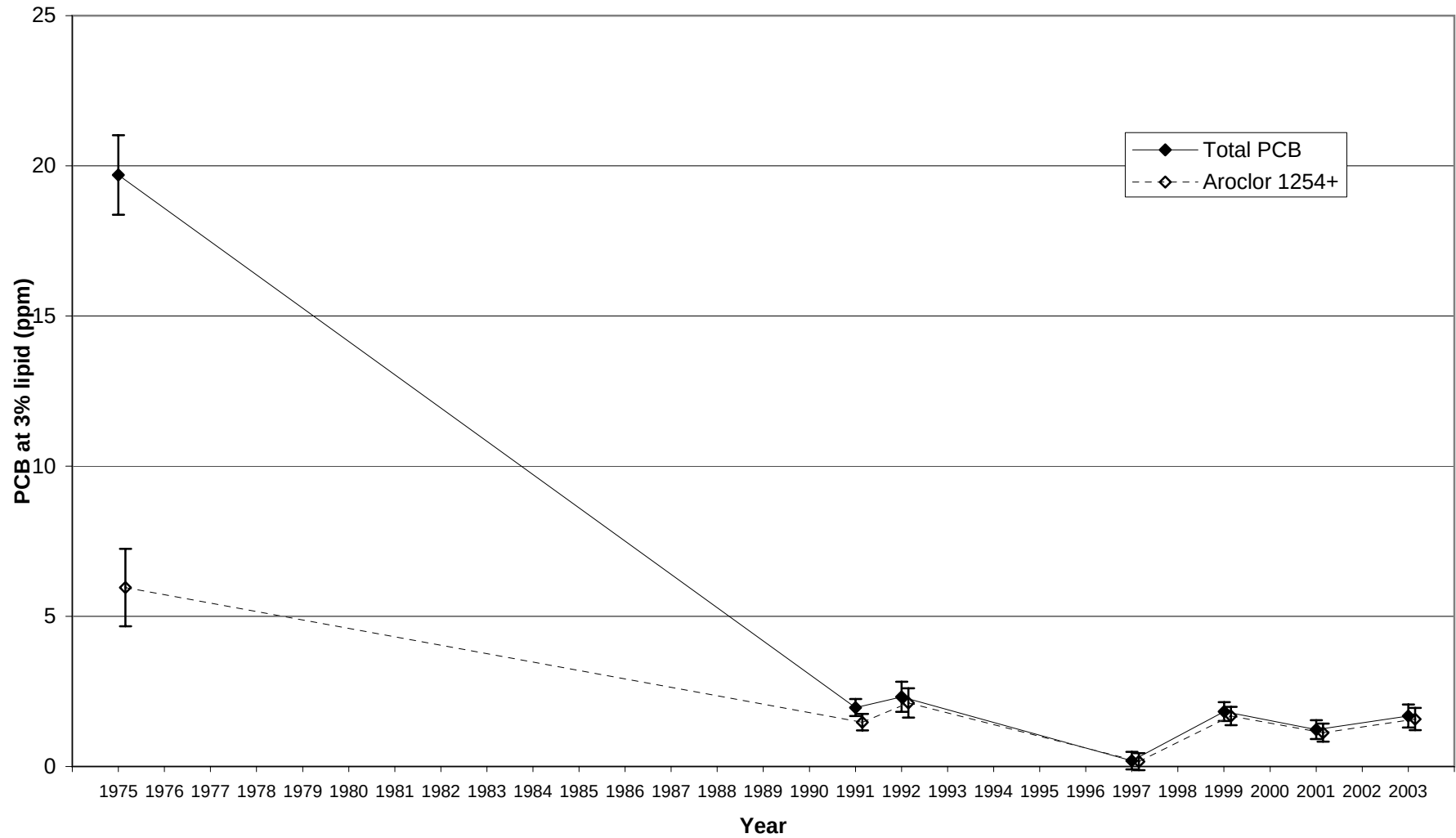
Figure 40. Trend in PCB concentrations at 3% lipid for American eel collected at Newburgh in the lower Hudson River (River mile 60). Results shown are Least Significant Difference mean comparisons (95% confidence intervals) for total PCB - solid lines, and higher chlorinated 'Aroclor 1254+' fraction - dashed lines.
