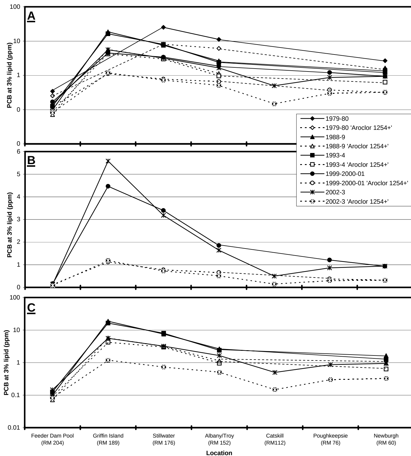
Figure 67. Spatial gradient of PCB concentrations for yearling pumpkinseed collected during selected time periods from the Hudson River. Details of the accompanying ANOVA are provided in Table 50. Graphs are separated and presented on differing scales as noted to provide clarity. A). Gradient across all the selected years. B). Gradient for the most recent years (2000-01 vs. 2002-03). C). Gradients for the middle years (1984,85,86 and 1992,93) vs. 2002-03.
