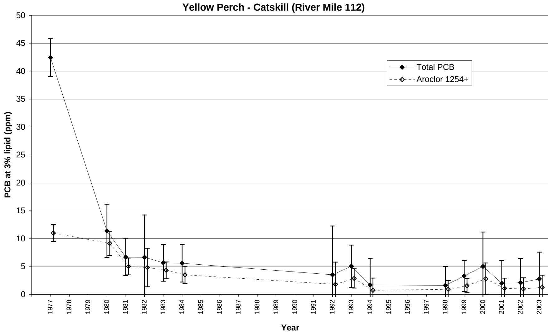
Figure 28. Trend in PCB concentrations at 3% lipid for yellow perch collected at Catskill in the lower Hudson River (River mile 112). Results shown are Least Significant Difference mean comparisons (95% confidence intervals) for total PCB - solid lines, and higher chlorinated 'Aroclor 1254+' fraction - dashed lines.
