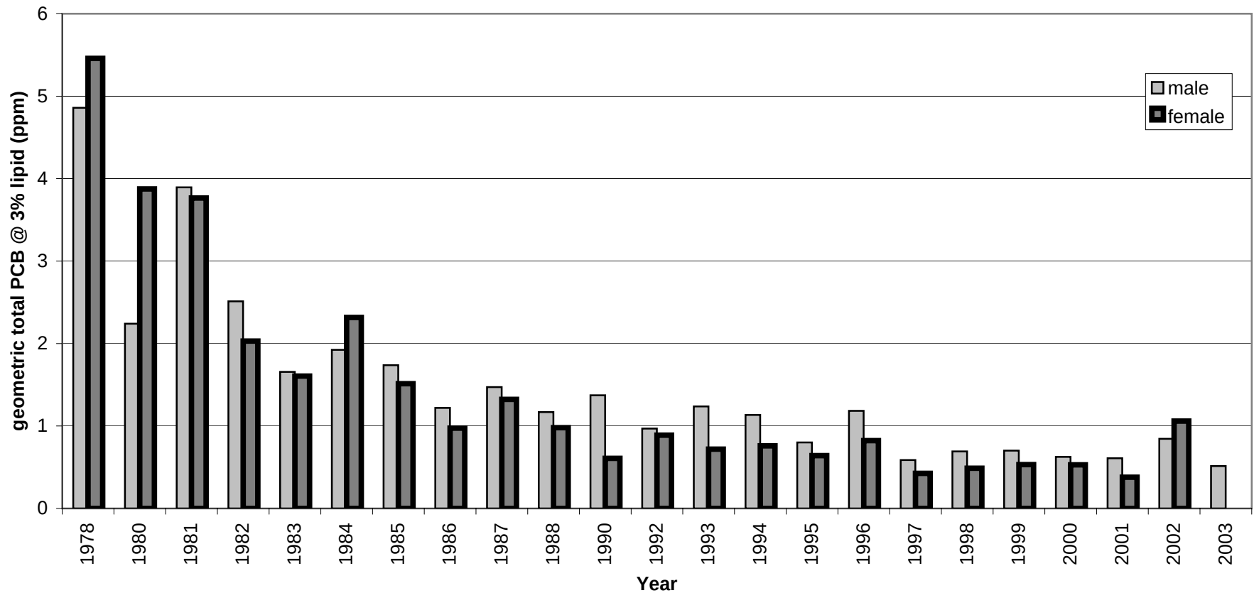
Figure 57C. Geometric trend in total PCB (ppm) log10-transformed at 3 % lipid for striped bass greater than 450 mm total length for each sex by year collected in the spring from Poughkeepsie to the George Washington Bridge which includes one female in 2002 with a wet weight total PCB concentration of 52.98 ppm. Results of a one-way ANOVA are provided in Table 45A2.
