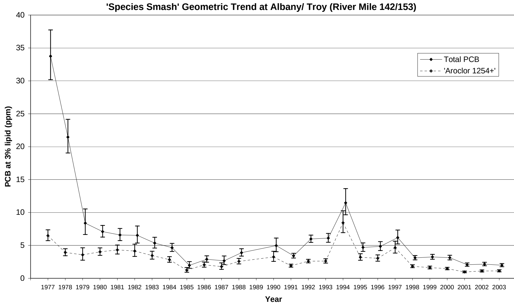
Figure 61. Trend in geometric PCB concentrations at 3% lipid for combined species ('Species Smash') collected at Albany/ Troy (River Mile 142/153). Results shown are least significant difference mean comparisons (95% confidence intervals) for total PCB - solid lines and higher chlorinated 'Aroclor 1254+' fraction - dashed lines.
