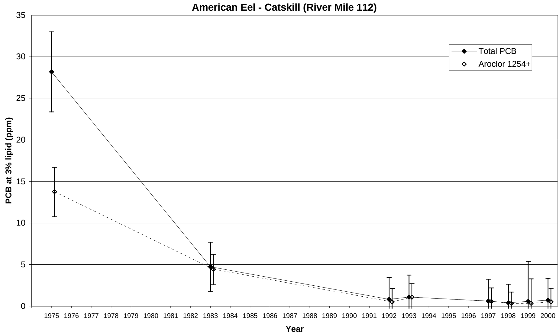
Figure 26. Trend in PCB concentrations at 3% lipid for American eel collected at Catskill in the lower Hudson River (River mile 112). Results shown are Least Significant Difference mean comparisons (95% confidence intervals) for total PCB - solid lines, and higher chlorinated 'Aroclor 1254+' fraction - dashed lines.
