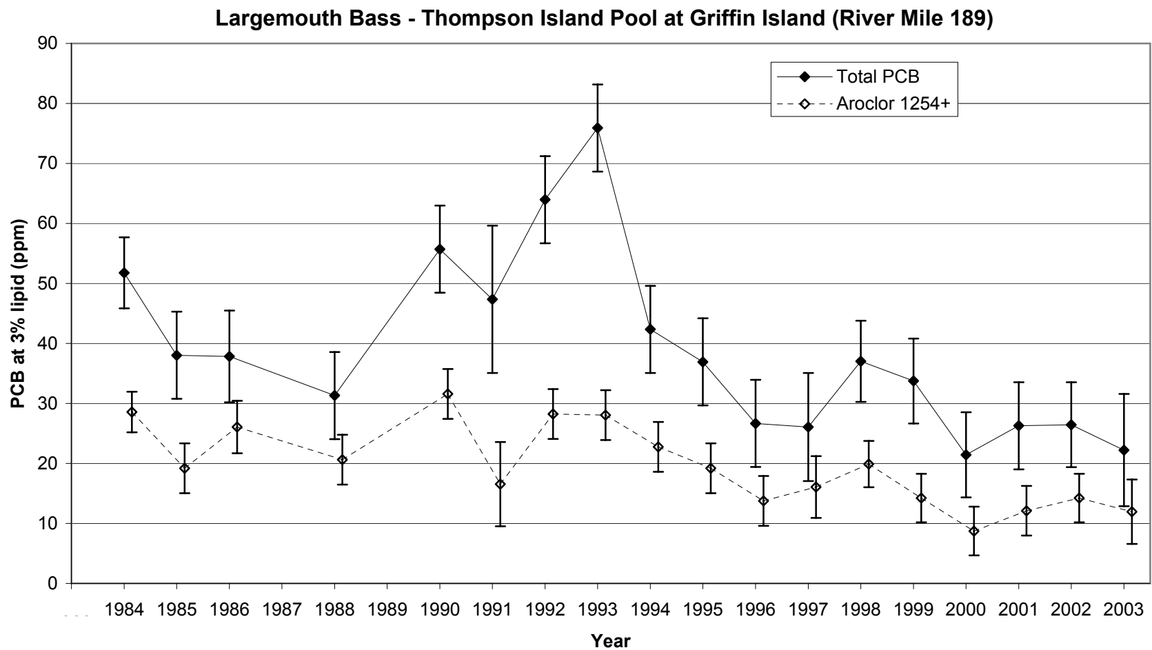
Figure 8. Trend in PCB concentrations at 3% lipid for largemouth bass collected at Griffin Island in the Thompson Island Pool (River mile 189). Results shown are Least Significant Difference mean comparisons (95% confidence intervals) for total PCB - solid lines, and higher chlorinated 'Aroclor 1254+' fraction - dashed lines.
