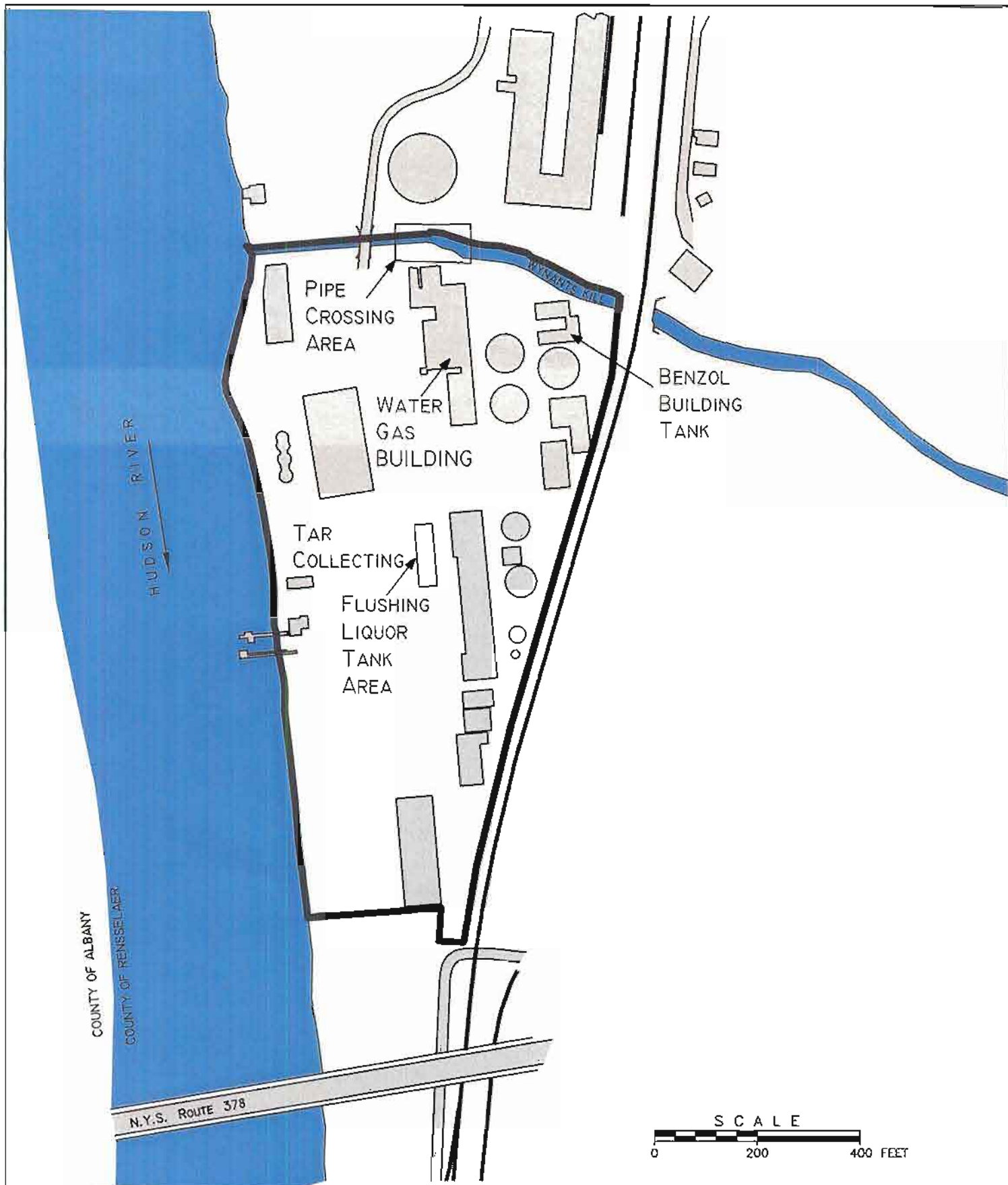
NMPC TROY (WATER ST) AREA 2 SITE TROY, RENSSELAER COUNTY, NEW YORK AREAS TO BE INVESTIGATED (SECTION 8, PARAGRAPH 1)
