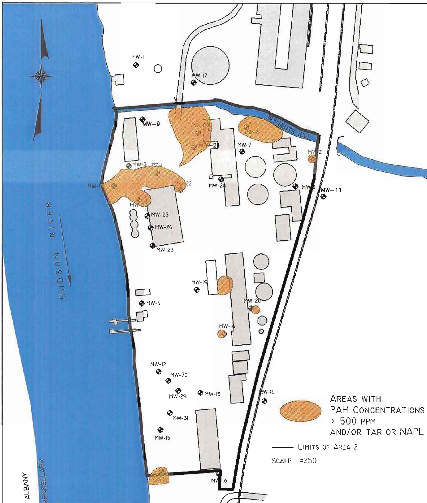
NMPC TROY (WATER ST) AREA 2 SITE TROY, RENSSELAER COUNTY, NEW YORK AREAS WITH SOIL CONC > 500 PPM PAHS, VISUAL TAR, OR NAPL
