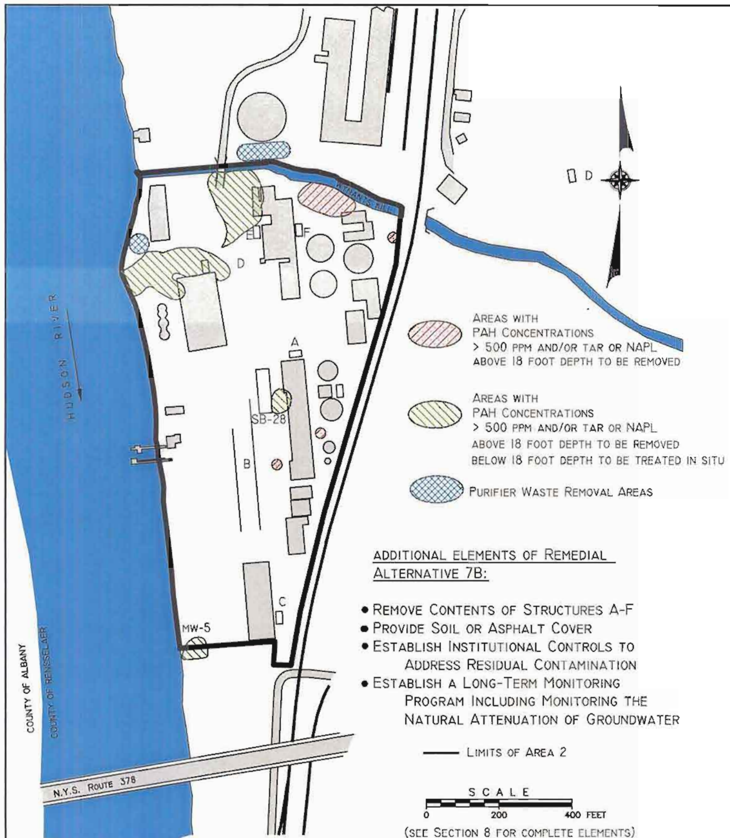
NMPC TROY (WATER ST) AREA 2 SITE TROY, RENSSELAER COUNTY, NEW YORK SELECTED REMEDY COMPONENTS
