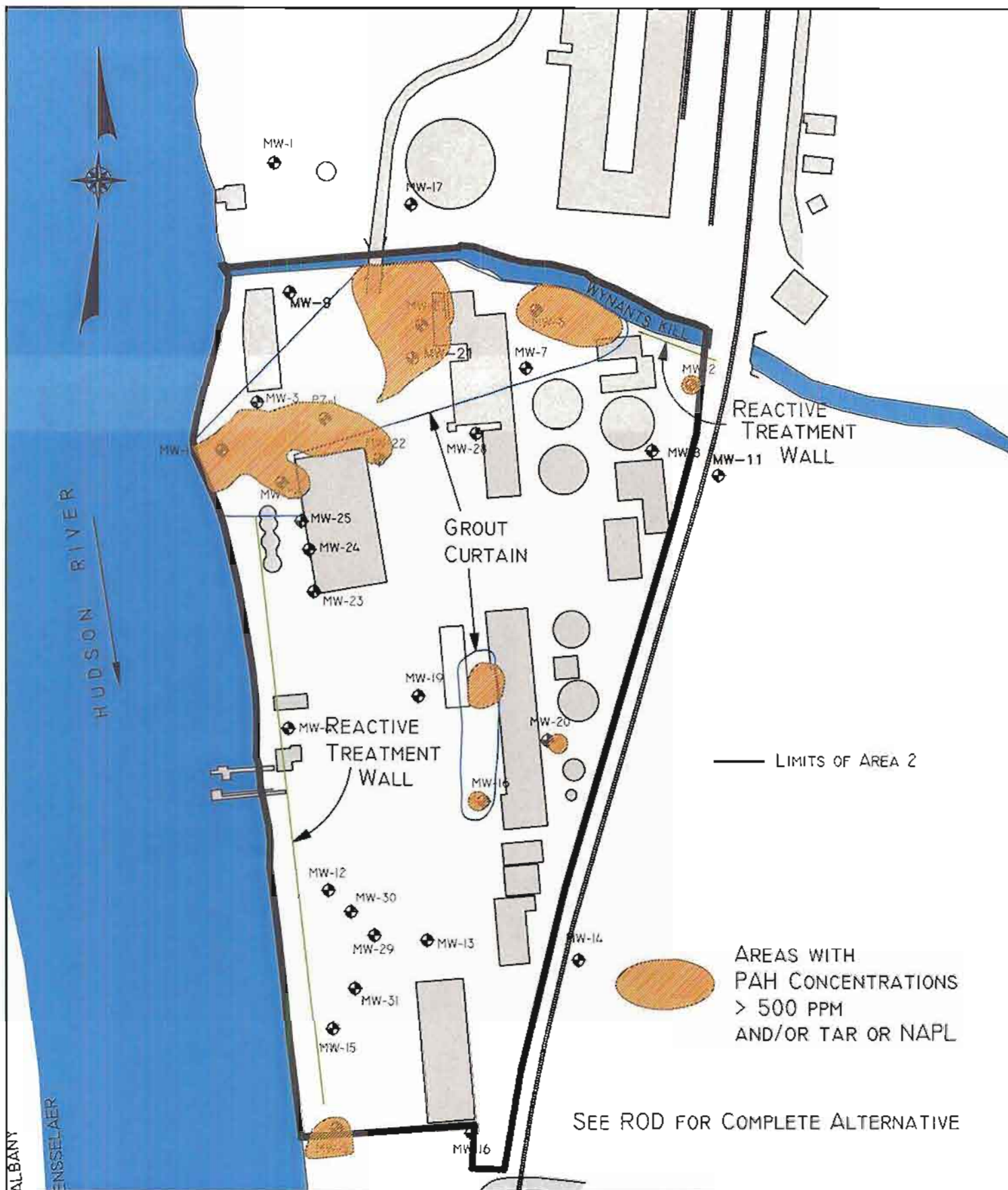
NMPC TROY (WATER ST) AREA 2 SITE TROY, RENSSELAER COUNTY, NEW YORK ALTERNATIVE 2: GROUT CURTAIN, REACTIVE TREATMENT WALL
