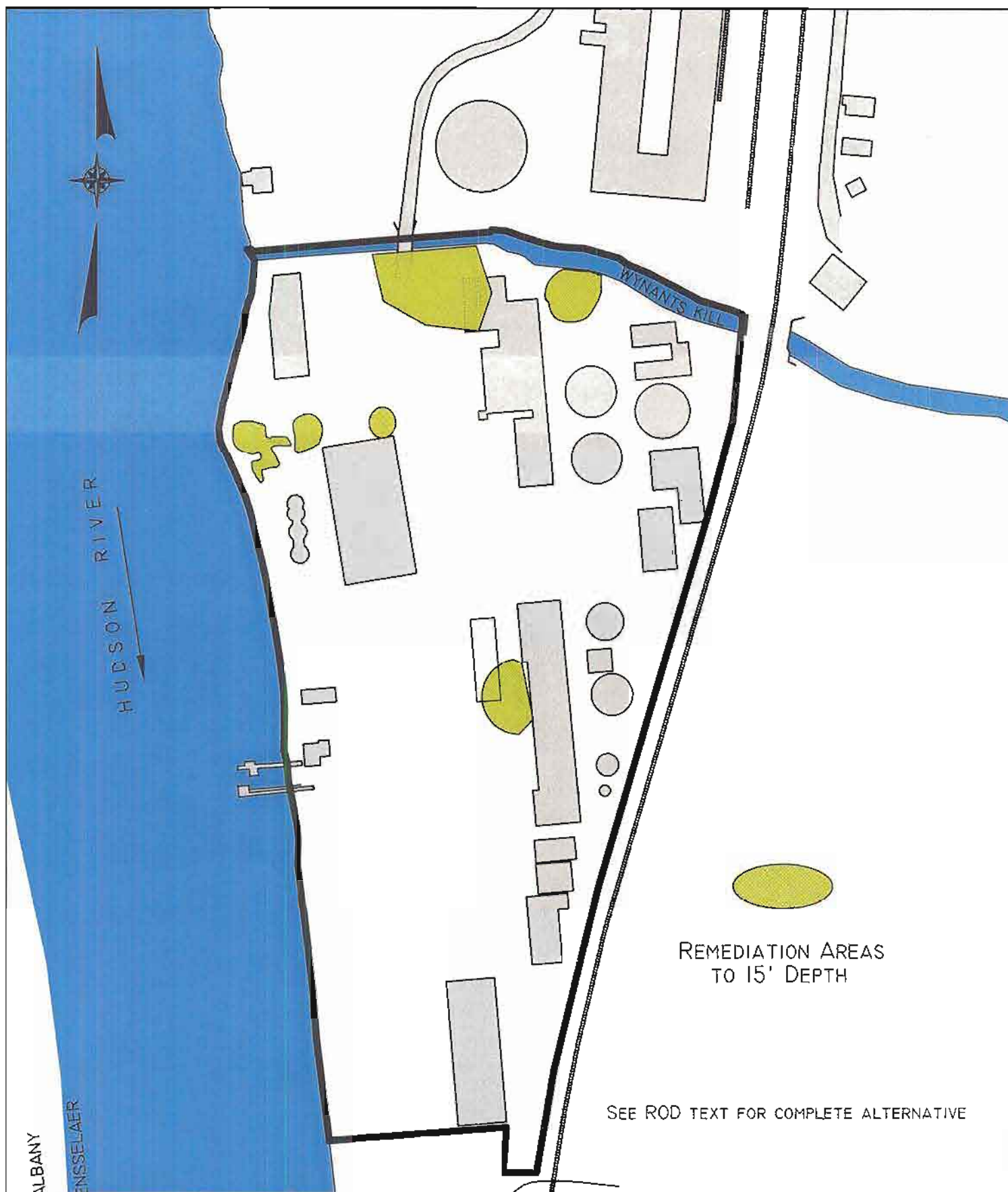
NMPC TROY (WATER ST) AREA 2 SITE TROY, RENSSELAER COUNTY, NEW YORK ALTERNATIVE 3 - REMOVAL AREAS
