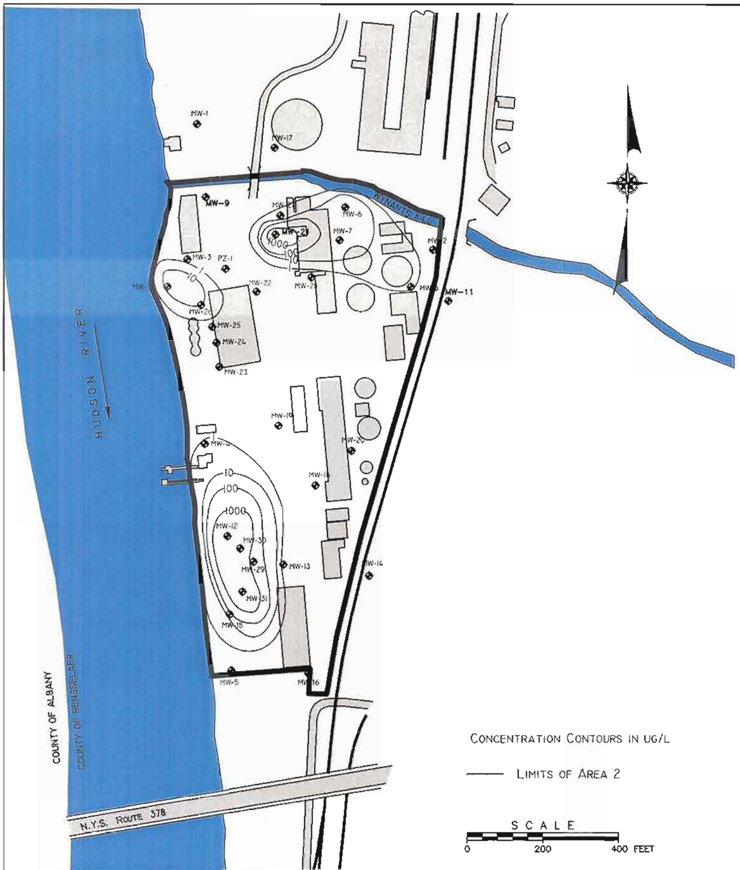
NMPC TROY (WATER ST) AREA 2 SITE TROY, RENSSELAER COUNTY, NEW YORK BTEX IN GROUNDWATER
