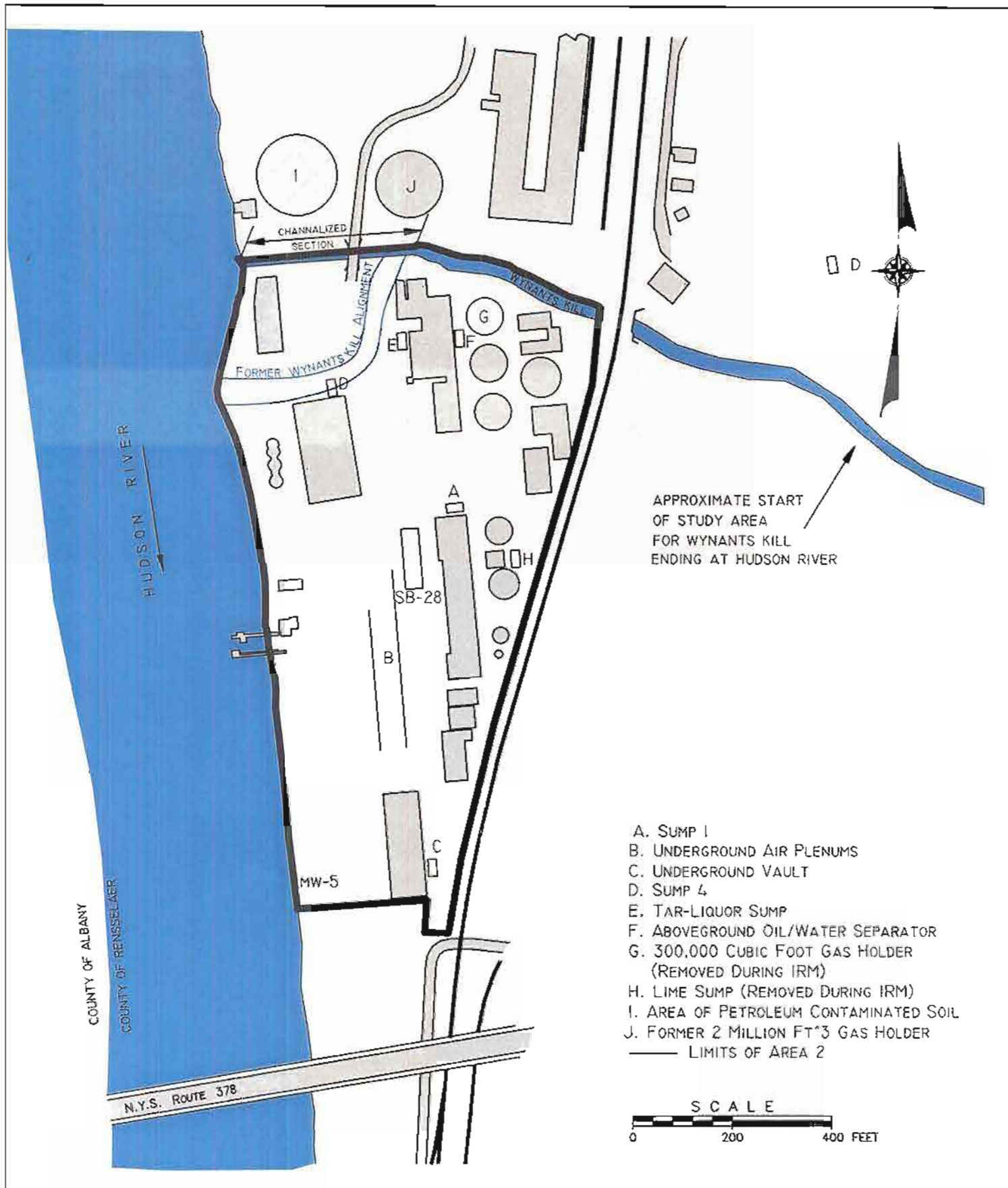
NMPC TROY (WATER ST) AREA 2 SITE TROY, RENSSELAER COUNTY, NEW YORK STRUCTURES OF INTEREST
