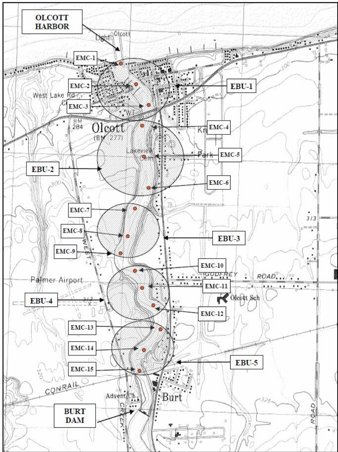
FIGURE 2-2 2004 AOC SEDIMENT SAMPLING SITES AND REACHES
