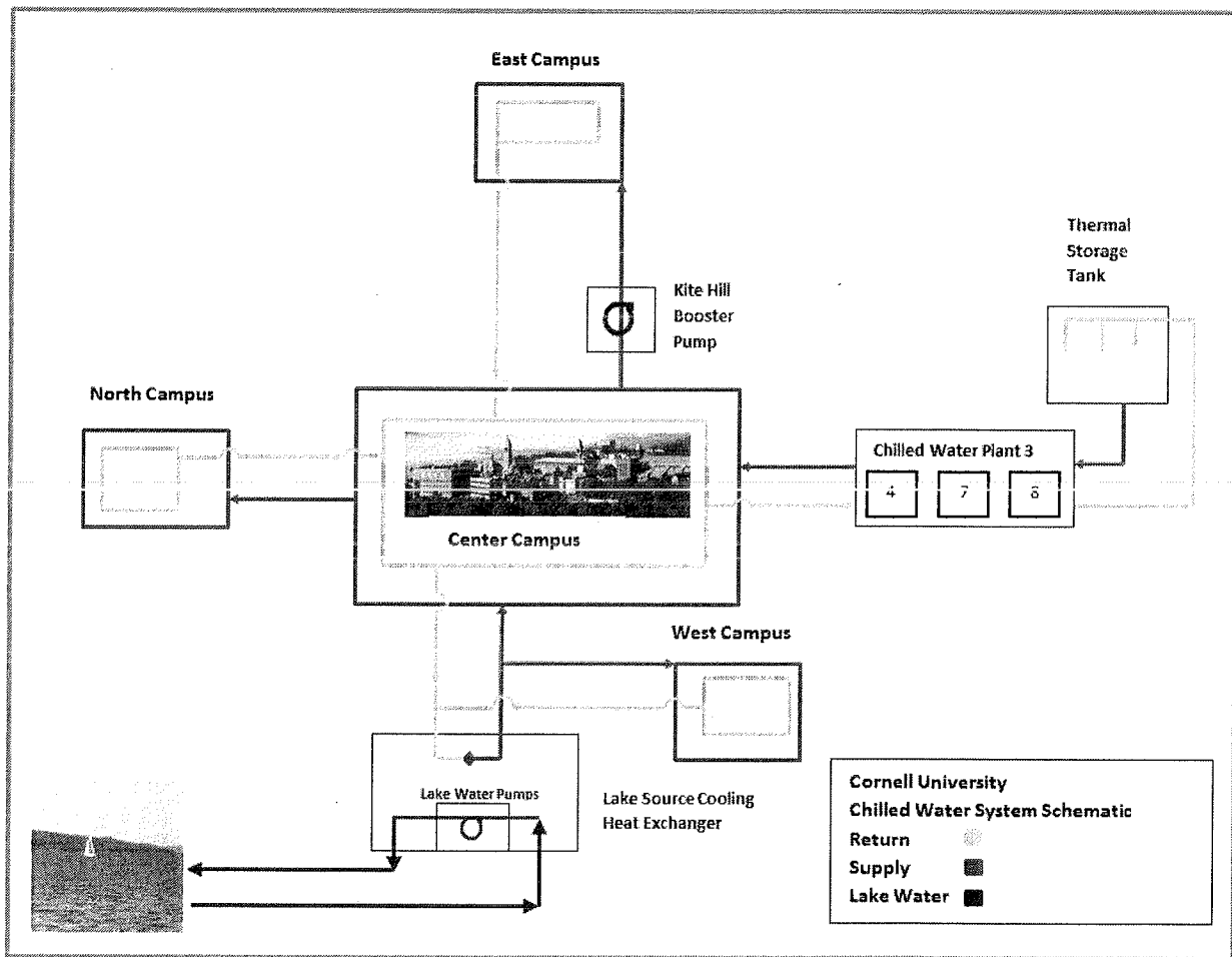
Figure 2.1 Cornell Chilled Water System
