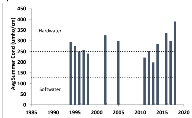
Specific Conductance
