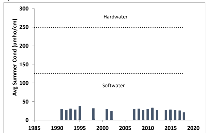
Specific Conductance
