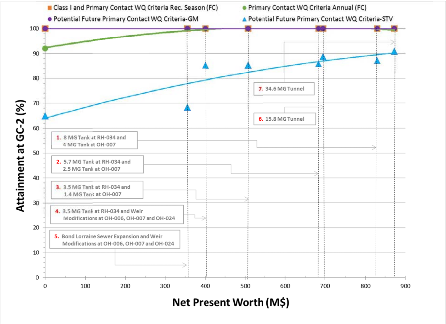
Figure 8-17. Cost vs. Bacteria Attainment at Station GC-2 (2008 Rainfall)
