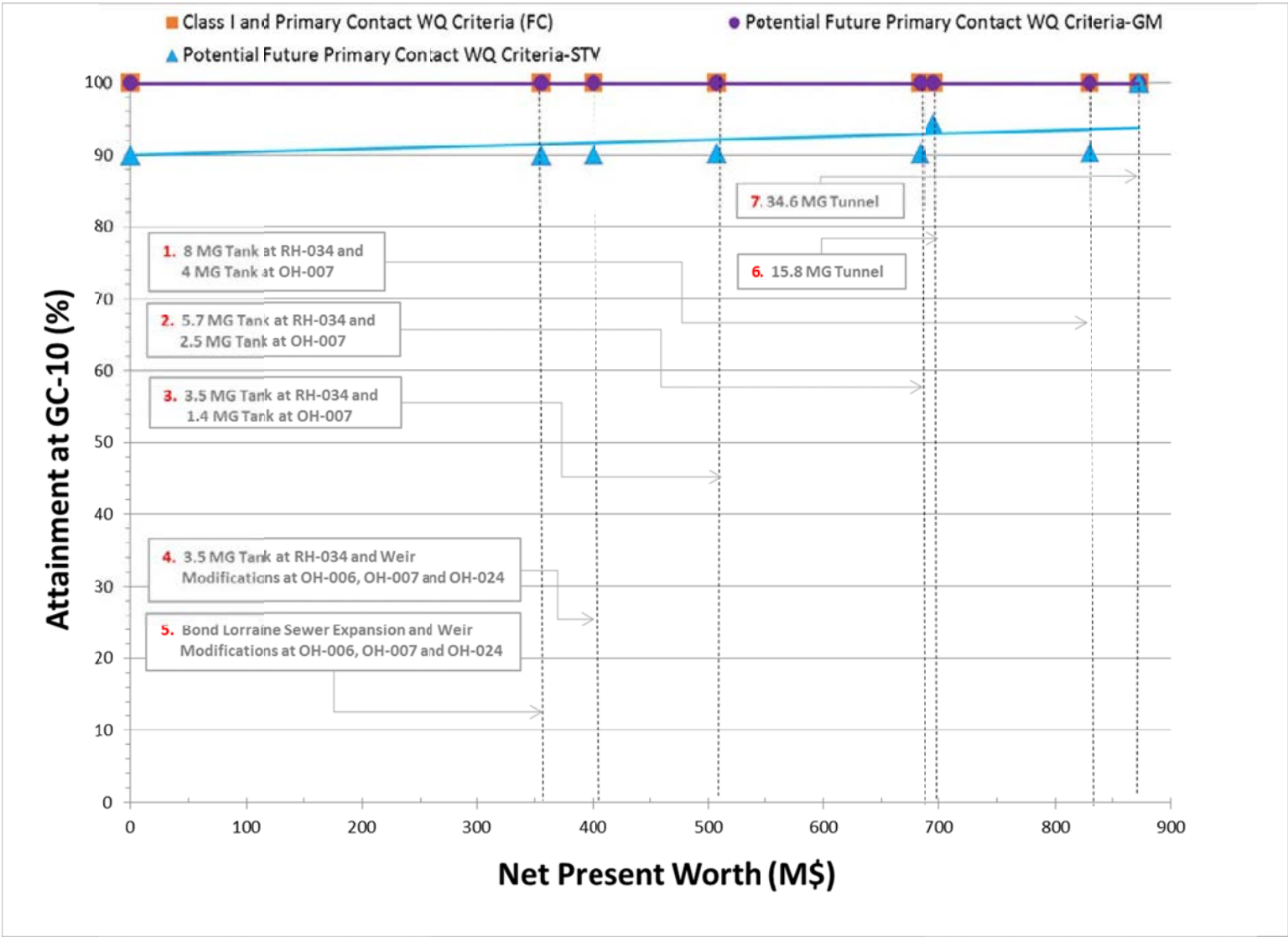
Figure 8-25. Cost vs. Bacteria Attainment at Station GC-10 (2008 Rainfall)
