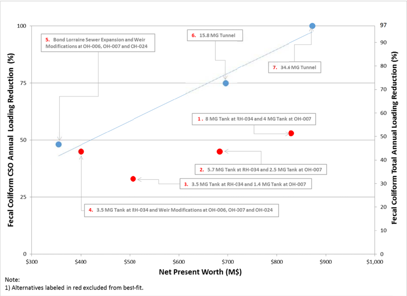
Figure 8-15. Cost vs. Fecal Coliform Loading Reduction (2008 Rainfall)
