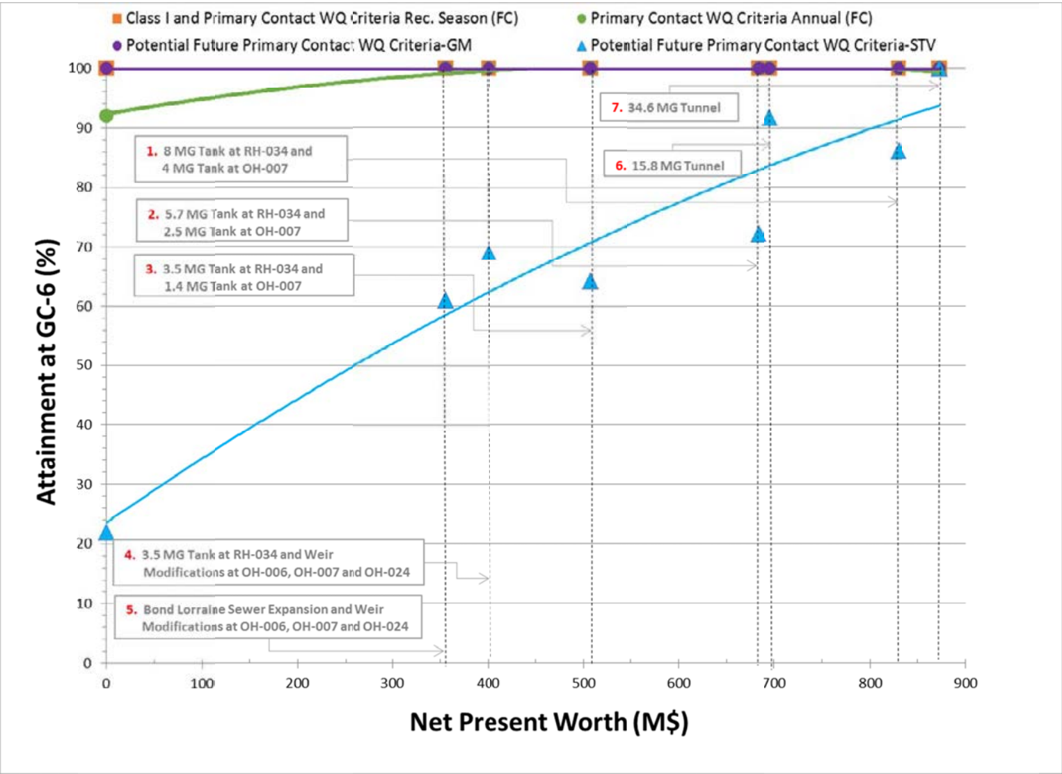
Figure 8-21. Cost vs. Bacteria Attainment at Station GC-6 (2008 Rainfall)
