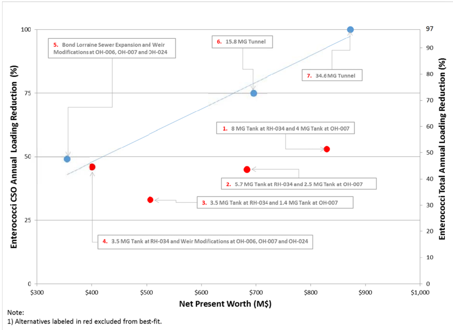
Figure 8-14. Cost vs. Enterococci Loading Reduction (2008 Rainfall)
