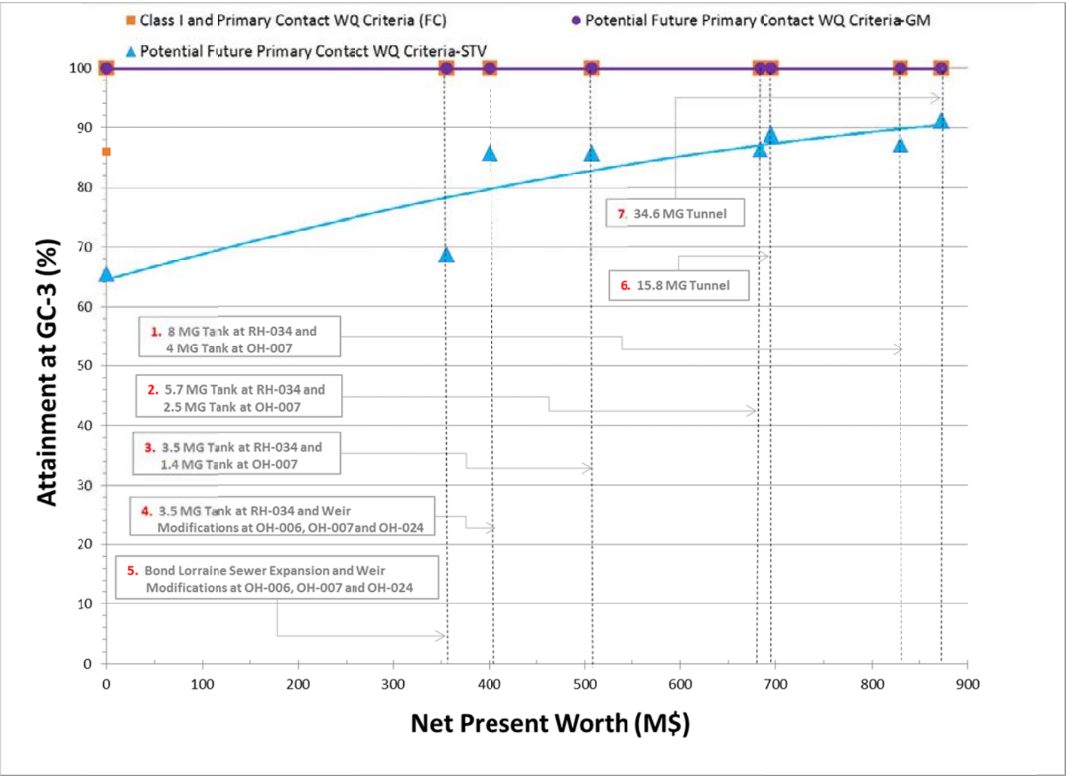
Figure 8-18. Cost vs. Bacteria Attainment at Station GC-3 (2008 Rainfall)
