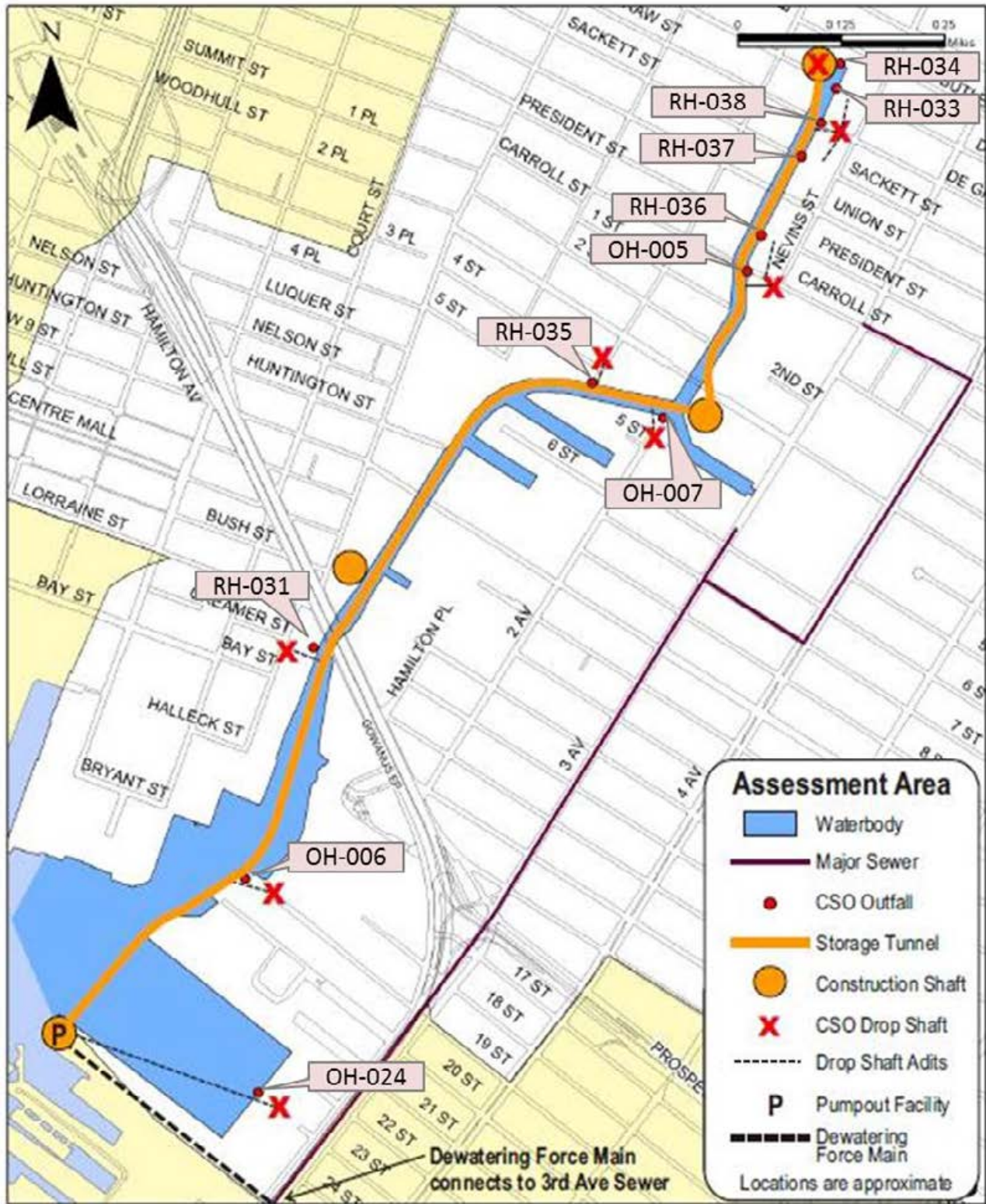
Figure 8-11. Route of Tunnels for 75% and 100% CSO Control
