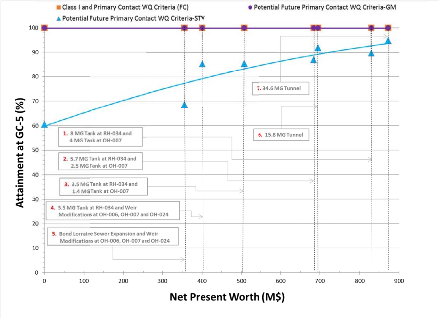
Figure 8-20. Cost vs. Bacteria Attainment at Station GC-5 (2008 Rainfall)
