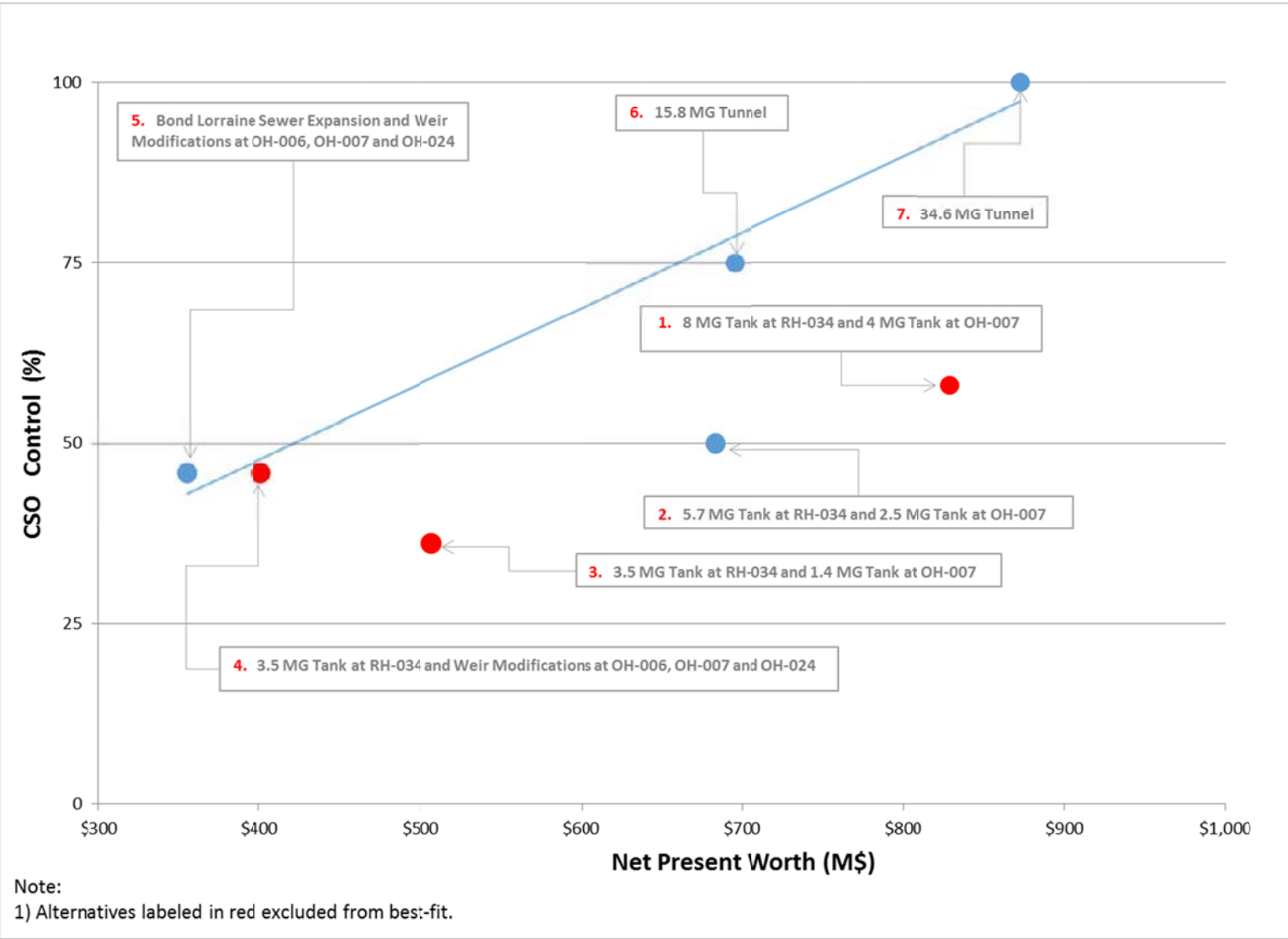
Figure 8-13. Cost vs. CSO Control (2008 Rainfall)
