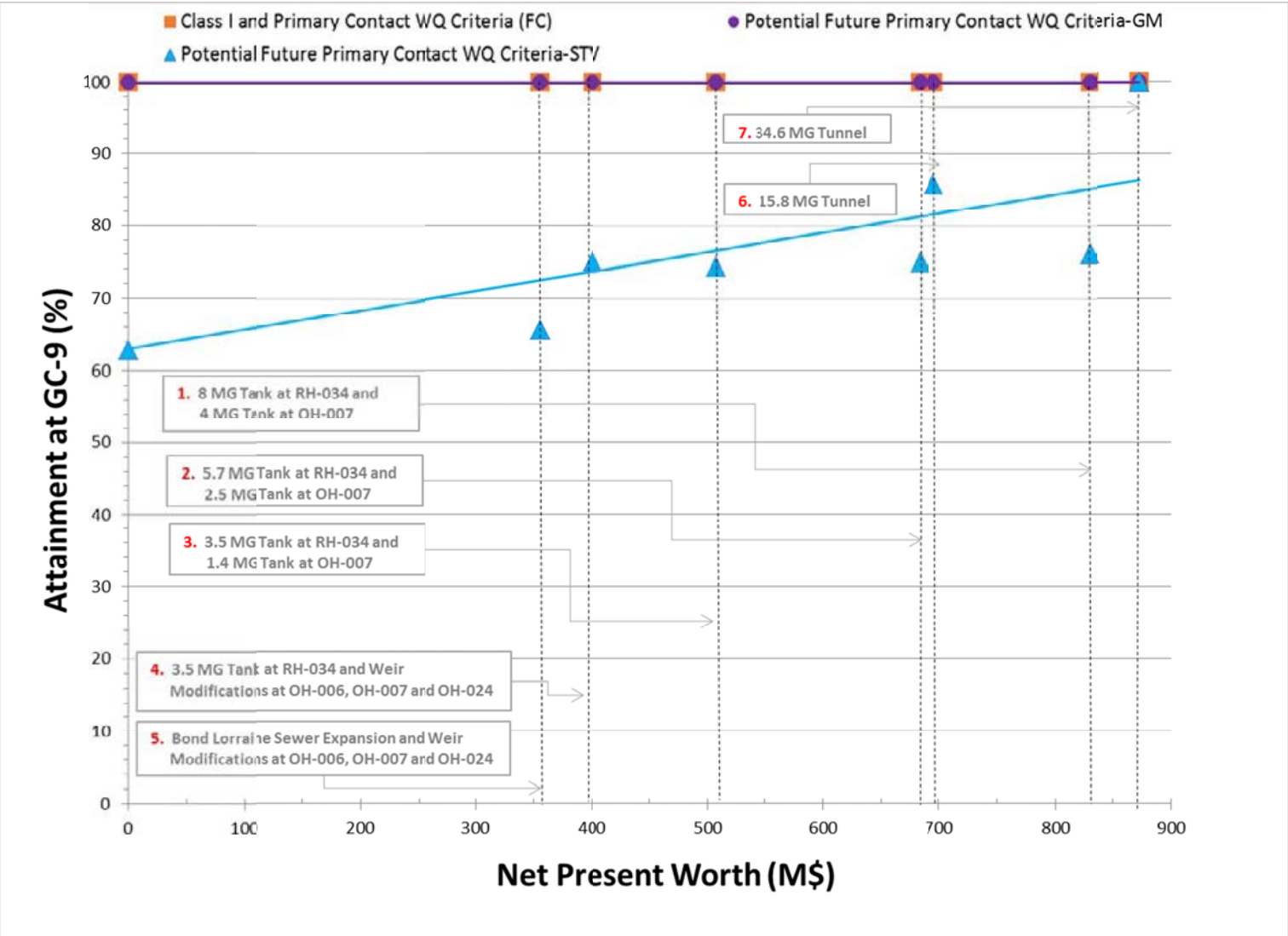
Figure 8-24. Cost vs. Bacteria Attainment at Station GC-9 (2008 Rainfall)
