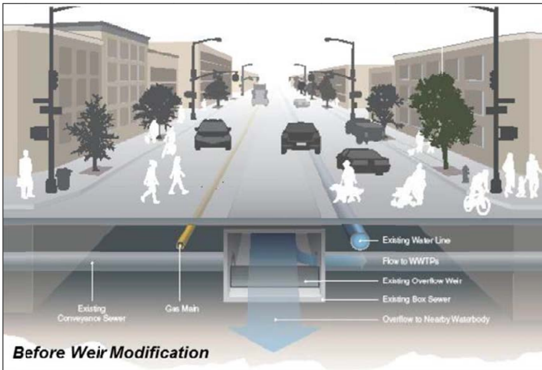
Figure 8-5. Current Weir Schematic at Outfall OH-007
