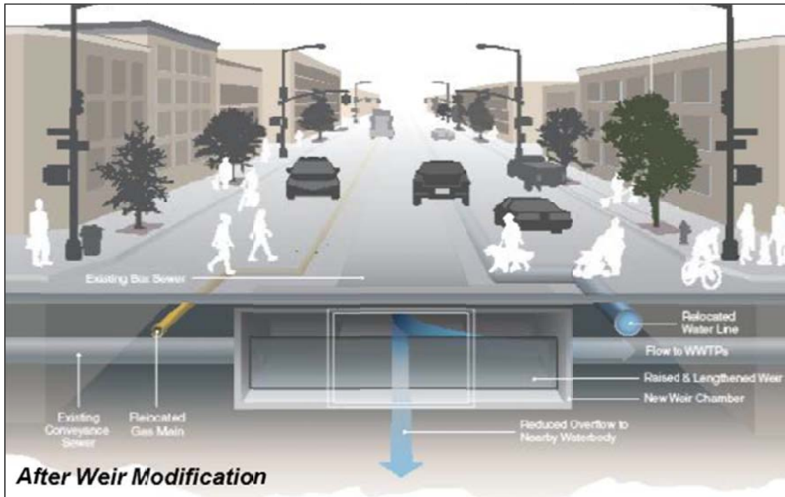
Figure 8-6. Proposed Weir Modification at Outfall OH-007
