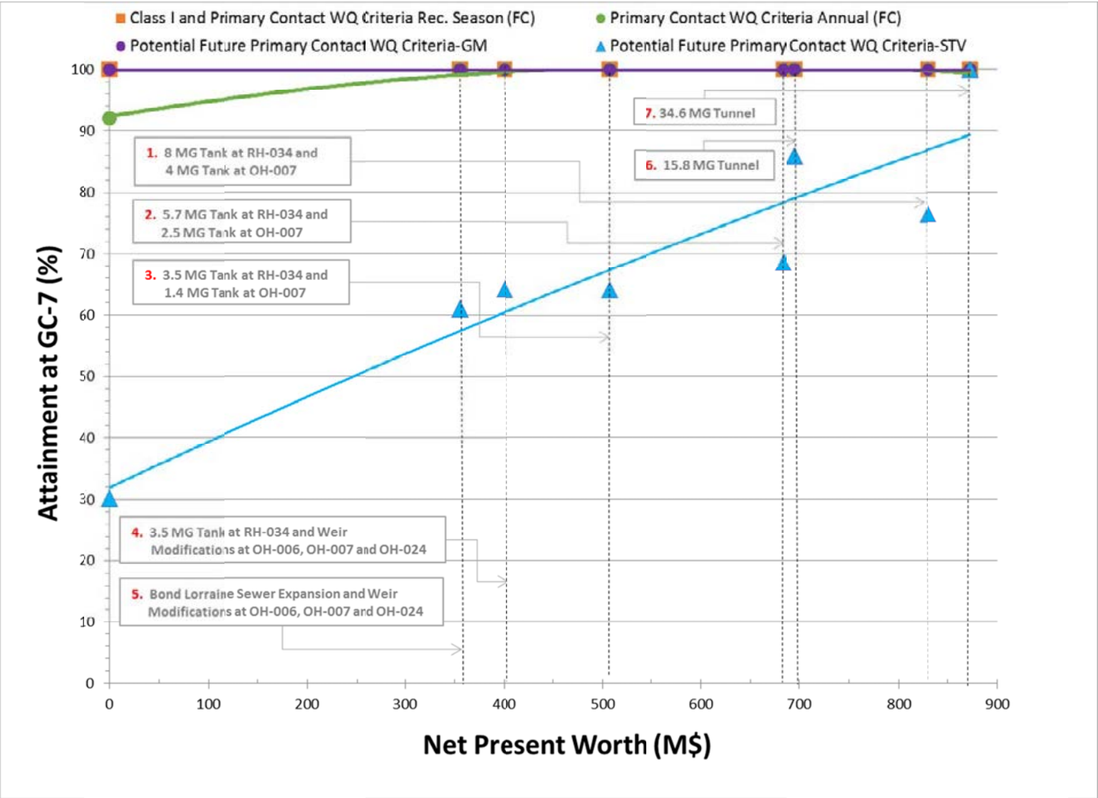
Figure 8-22. Cost vs. Bacteria Attainment at Station GC-7 (2008 Rainfall)
