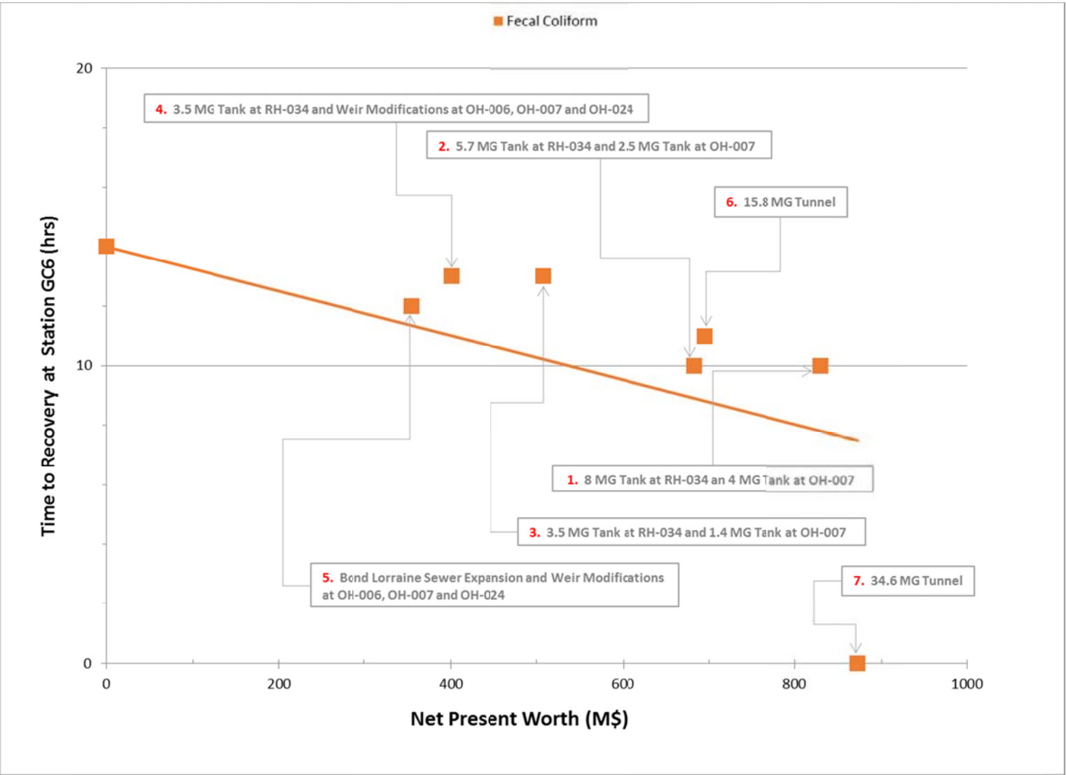
Figure 8-26. Time to Recovery at Station GC-6
