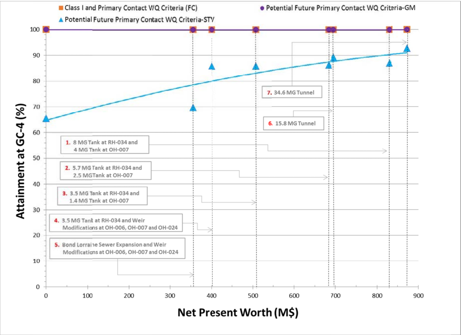
Figure 8-19. Cost vs. Bacteria Attainment at Station GC-4 (2008 Rainfall)
