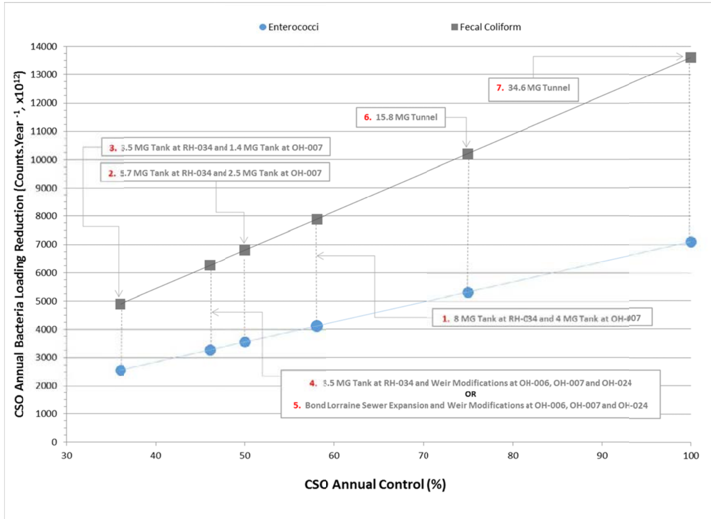
Figure 8-12. CSO Annual Control vs. Annual CSO Bacteria Loading Reduction (2008 Rainfall)
