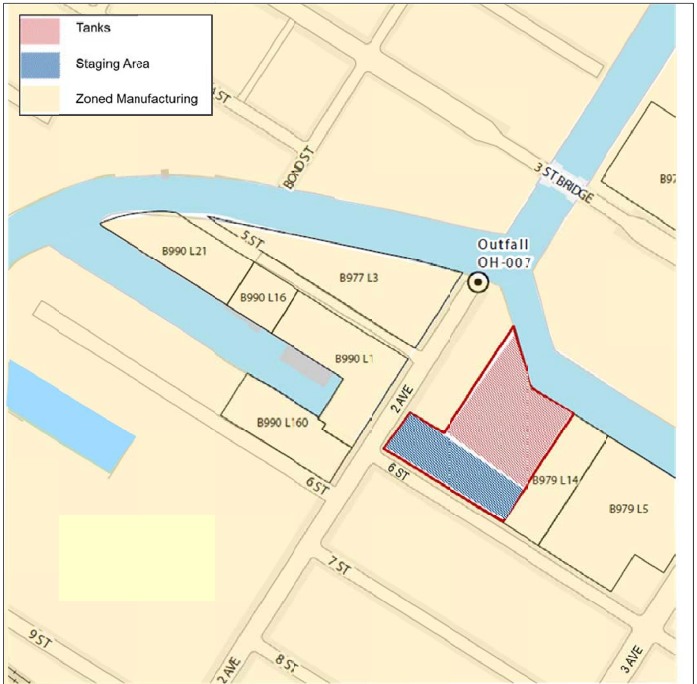
Figure 8-10. Outfall OH-007 Site OH-5
