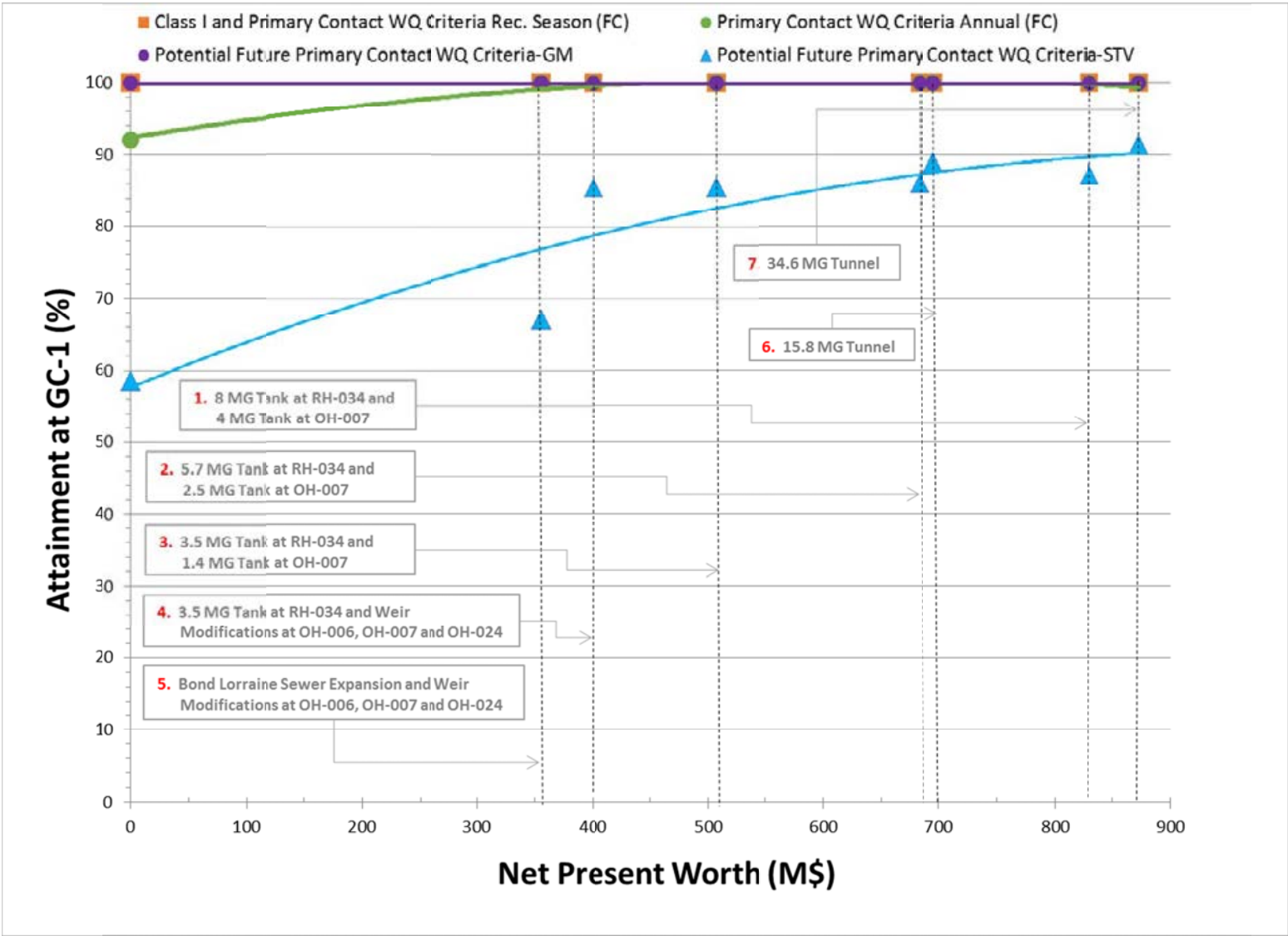
Figure 8-16. Cost vs. Bacteria Attainment at Station GC-1 (2008 Rainfall)
