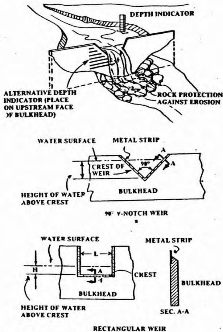
Figure 6.7 - Standard Weirs
