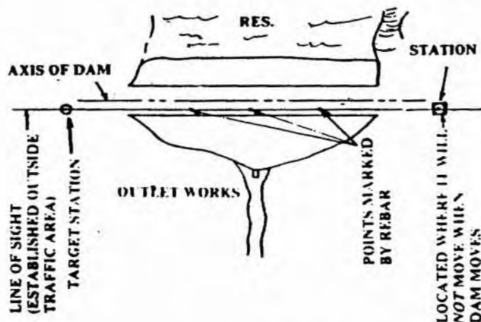
Figure 6.1b - Plan of Alignment System
