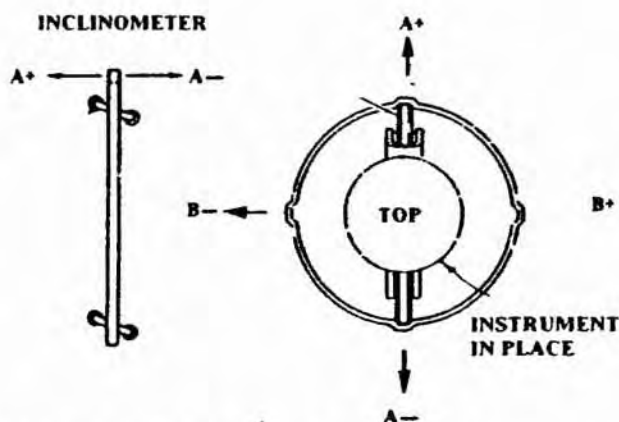
Figure 6.3c Inclinator and Casing
