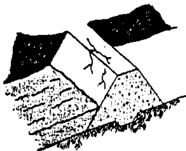
Figures 5.5 Inspection Guidelines - Spillways
