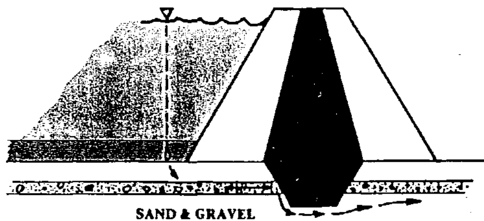
Figure 2.5 Culoff Trench and Upstream Blanket
