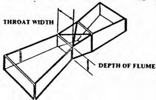
Figure 6.8 Parshall Flume
