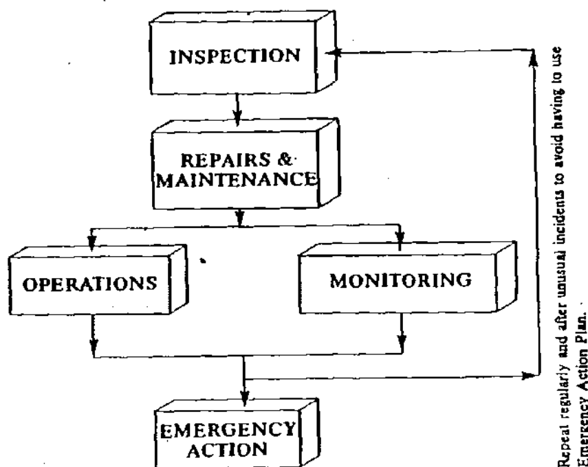
Figure 4.1 Procedural Guidelines for A Dam Safety Program
