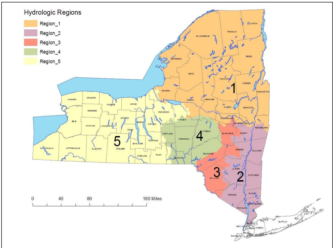
Figure 1: Hydrologic Regions of New York Adapted from Magnitude and Frequency of Floods in New York (USGS 2006) 1
