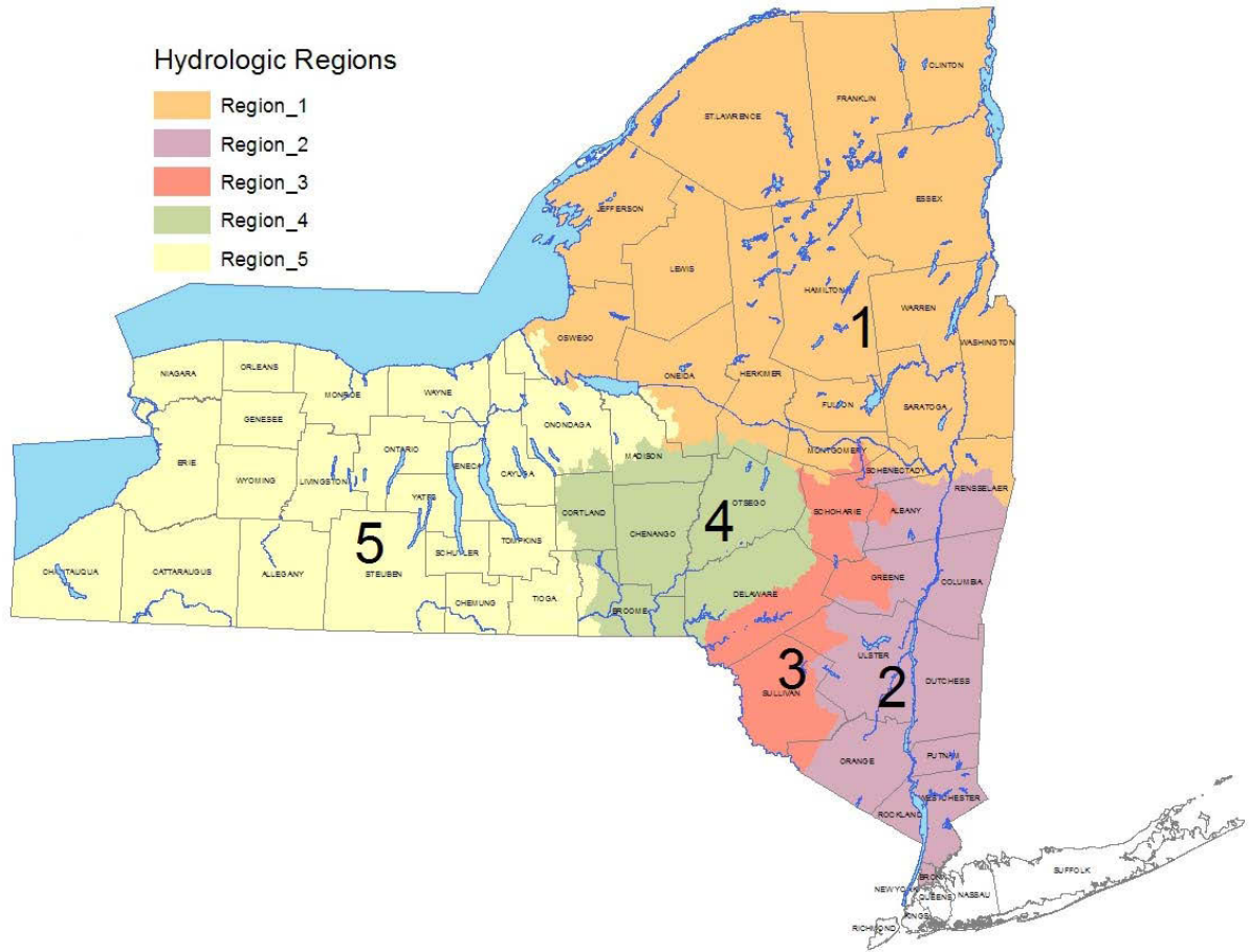
Figure 1. Hydrologic Regions of New York. as adopted from “Magnitude and Frequency of Floods in New York” (USGS 2006).
