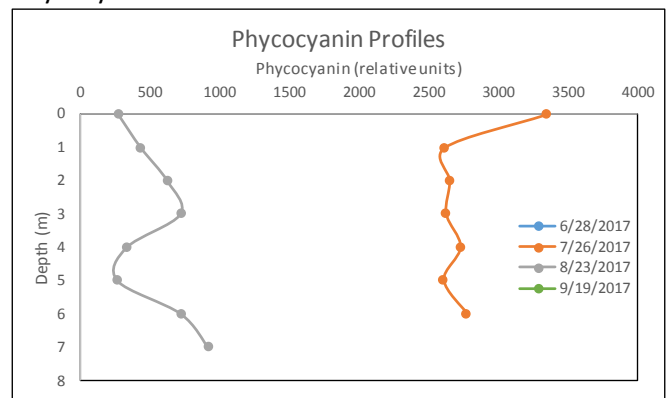
Phycocyanin
