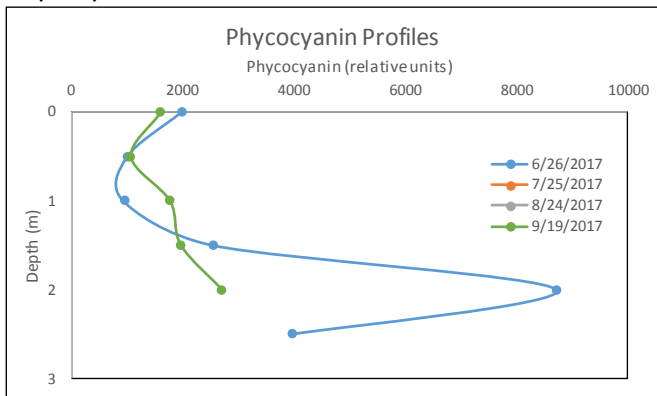
Phycocyanin
