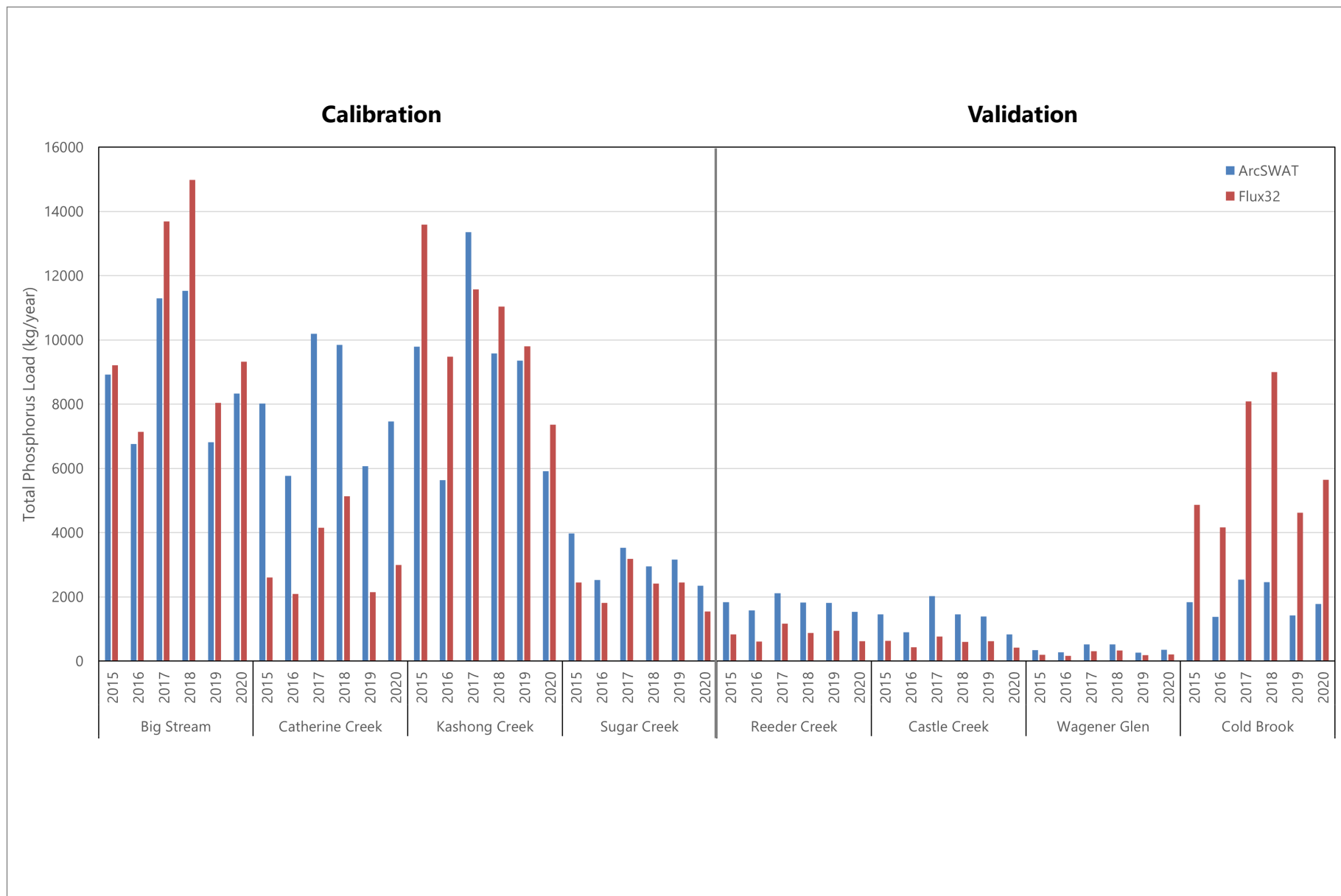
Figure A3-16 Annual Total Phosphorus Load at Validation Locations Seneca-Keuka Watershed Model Report Seneca-Keuka Watershed Nine Element Plan
