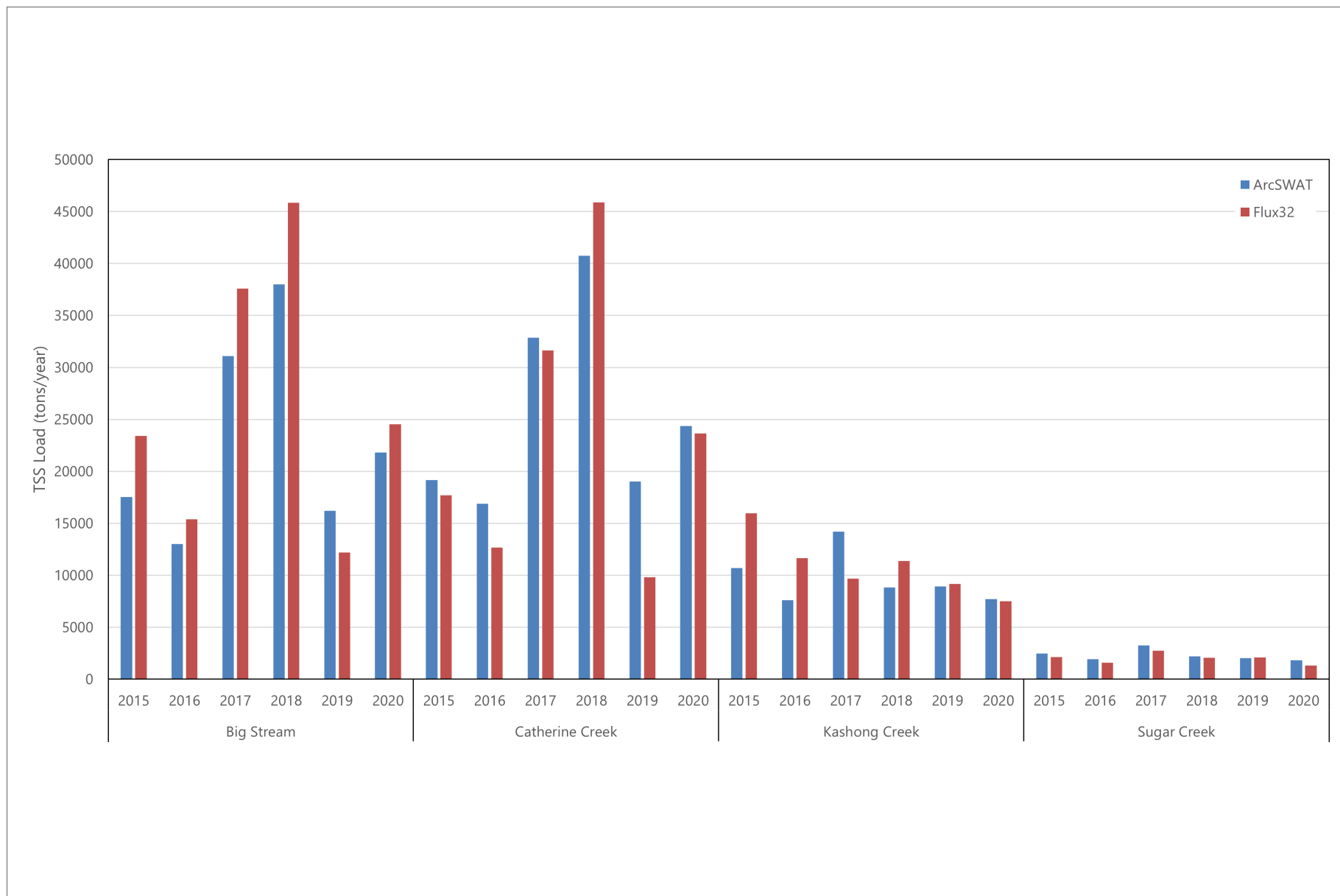
Figure A3-12 Annual Total Suspended Solids Load at Calibration Locations
