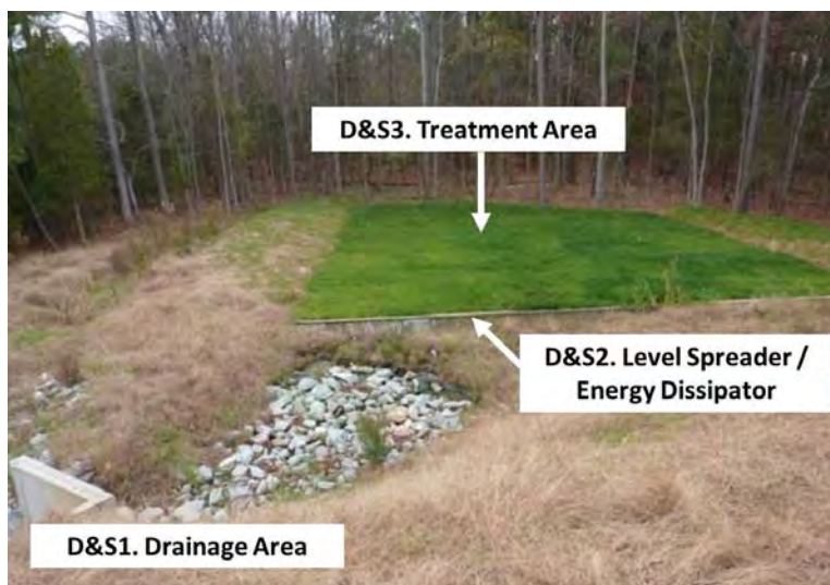
Figure 2.4.1 Key Areas for Level 1 Inspection of Disconnection and Sheetflow with filter strip shown.
