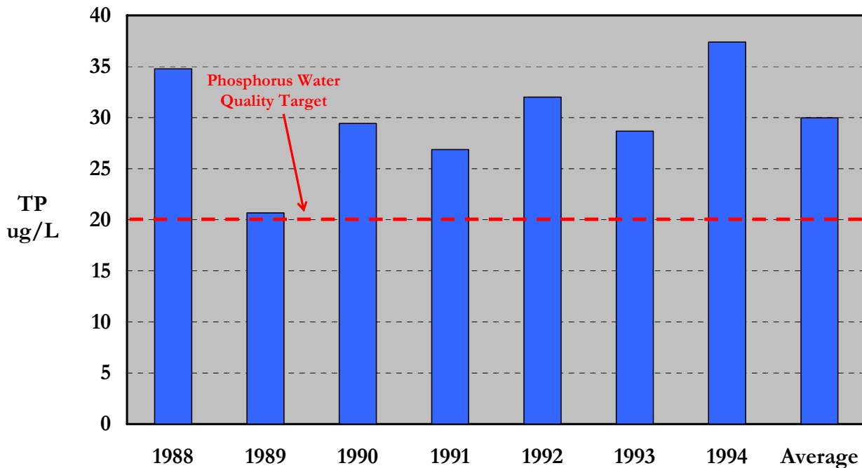
Figure 6. Summer Mean Epilimnetic Total Phosphorus Levels in Little Sodus Bay
