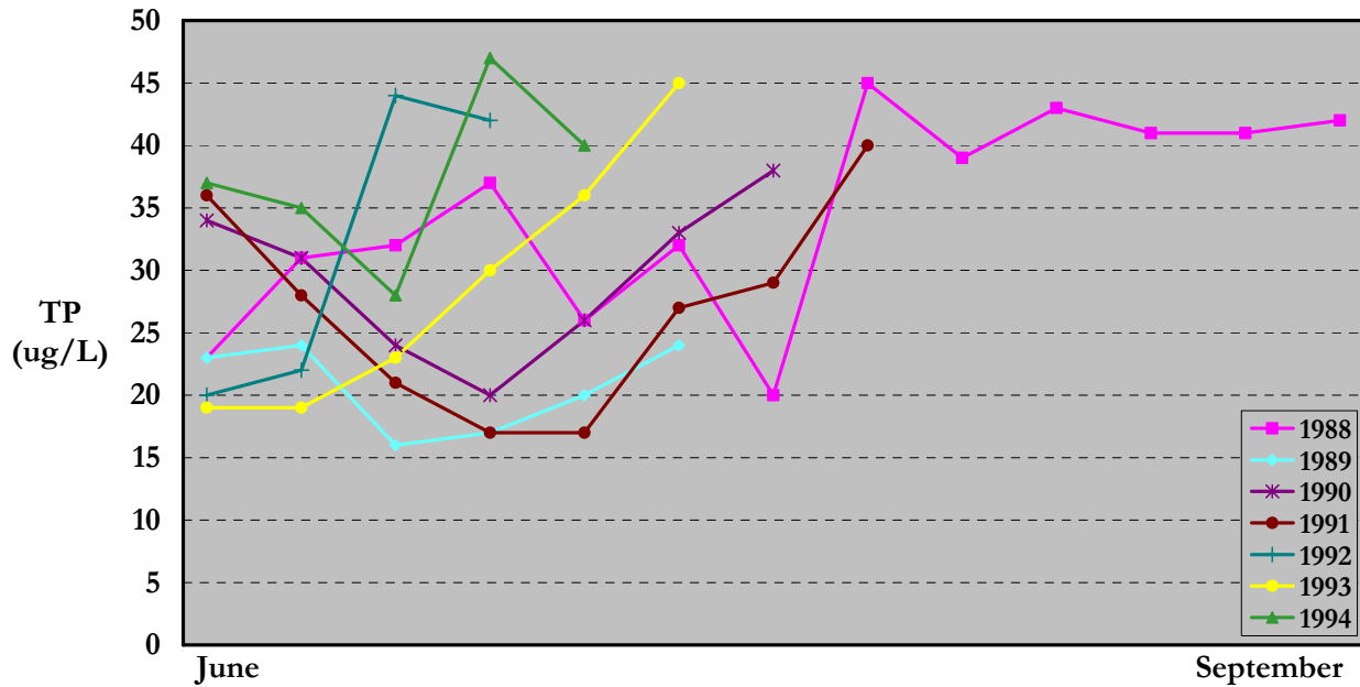
Figure 5. Epilimnetic Phosphorus Concentrations For Little Sodus Bay
