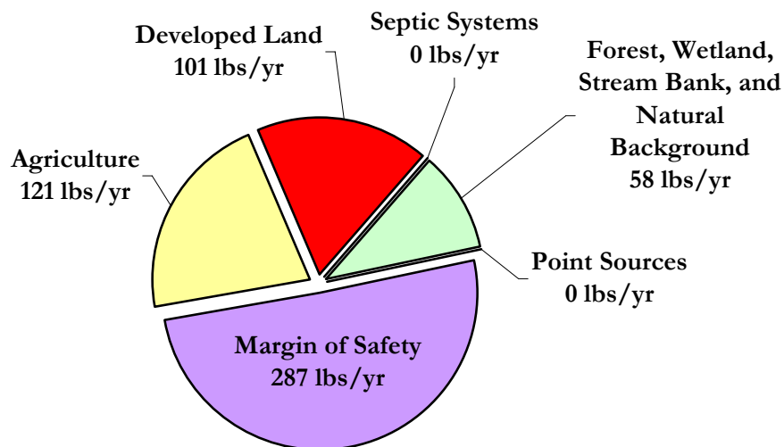
Figure 9. Total Phosphorus Load Allocations for Little Sodus Bay (lbs/yr)
