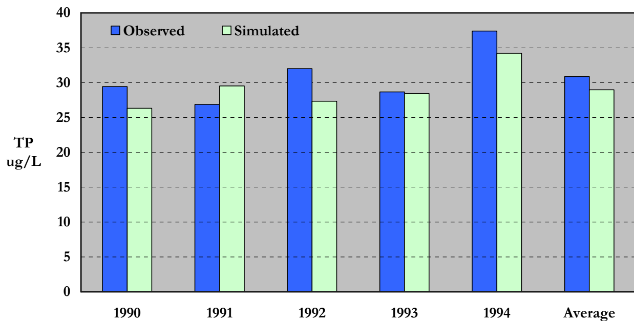
Figure 8. Observed vs. Simulated Summer Mean Epilimnetic Total Phosphorus Concentrations ( \mu\text{g/L} ) in Little Sodus Bay
