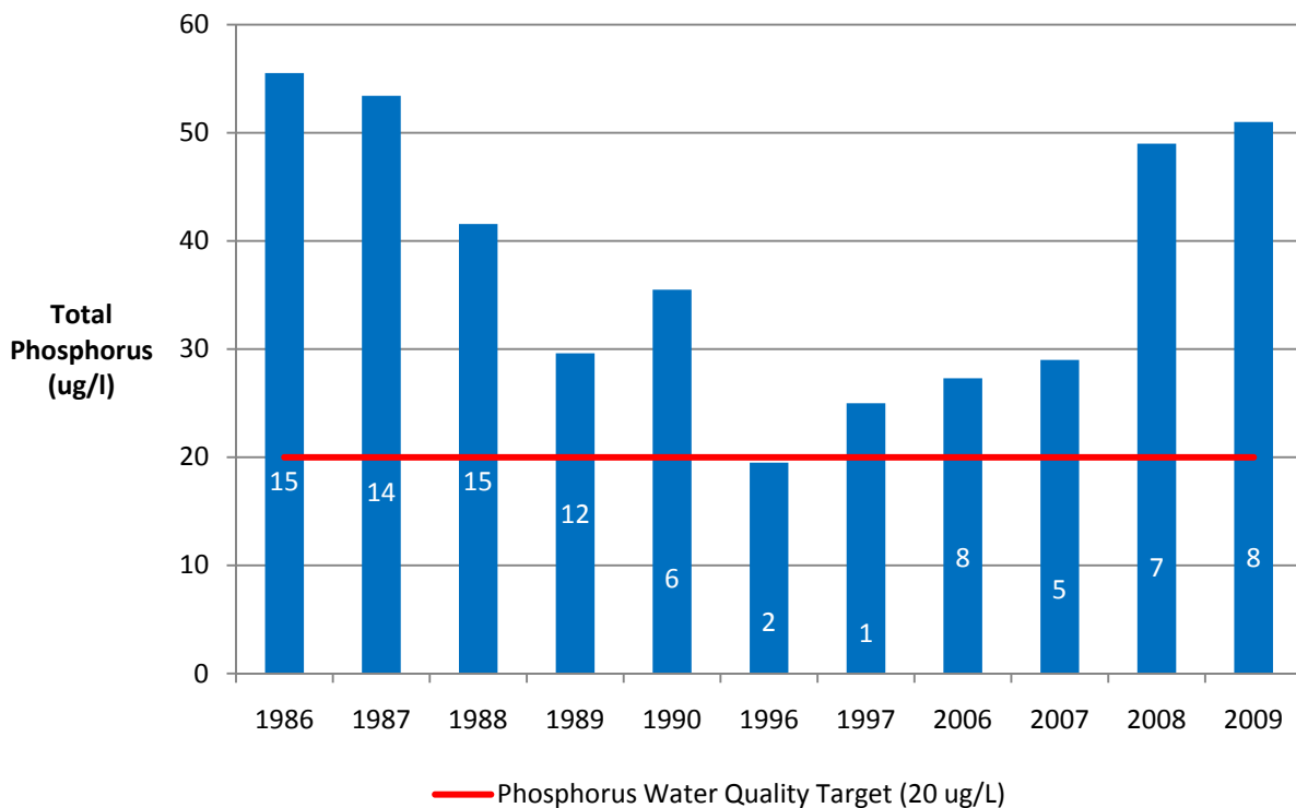
Figure 6. Summer Mean Epilimnetic Total Phosphorus Levels in Silver Lake
