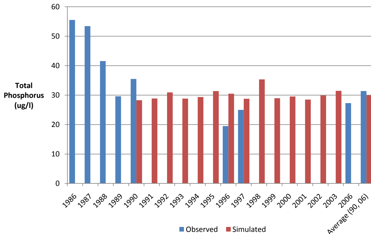
Figure 8. Observed vs. Simulated Summer Mean Epilimnetic Total Phosphorus Concentrations ( \mu\text{g/L} ) in Silver Lake
