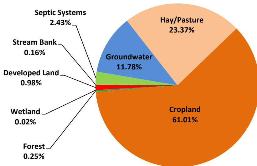
Figure 7. Estimated Sources of Total Phosphorus Loading to Silver Lake
