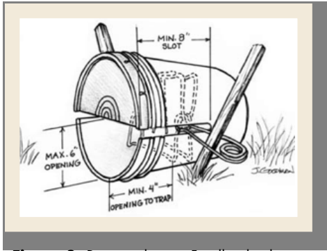
Figure 8. Restricted entry 5-gallon bucket set
