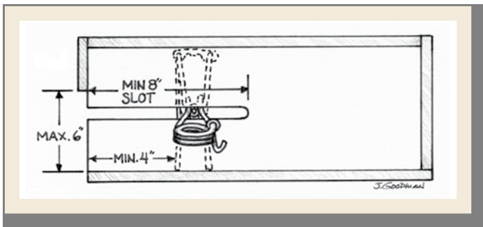
Figure 11. Box cubby with "mid-slot" trap
