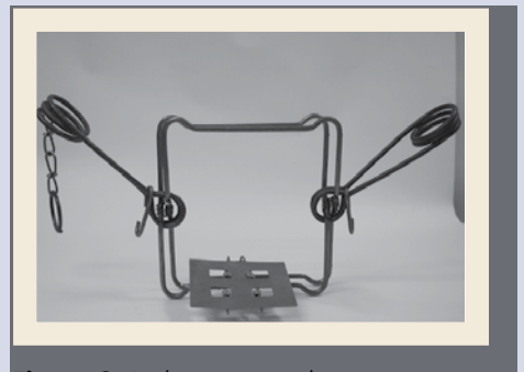
Figure 2. Bodygrip trap with pan-trigger
