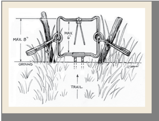
Figure 16. Typical trail set without enclosure
