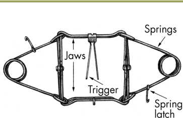
Figure OT10. Bodygrip trap
