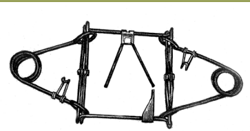
Figure OT11a. Bodygrip trap with "V" configured trigger
