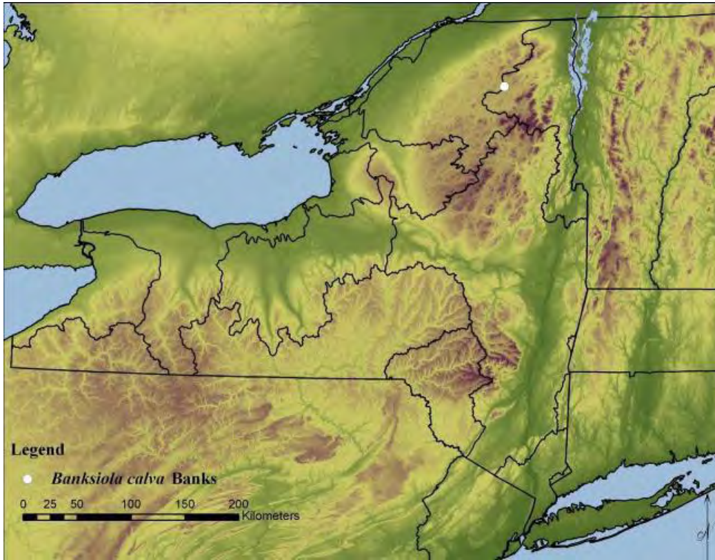
Figure 2. Distribution of Banksiola calva in New York State (Myers et al. 2010).
