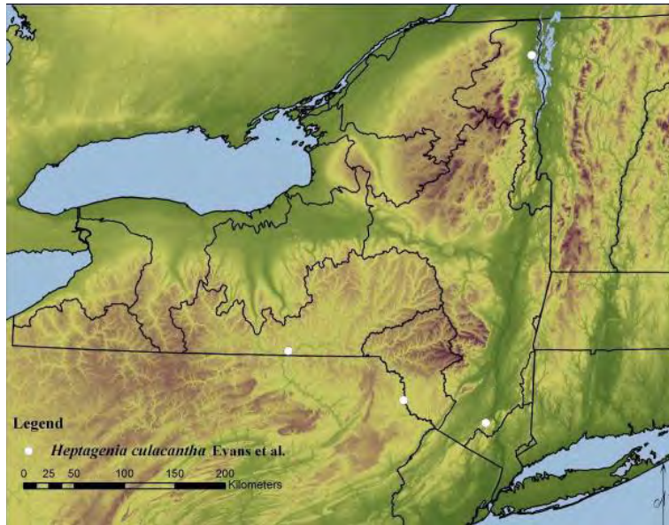
Figure 2. Records of Heptagenia culacantha (Evans et al. 1985) in New York (Myers et al. 2010)
