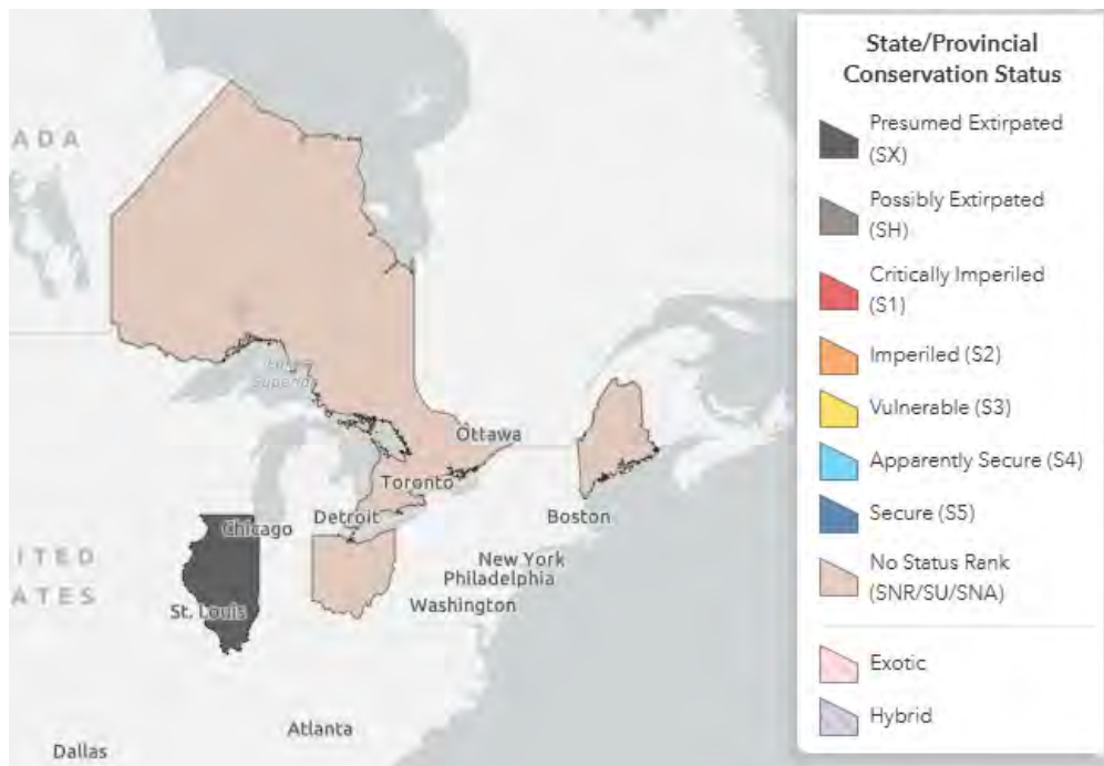
Figure 1. Conservation Status of Neoperla mainensis in North America (NatureServe 2024).
