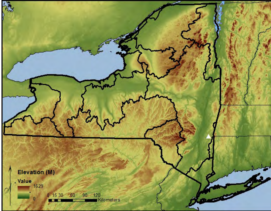
Figure 2. Distribution of Neoperla mainensis in New York.
