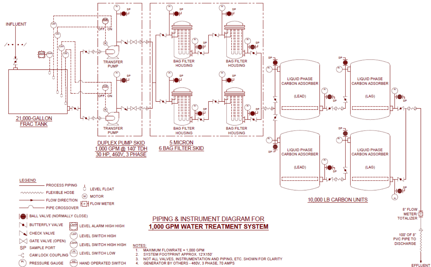
Water Treatment System Schematic
