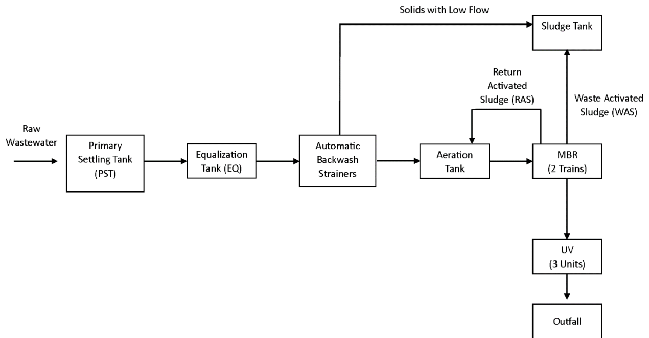
Overlook Farms WWTP - Flow Diagram Design Average Daily Flow: 41,800 gallons
